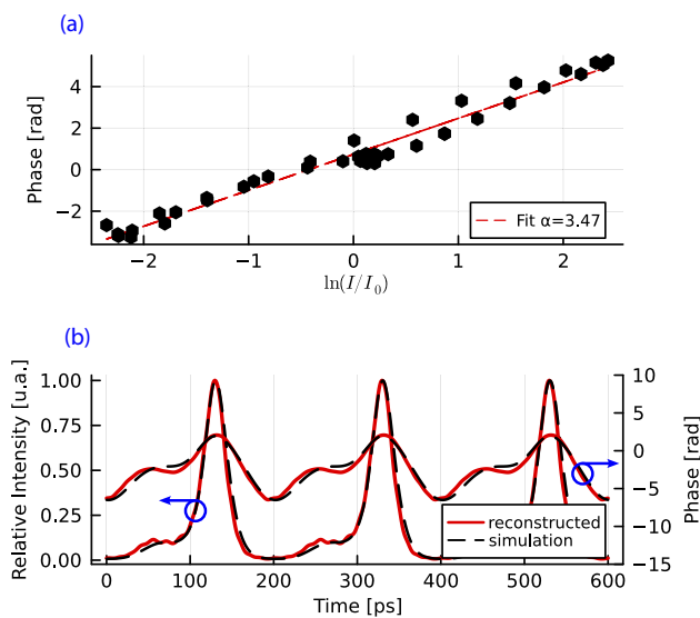
Fig. 6. (a) Plot of \phi(t) as a function of \ln(I(t)) , for i_0 = 26 mA ( r = 2 ). (b) Reconstructed (full lines) versus simulated (dashed lines) I(t) and \phi(t) . The simulation uses Eqs. (6)–(8), with \alpha = 3.47 , r = 2 , m = 1.5 , \epsilon = 0.028 .
