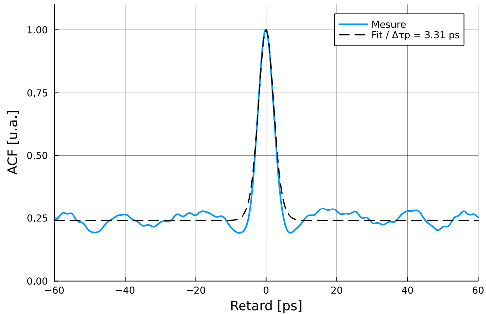
FIGURE 4.25 – Autocorrélation.
