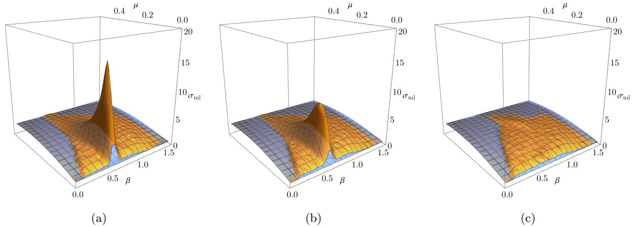
FIGURE C.3. Mitigation limit \sigma_{ml} as a function of \beta and \mu in the case of an NES (blue surface) and a BNES (orange surface) for \lambda given by (C.7a), \alpha = 2 and \epsilon given by Eq. (C.7c). The initial conditions are (x_0, y_0) = p_0^{st} + (per, per) for the NES and (x_0, y_0) = p_1^{st} + (per, per) for the BNES, respectively. The perturbation parameter is 0.001, 0.01 and 0.1 in (a) to (c), respectively.
