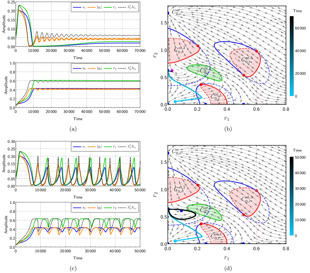
FIGURE B.10. Bifurcation of a fixed point to a limit cycle of the slow subsystem. Same caption as in Fig. B.4 with the initial condition \mathbf{r}_{0,7} = (0.05, 0.05) . The parameters (B.59) are used, with (a) and (b) \gamma = 0.09053 and (c) and (d) \gamma = 0.09075 .
