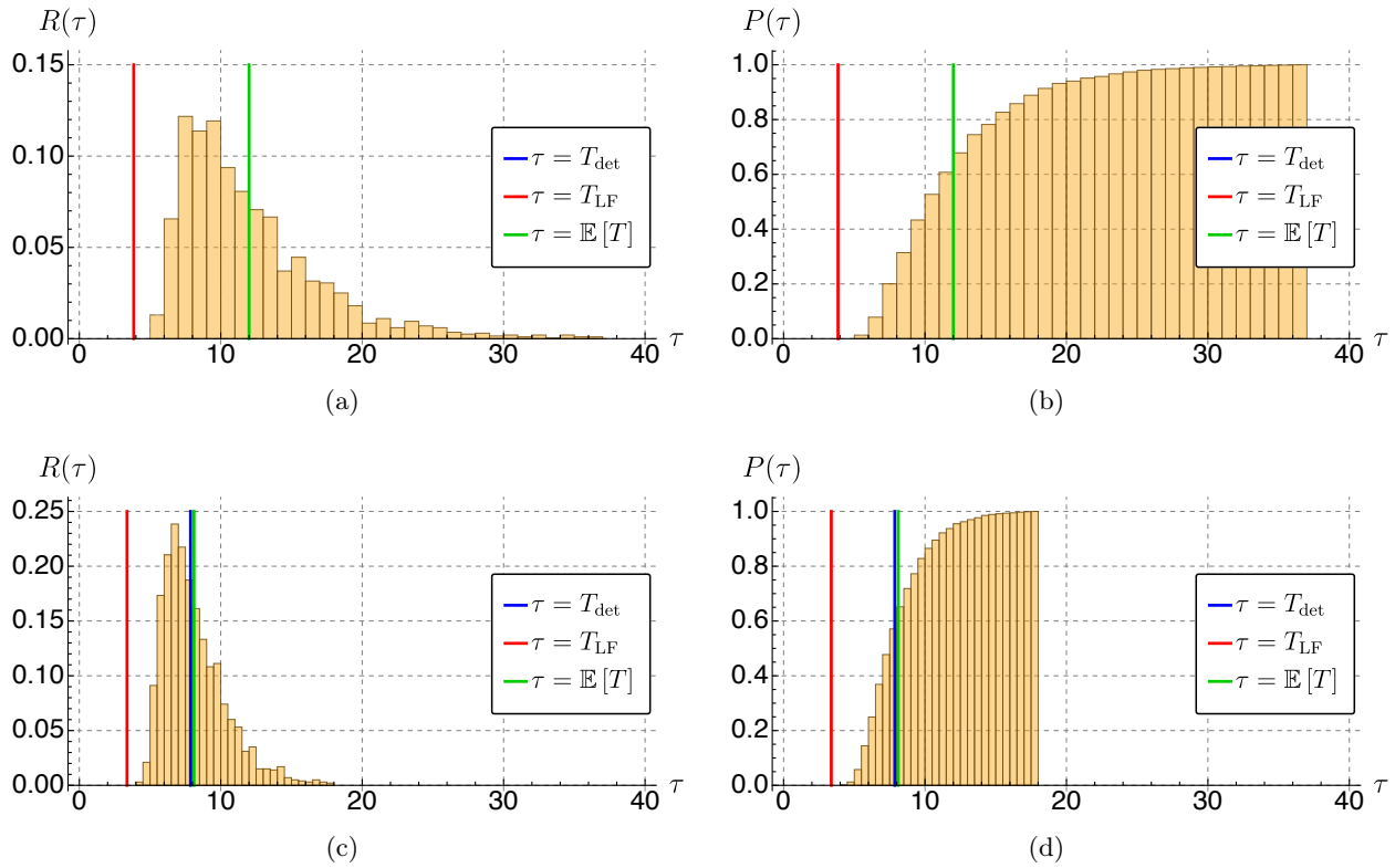
FIGURE E.7. Histograms representing R(\tau) (Figs. E.7(a) and E.7(c)) and P(\tau) (Figs. E.7(b) and E.7(d)). Vertical lines of equations \tau = T_{\text{det}} (blue lines), \tau = T_{\text{LF}} (red lines) and \tau = \mathbb{E}[T] (green lines) are also represented. The same parameters as in Section E.4.2 are used with \rho = 1.8 < \rho_{\text{ml}} (Figs. E.7(a) and E.7(b)) and \rho = 2 > \rho_{\text{ml}} (Figs. E.7(c) and E.7(d)).
