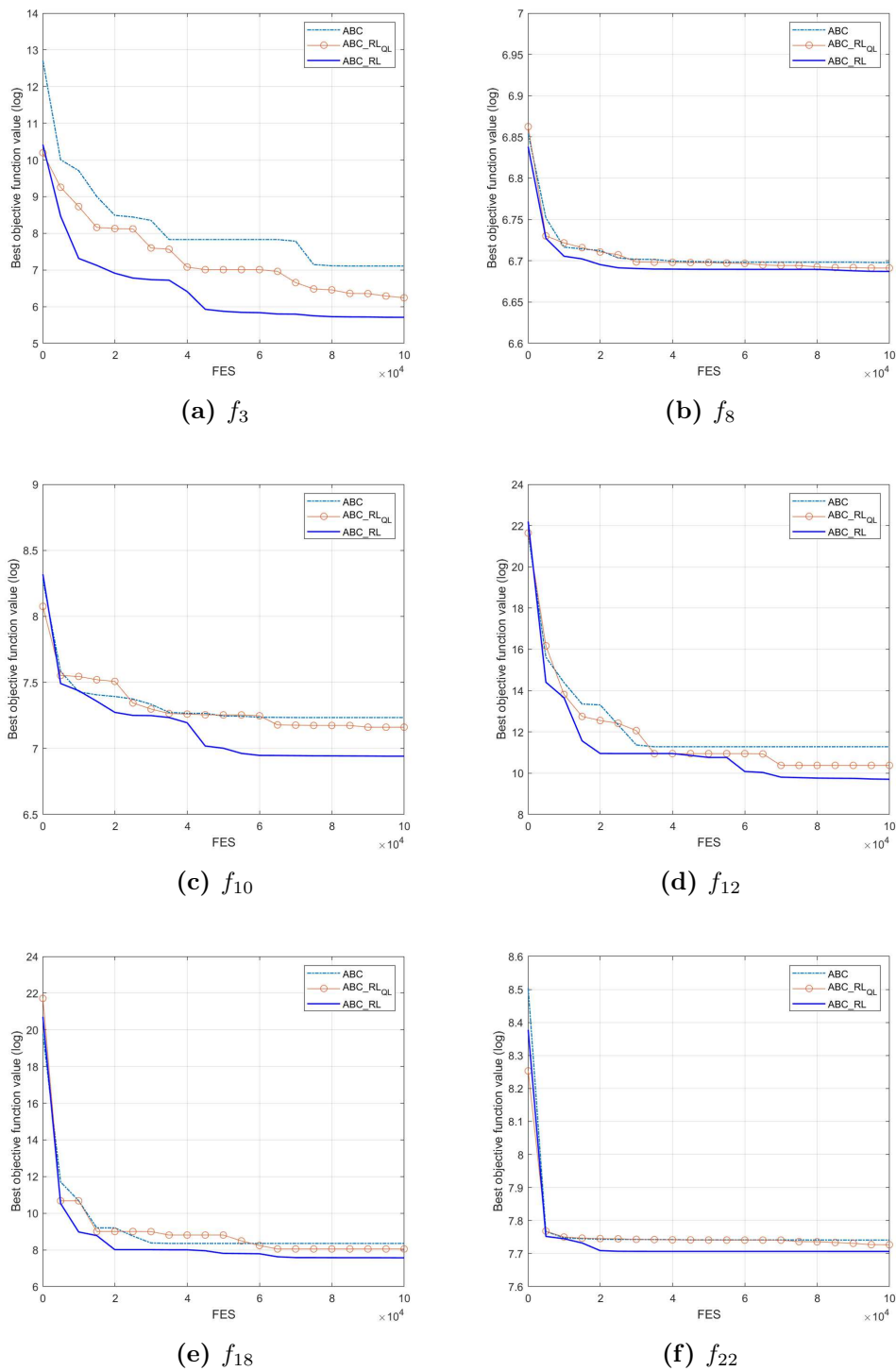
Fig. 3.6. The influence of RL method on convergence rate of ABC algorithm
