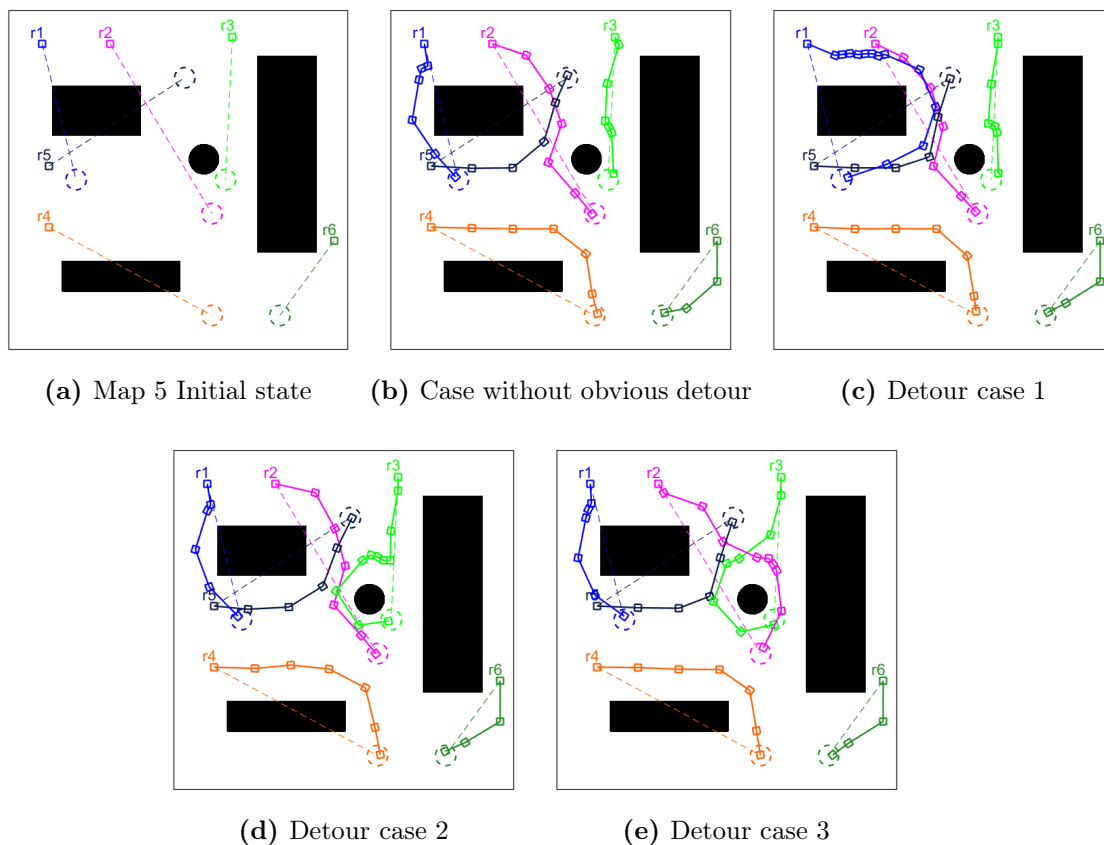
Fig. 6.13. The examples of detours in Map 5 planned by ABC algorithm
