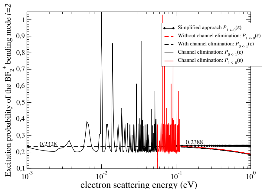
Figure III.6: Vibrational (de-)excitation probabilities, used in Fig. III.5, for transitions between the two lowest vibrational levels of the bending mode of \text{BF}_2^+ . Solid lines represent the results obtained using the complete treatment in addition to the closed-channel elimination procedure in dashed lines. Dotted lines show the results from the simplified approach using Eq. (III.6).
