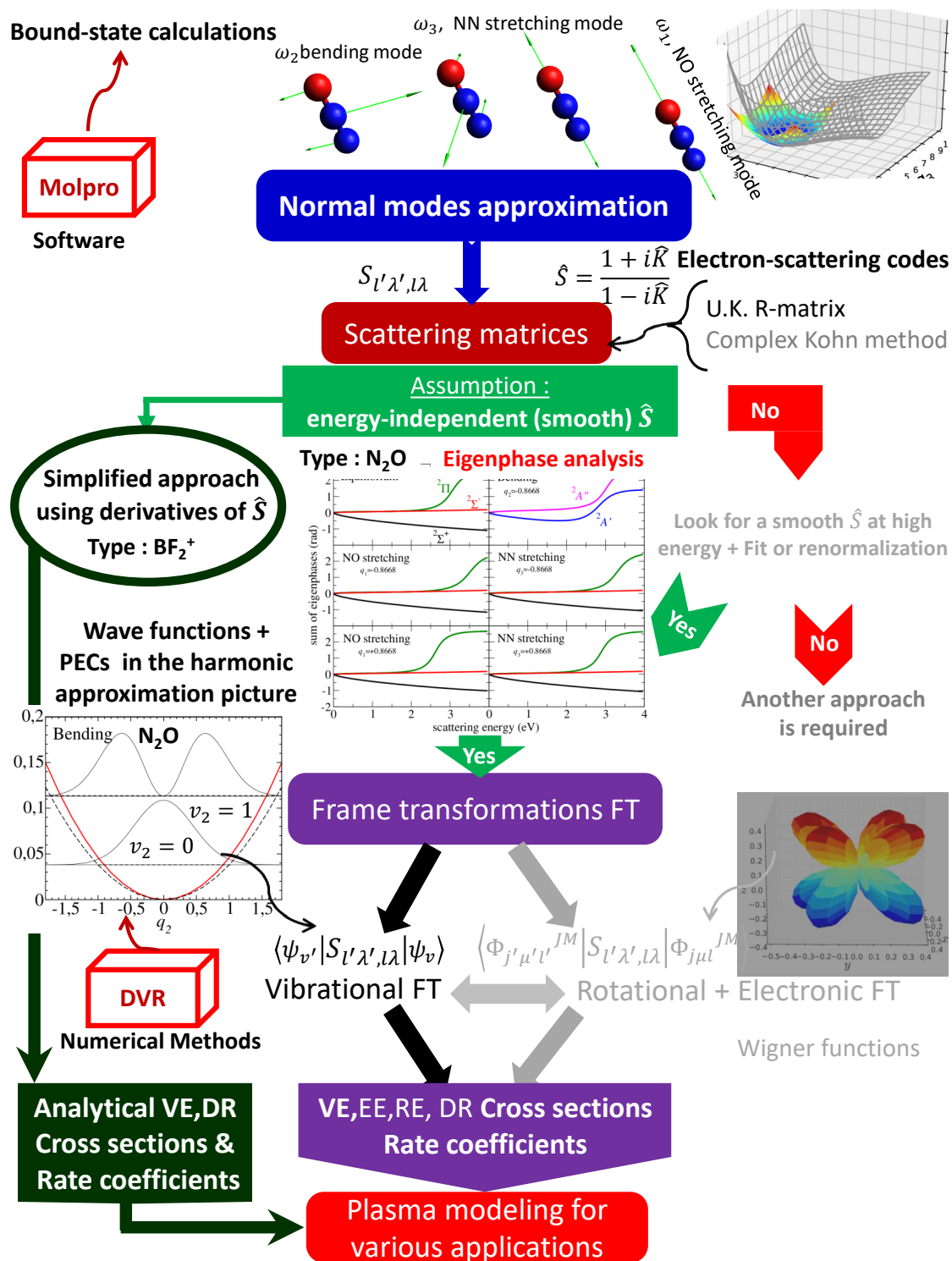
Figure II.1: The flow chart of different ingredients employed in the theoretical model developed for the description of vibrational (de-)excitation (VE) as well as dissociative recombination (DR) of polyatomic molecular ions such as NO_2 , N_2O , CH_2NH_2^+ (described in Chapter I) and BF_2^+ (described in Chapter III). The following abbreviations are used. FT: frame transformation. DVR: discrete variable representation. Tasks or methods in non-bold text are not performed in this HDR yet.
