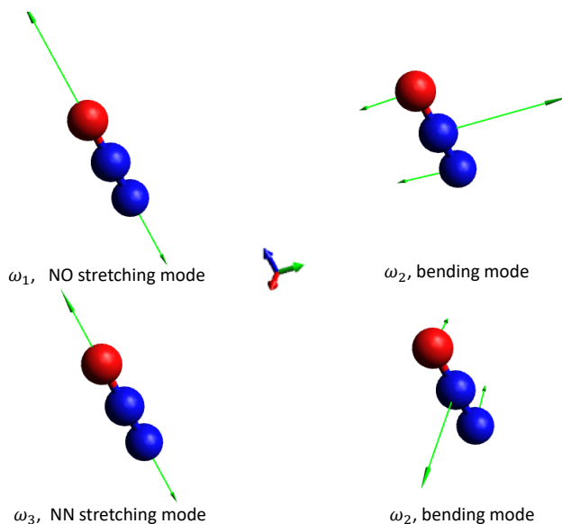
Figure II.14: Normal modes of N 2 O. The arrows indicate the direction and magnitude of displacements for each mode. Note that arrowheads are not shown for the displacements of relatively large magnitudes. Vibrational frequencies and symmetries are listed in Table 1 of paper .6.
