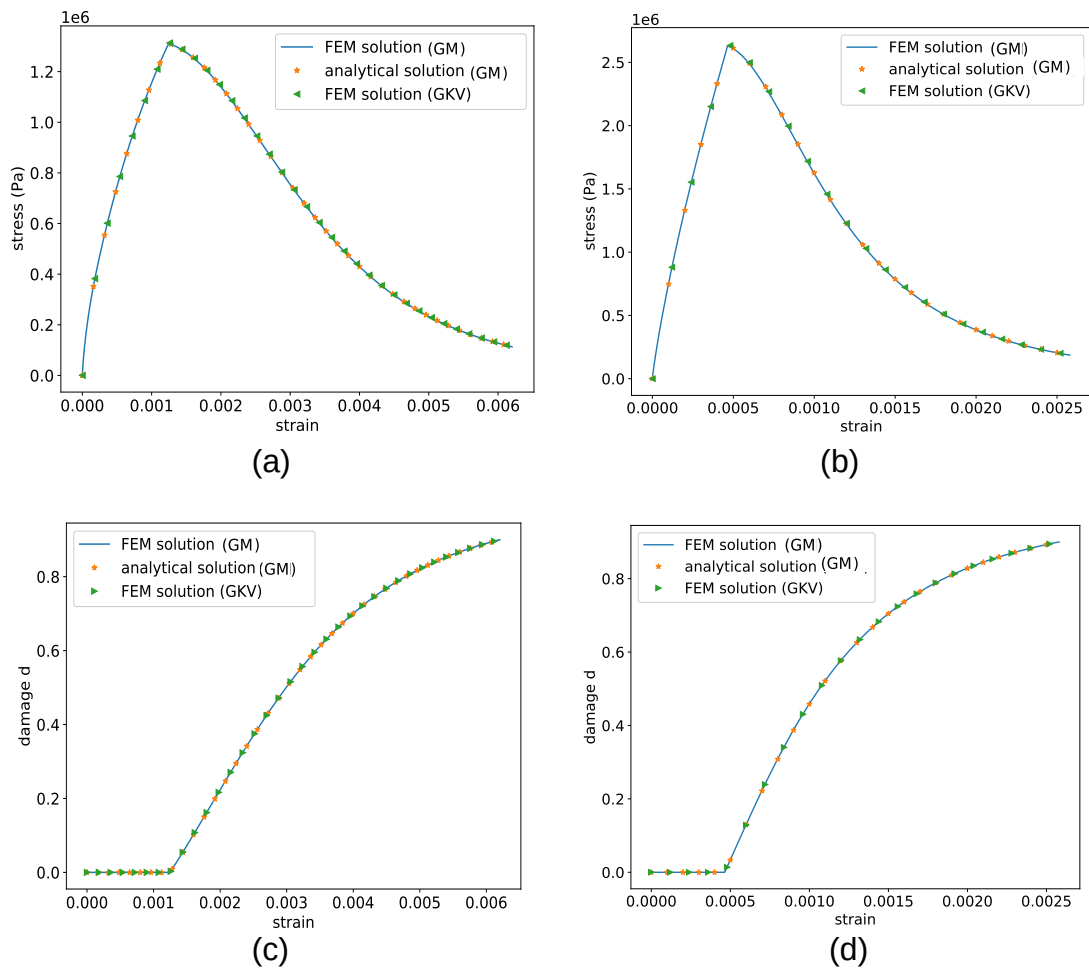
Figure 3.15 – Validation of numerical implementation: Local (or homogeneous) stress-strain plots (top row) and damage evolution plots (bottom row) for \dot{\epsilon}_{\text{mean}} = 1e - 5 \text{ s}^{-1} (left column) and \dot{\epsilon}_{\text{mean}} = 1e - 3 \text{ s}^{-1} (right column)
