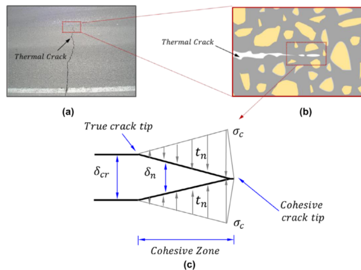
Figure 1.29 – Schematic of CZM [58]
