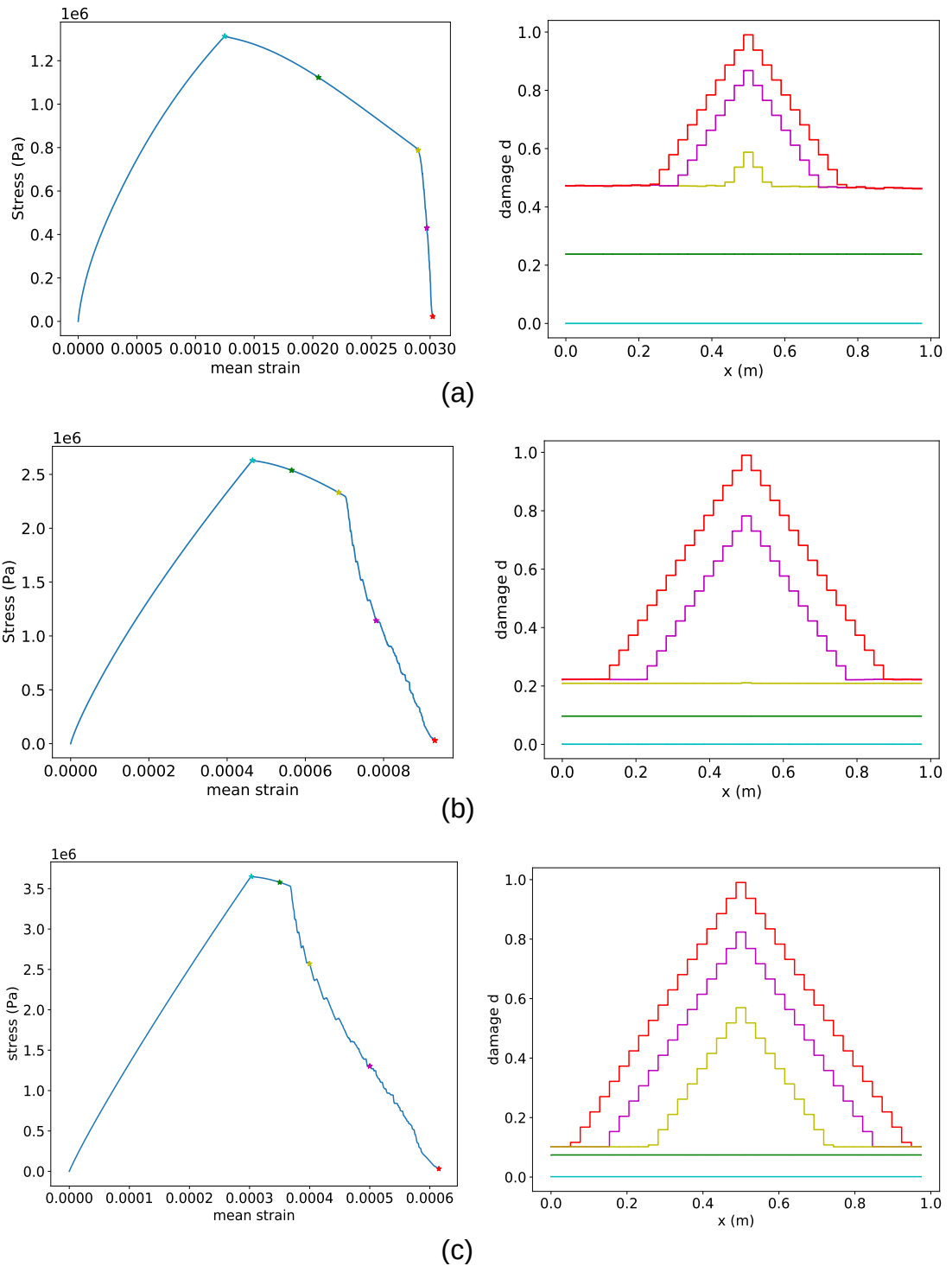
Figure 3.5 – Stress-strain plots and the damage evolution plots for \dot{U} = \{1e - 5, 1e - 3, 1e - 1\} m/s (from top to bottom). The damage profile along the bar is plotted at different time instants indicated by colored bullets in stress-strain plots
