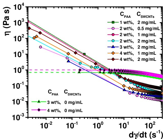
Figure IV.35 Viscosity at low shear rate for some typical examples at pH = 7. A comparison without SWCNTs is shown for the cases of C_{\text{PAA}} = 3 wt% and 4 wt%. It helps to visualize the differences in viscosity when CNTs are added. Dashed lines are linear extrapolations to zero shear viscosity. All lines are a guide to the eye.
