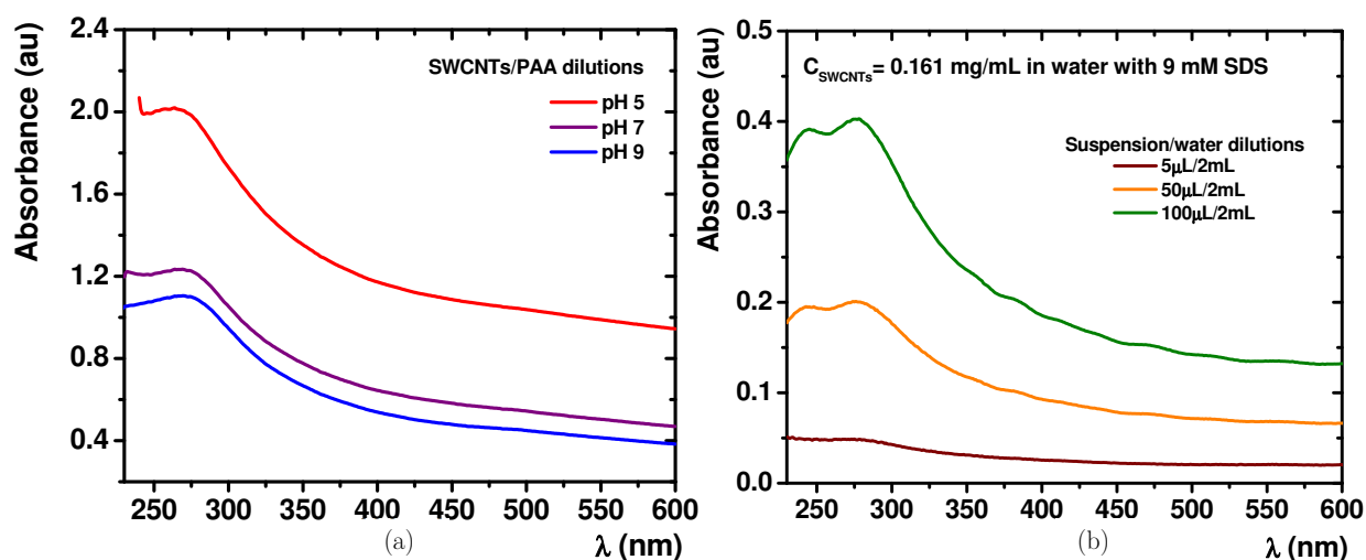
Figure IV.31 (a) UV-vis spectra of SWCNTs/PAA suspensions at different \text{pH} values. C_{\text{SWCNTs}} = 0.02 mg/mL and C_{\text{PAA}} = 2 wt%. (b) The same shape in the spectra for different dilutions of SWCNTs at C_{\text{SWCNTs}} = 0.161 mg/mL, suspended in water with 9 mM SDS.
