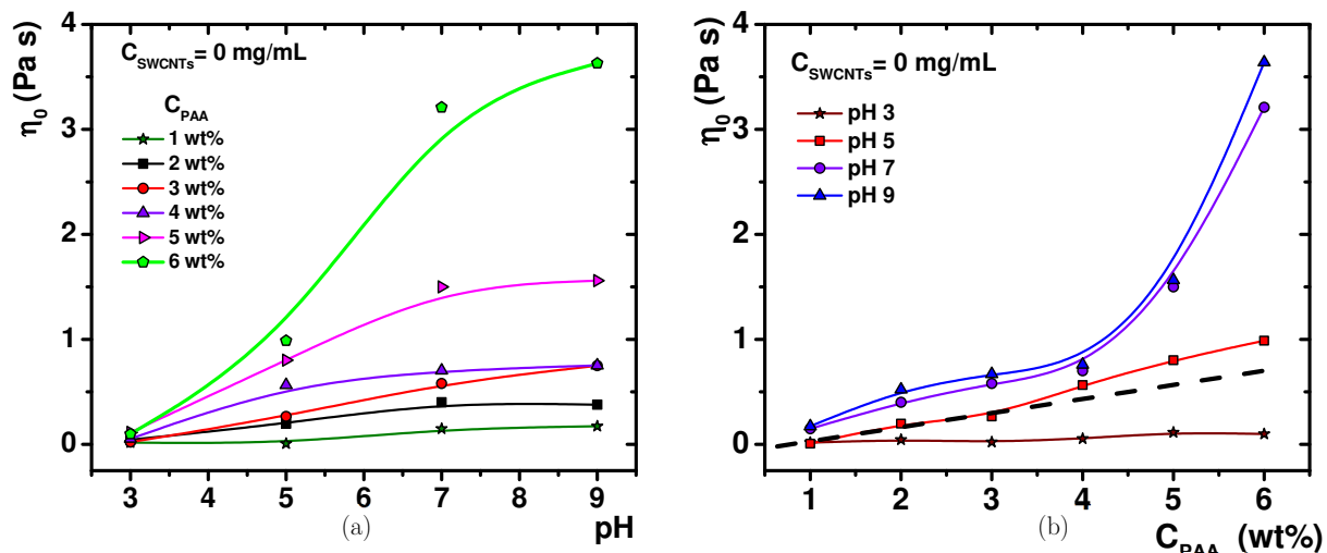
Figure IV.28 (a) \eta_0 vs. pH for different polymer concentrations. Lines are a guide to the eye. (b) \eta_0 vs. C_{PAA} at various pH values. The black dash line at \text{pH} = 5 shows where \eta_0 is no longer linearly dependent on C_{PAA} .
