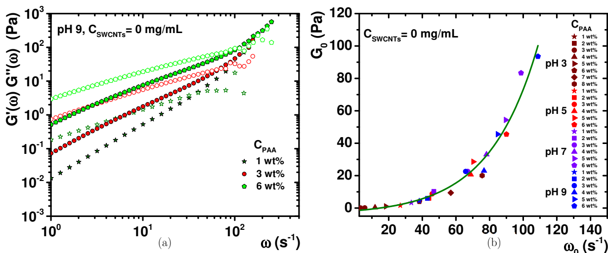
Figure IV.30 Viscoelastic spectra of PAA. (a) G'(\omega) and G''(\omega) as a function of the polyelectrolyte concentration, at constant \text{pH} = 9 . Full symbols are for the elastic modulus, open symbols are for the viscous modulus. (b) The relation between G_0 vs. \omega_0 defined by the crossing points as a function of \text{pH} and concentration. Green line is an exponential fitting for all the crossing points.
