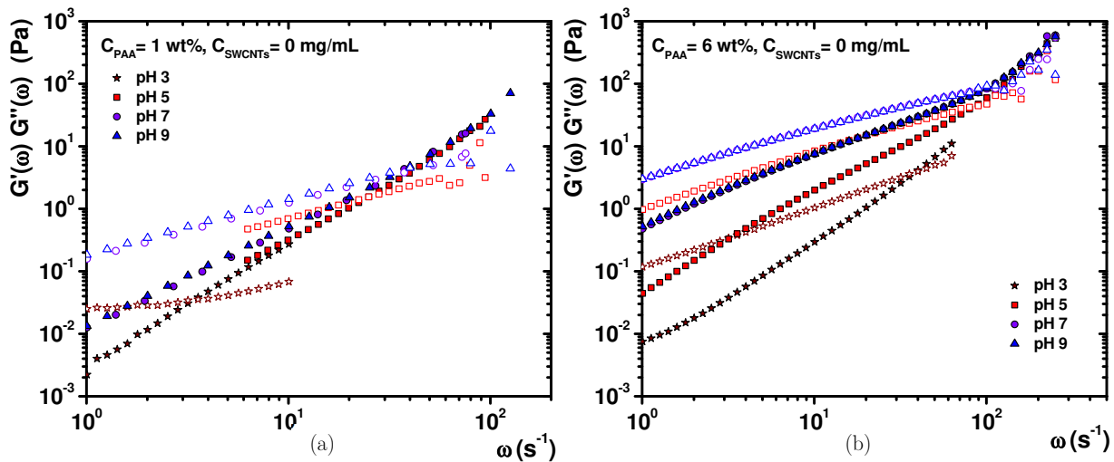
Figure IV.29 Viscoelastic spectra of PAA solutions for different values of concentrations and pH: (a) C_{\text{PAA}} = 1 wt%, (b) C_{\text{PAA}} = 6 wt%. Full symbols are for the elastic modulus, open symbols are for the viscous modulus.
