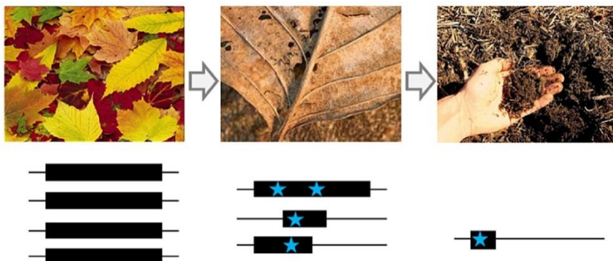
Figure 2: Repeat decay. Metaphorically, repeats are composted over time towards becoming genomic humus. Image taken from publication (Maumus and Quesneville, 2016).
