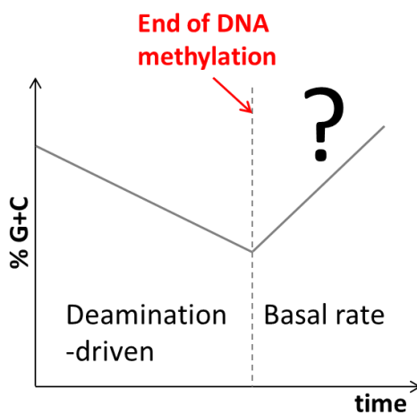
Figure 6: Theoretical evolution of G+C levels in repetitive elements over time: first decreasing owing to deamination events, and then increasing following methylation-free mutational forces.
