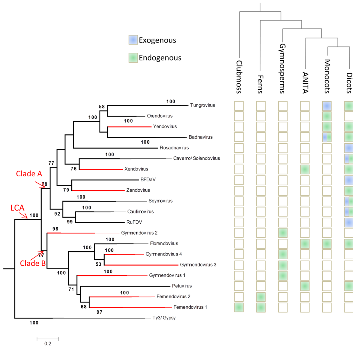
Figure 9: Phylogeny of the Caulimoviridae , as inferred using maximum likelihood criteria and a multiple sequence alignment of protease, reverse transcriptase and ribonuclease H1 domain sequences from recognized (black) and putative (red) genera. The upper cladogram indicates the evolutionary relationships between major classes of vascular plants. At the intersection between both trees, colored boxes indicate the presence of either endogenous (green) or exogenous (blue) representatives of the Caulimoviridae . Image taken from publication (Diop et al., 2017).
