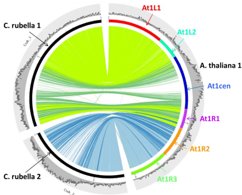
Figure 5: Regular (gray) and deep (dark gray) repeatome annotations on outmost track are positioned along the A. thaliana chromosome 1 (right) and the C. rubella chromosomes 1 (top left) and 2 (bottom left). At1R2 region is orange on the inner band. The central ribbons connect orthologous genes identified by best reciprocal hits and synteny conservation. Ribbons are bold when deep repeatome density in C. rubella exceeds 50%. Image taken from publication (Maumus and Quesneville, 2016).
