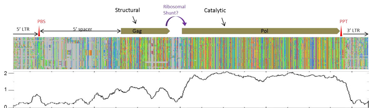
Figure 7: From top to bottom: structural annotation of Habitans elements, overview of multiple sequence alignment of 45 consensus from 17 Brassicaceae species, and inferred conservation plot.
