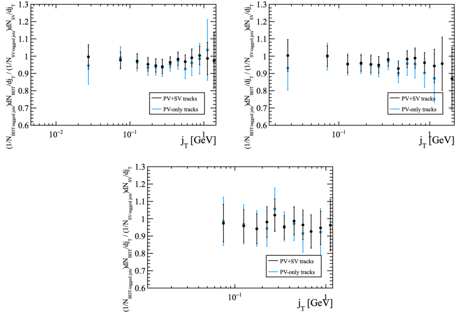
Figure B.11: The bias due to the BDT cut requirement on the c -jet j_T distributions. The bias is calculated in bins of jet p_T : 20-30 GeV (top left), 30-50 GeV (top right), and 50-100 GeV (bottom).
