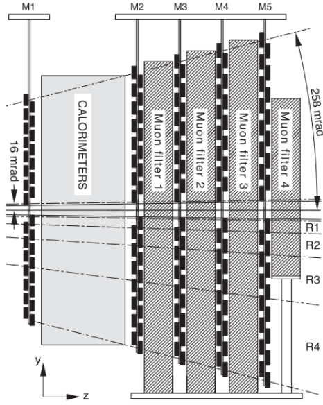
Figure 2.7: A side view of the LHCb Muon System. M1-M5 are the five muon stations composed of MWPCs and GEMs. The four muon filters are iron absorbers. [17]
