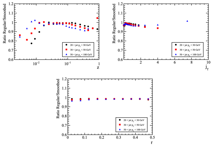
Figure 4.26: The ratios of the z , j_T , and r distributions corrected with the nominal track efficiencies to those corrected with the smoothed track efficiencies.
