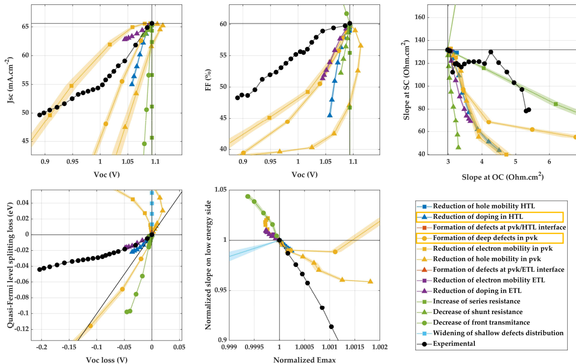
Figure 4-23. Experimental degradation pathway of device JV-PL-1 and associated simulated mechanisms. Two mechanisms are compatible on all planes: formation of defects in the perovskite layer (yellow circles) and reduction of HTL doping (blue triangles).
