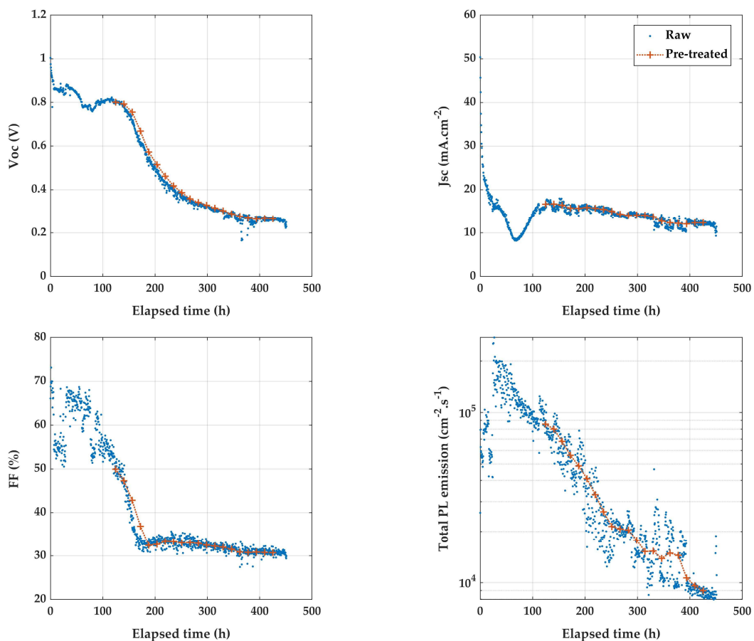
Figure 4-3. Degradation over time of the device JV-PL-4. Only part of the recorded degradation is extracted to be investigated, from 125 to 425 h of aging. All optoelectrical parameters are available in Appendix D, Figure D6.
