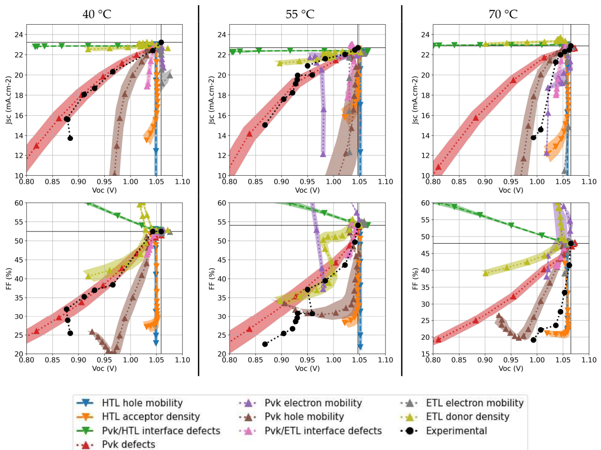
Figure 4-18. Experimental degradation pathways from results published by Lim et al., measured at 40, 55 and 70 °C (left, middle and right respectively). Associated simulated pathways are superposed. Second degradation step is analyzed. Only the second part of the experimental degradation is extracted from respectively 475, 175 and 10 minutes. A formation of defects in the perovskite layer (red) is the closest mechanism at lower temperatures and experimental pathway at 70 °C is close to a reduction of acceptor density in the HTL (orange).
