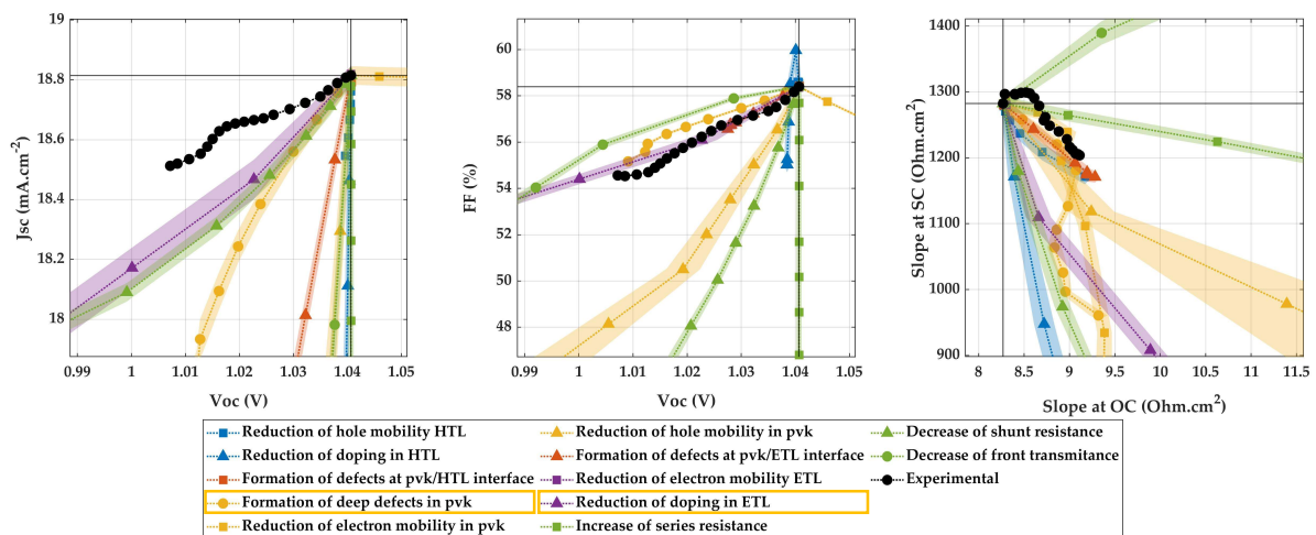
Figure 4-21. Experimental degradation pathway of device JV-3.1 and associated simulated mechanisms. Reduction of ETL doping (purple triangles) and formation of perovskite deep defects (yellow circles) are compatible. Other mechanisms mostly induce too strong Jsc or FF losses.
