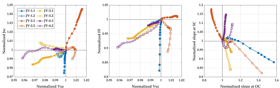
Figure 4-7. Experimental degradation pathways of eight devices characterized through periodic JV measurements. Four techniques were employed to prepare the perovskite solution: the day of deposition or one day before, and with a pre-heating step of the solution or not. The optoelectrical parameters are normalized to the initial value before degradation.
