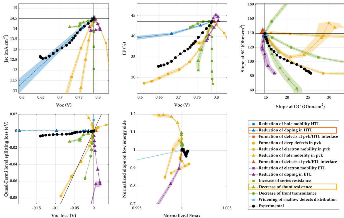
Figure 4-27. Experimental degradation pathway of device JV-PL-5 (starting at 85h) and associated simulated mechanisms. Reduction of doping in HTL (blue triangles) is close to the experiment but decrease of shunt resistance (green triangles) is also compatible.
