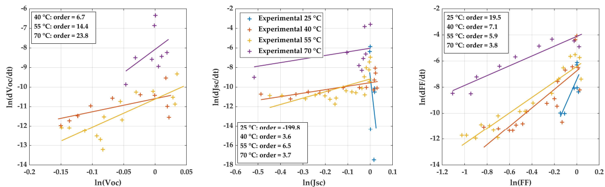
Figure 4-6. Normalized V_{oc} , J_{sc} and FF reported by Lim et al., plotted as \log\left(\frac{dX}{dt}\right) versus \log(X) (crosses). Linear regressions are displayed in plain lines and give estimations of reaction orders.
