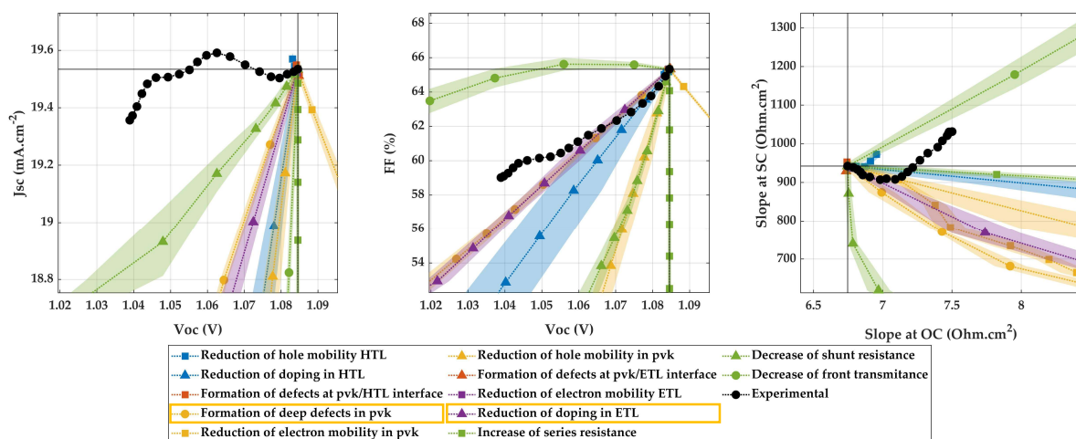
Figure 4-22. Experimental degradation pathway of device JV-4.2 and associated simulated mechanisms. No simulated mechanism explains such a stable J_{sc} . However, a loss of ETL doping (purple triangles) and formation of defects in perovskite layer (yellow circles) can't be totally excluded.
