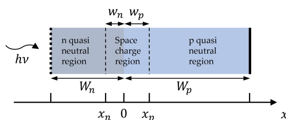
Figure 4-10. Considered pn junction for analytical model. Illumination arises upon n doped side.
