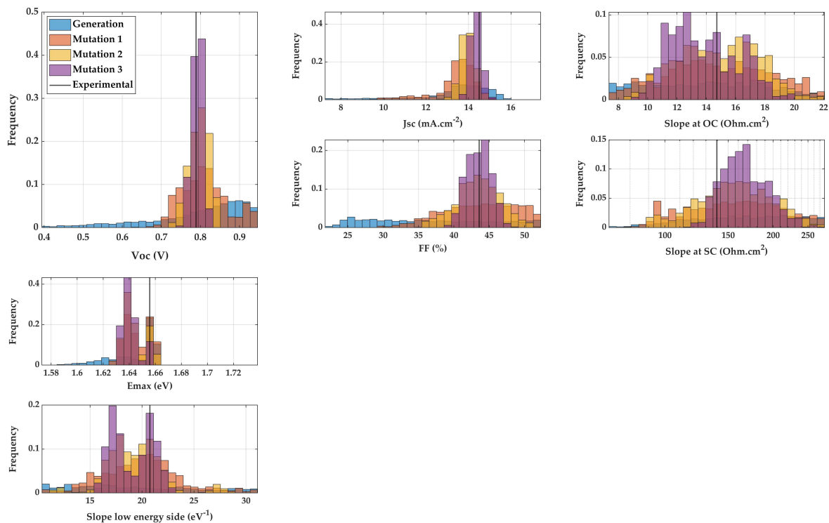
Figure 3-4. Distribution of optoelectrical parameters at each generation and mutation step of the genetic algorithm for the device JV-PL-5.
