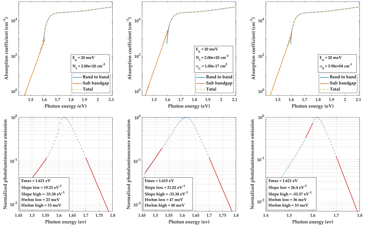
Figure 2-8. Top: absorption coefficient computed from three models for sub-bandgap absorption, and from experimental ellipsometry measurements for band-to-band. The sum of hole and electron generation contributions is directly displayed. Bottom: associated photoluminescence spectrum obtained by performing optical and electrical simulations with the above absorption coefficient. Left: Lucovsky model. Middle: constant model. Right: Katahara-Hillhouse model.
