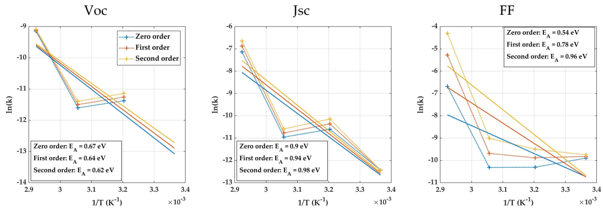
Figure 4-5. Arrhenius plots of the temperature dependence of reaction rates for V_{oc} , J_{sc} and FF (left middle and right, respectively) are displayed with crosses and dotted lines. Associated linear regressions (plain lines) provide activation energy through the slope. The negative reaction rate obtained for V_{oc} at 25 °C with all orders is responsible for the blank in left graph.
