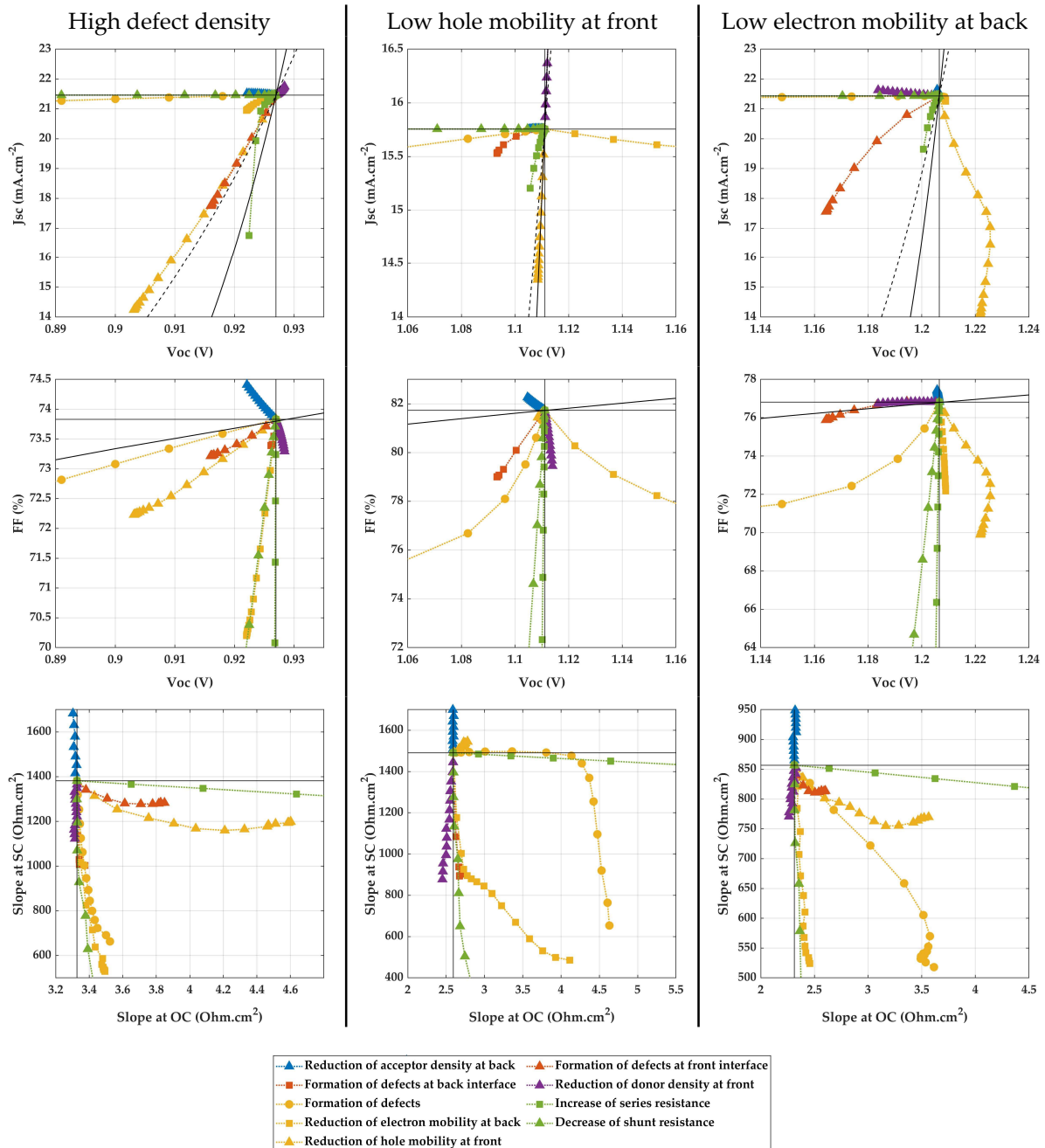
Figure 4-11. Simulated degradation pathways obtained through analytical model of a pn junction. Left column: high defect density ( 10^{17} \text{ cm}^{-3} ). Middle column: low hole mobility in n doped front layer ( 0.1 \text{ cm}^2 \cdot \text{V}^{-1} \cdot \text{s}^{-1} ). Right column: low electron mobility in p doped back layer ( 0.1 \text{ cm}^2 \cdot \text{V}^{-1} \cdot \text{s}^{-1} ). All input parameters are in Appendix D, Table D1. On J_{sc} - V_{oc} graphs, plain and dashed black lines show the J_{sc} - V_{oc} relation according to the single diode model, with ideality factor equal to 1 and 2, respectively.
