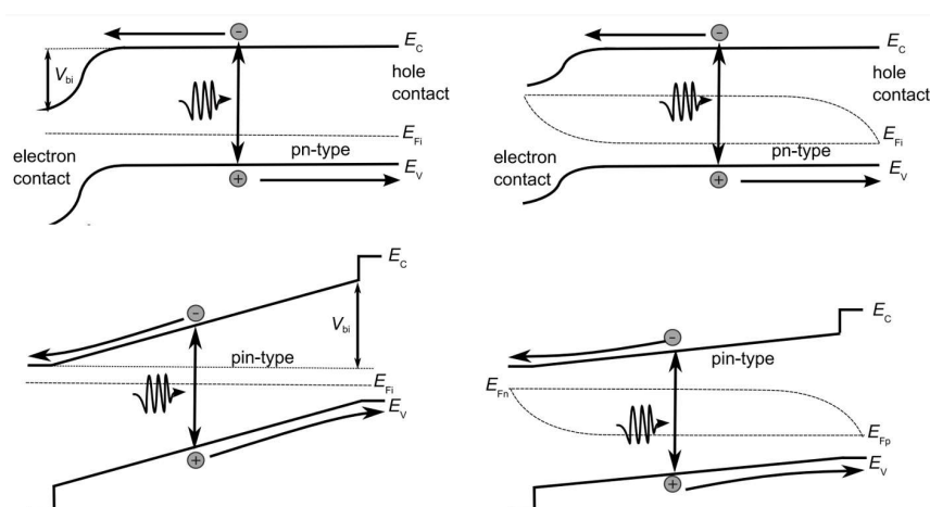
Figure 1-1. Band diagram of a pn (top) and pin (bottom) solar cell. Left is at short circuit and right is under a positive bias. Figure is extracted from [8]
