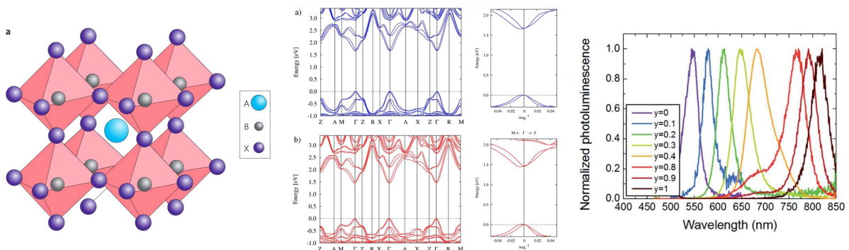
Figure 1-3. Left: single crystal of perovskite with cubic structure [12]. Middle: band structure of exemplary compositions with two A site cations: MAPbI_3 and FAPbI_3 , top and bottom respectively [13]. Right: photoluminescence emission spectra of FAPbI_yBr_{3-y} thin films [14].
