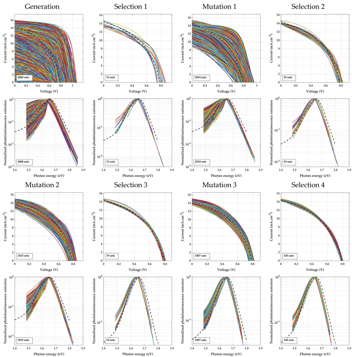
Figure 3-3. JV characteristics and PL spectra generated and selected at each step of the genetic algorithm for the device JV-PL-5. Dotted lines show the experimental JV characteristic and PL spectrum.
