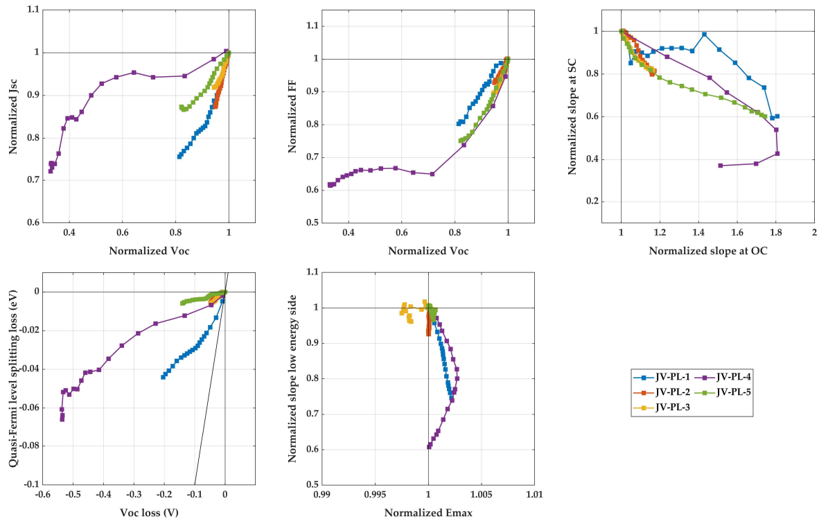
Figure 4-8. Experimental degradation pathways of five devices characterized through periodic JV and PL measurements. Aging sequence of JV-PL-4 and JV-PL-5 starts at 125 and 85 h respectively. The optoelectrical parameters are normalized to their initial value before degradation.
