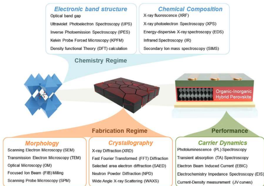
Figure 1-5. Summary of main characterization techniques employed to investigate perovskite solar cells stability. Extracted from [76]
