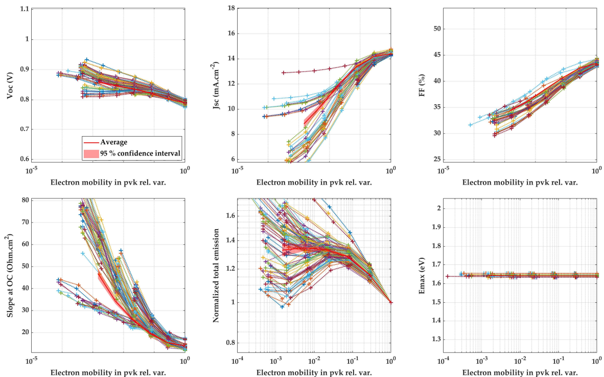
Figure 3-8. Simulated response to a decrease of the electron mobility in the perovskite. The 105 inputs sets reproducing the initial performances of JV-PL-5 are subjected to the same mechanism and represented with dotted lines and crosses. Average and 95 % confidence intervals are calculated at each degradation step.
