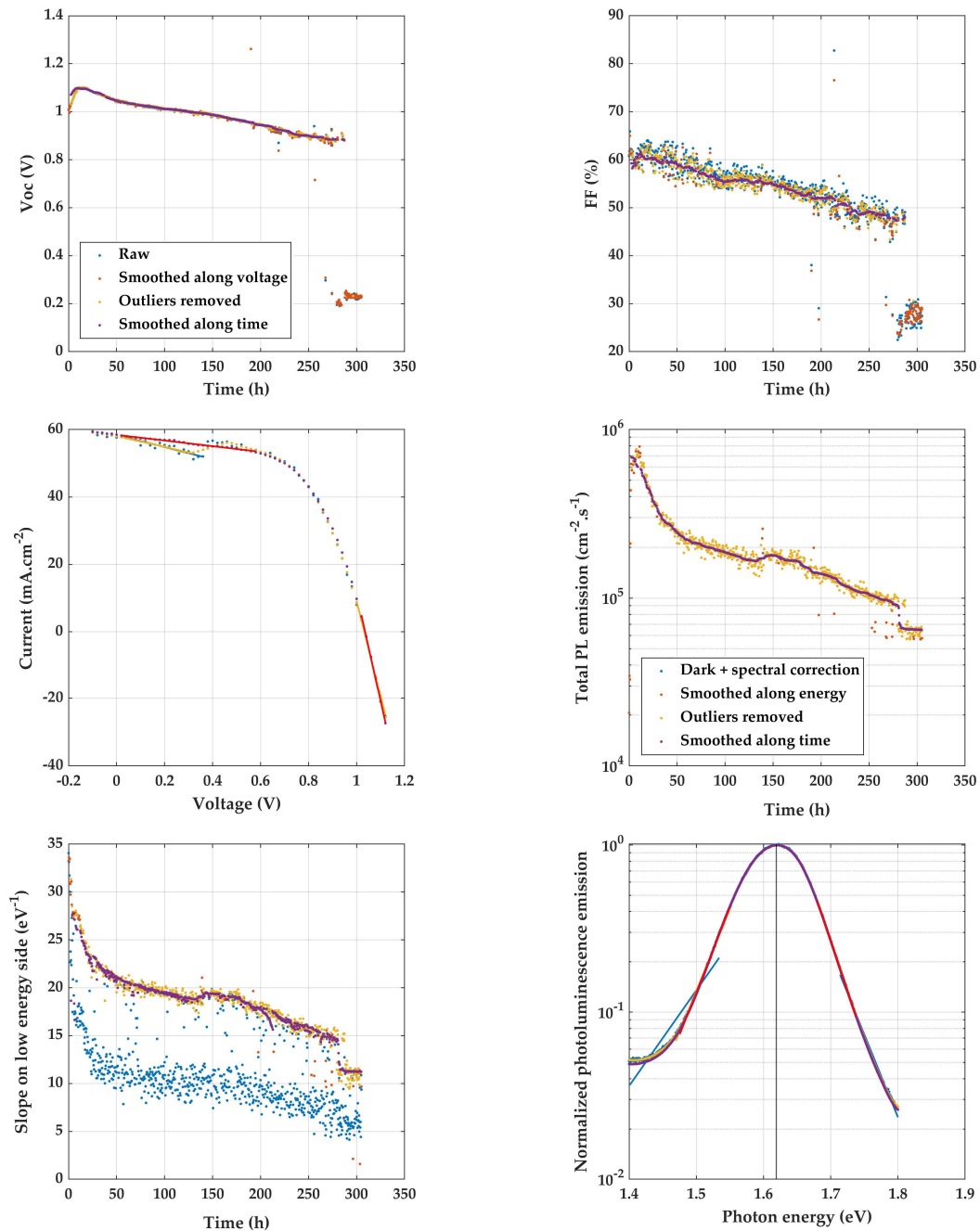
Figure 2-13. Degradation over time of device JV-PL-1 (reverse JV measurements). The parameters are extracted from the JV characteristics and PL spectra at each step of the pre-treatment. Example of JV characteristic and PL spectrum were measured at 62 h of aging. Other optoelectrical parameters are displayed in Appendix B, Figure B5.
