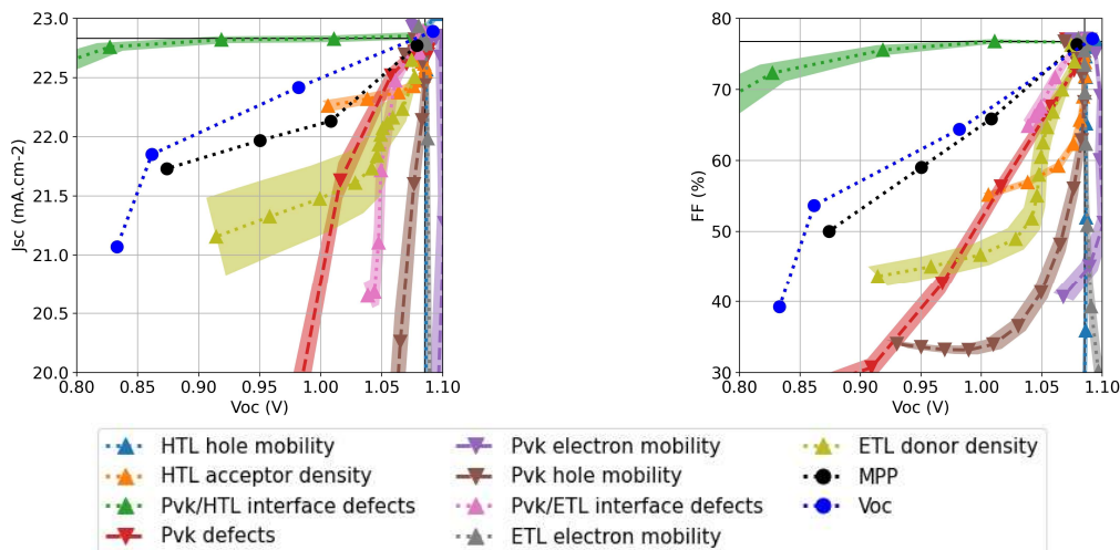
Figure 4-15. Experimental degradation pathways from results published by Li et al. : devices were aged under one sun, N 2 atmosphere, at 35 °C and tracked at maximum power point or kept at open circuit voltage. Associated simulated pathways are superposed (down triangles and dashed lines for causes identified by authors, up triangles and dotted lines for others). A formation of defects in the perovskite layer (red) is the closest mechanism explaining experimental degradation.
