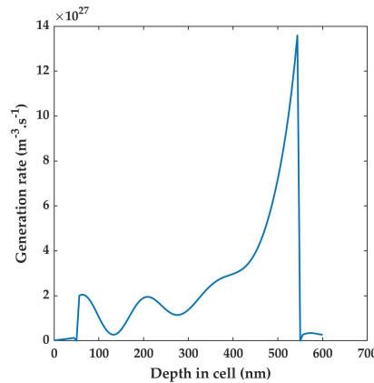
Figure 2-2. Generation rate in an exemplary perovskite solar cell. Note x axis starts at the bottom interface and light enters through the side at 600 nm. Only the ETL / perovskite / HTL stack is represented. Both transport layers are 50 nm thick, and the perovskite 500 nm.
