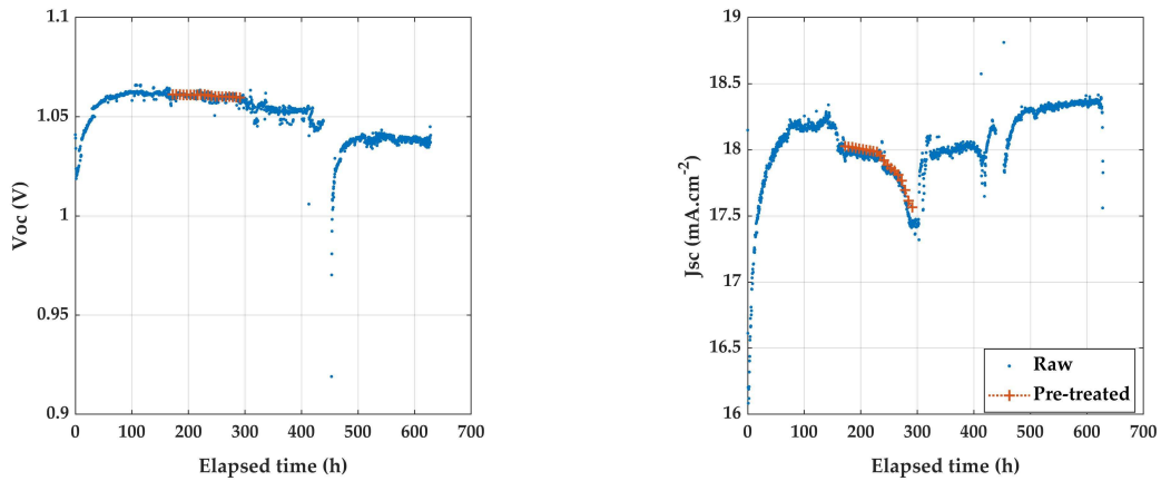
Figure 4-1. Degradation over time of the device JV-1.1. Only part of the recorded degradation is extracted to be investigated, from 170 to 290 h of aging. All optoelectrical parameters are displayed in Appendix D, Figure D1.
