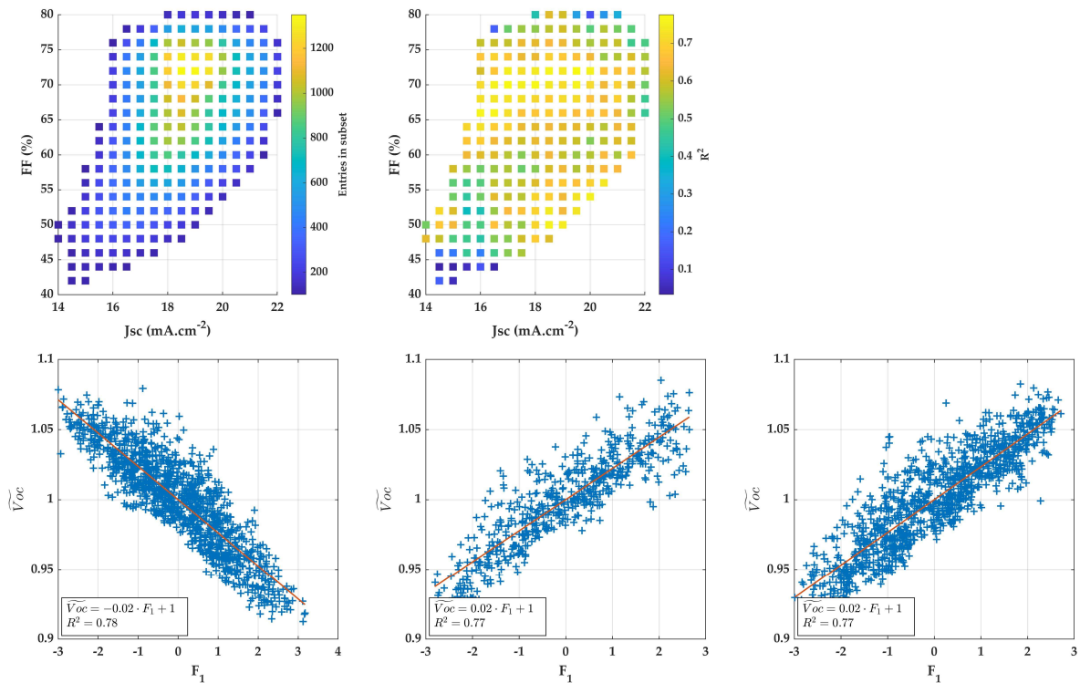
Figure E11. Top: size of selected subsets for considered J_{sc} -FF couples and associated R^2 values for the linear regression of V_{oc} with the first component. Bottom: correlation plot of first component with variable output parameter, in the three best cases of R^2 value.
