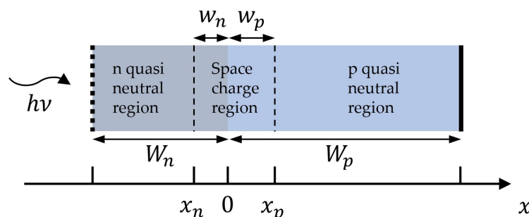
Figure 1-2. Considered pn junction and associated x axis. Zero is at the interface and illumination arises upon n doped side.
