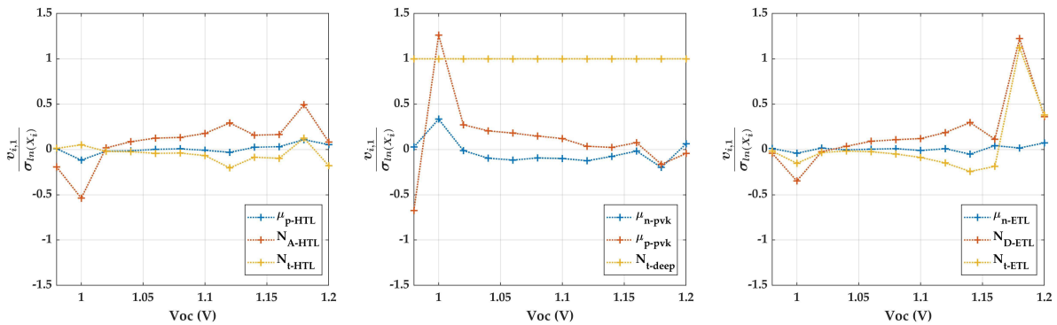
Figure 5-3. Exponents of the first component for fixed values of Voc. For each point, entries within 25 mV are aggregated. Associated standard deviations are stable in the range 1.05 – 1.1 V, see Appendix E, Figure E8.
