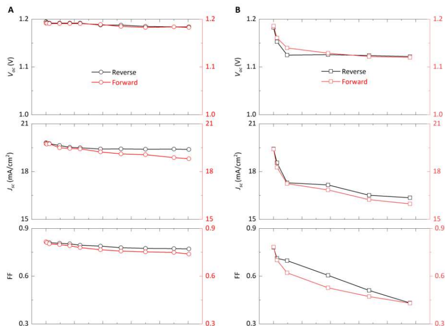
Figure 2-9. Evolution of JV parameters reported by Peng et al. , for devices fabricated with P3HT:CuPc (left) and Spiro-OMeTAD (right) HTL. Aging conditions were 85 °C, 85 % relative humidity and dark.
