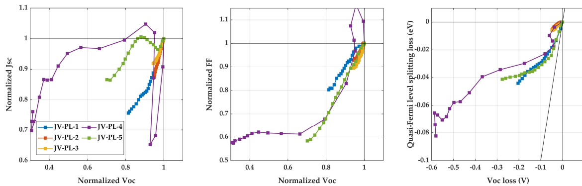
Figure 4-9. Experimental degradation pathways of five devices characterized through periodic JV and PL measurements. Aging sequence of JV-PL-4 and JV-PL-5 starts at 25 and 20 h respectively. The optoelectrical parameters are normalized to their initial value before degradation.
