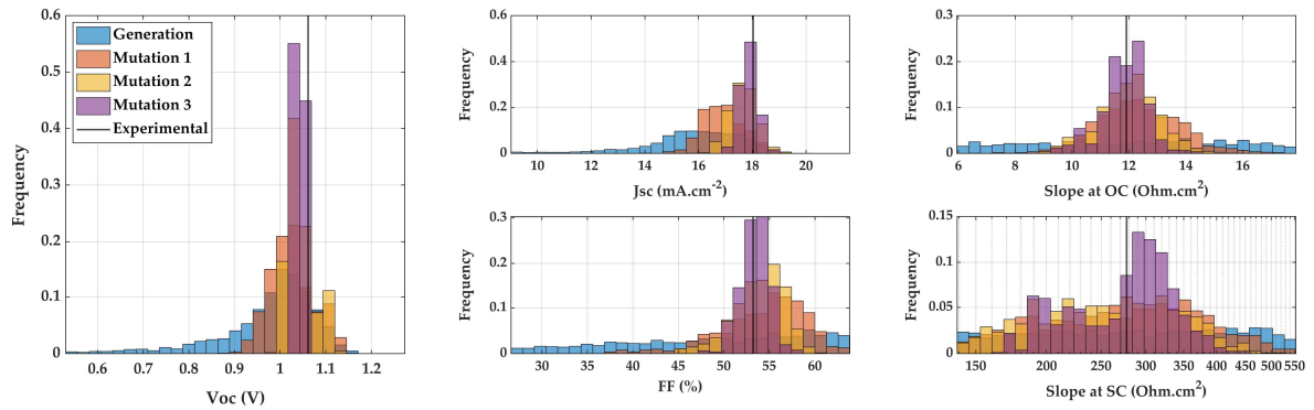
Figure 3-2. Distribution of optoelectrical parameters at each generation and mutation step of the genetic algorithm for the device JV-1.1.
