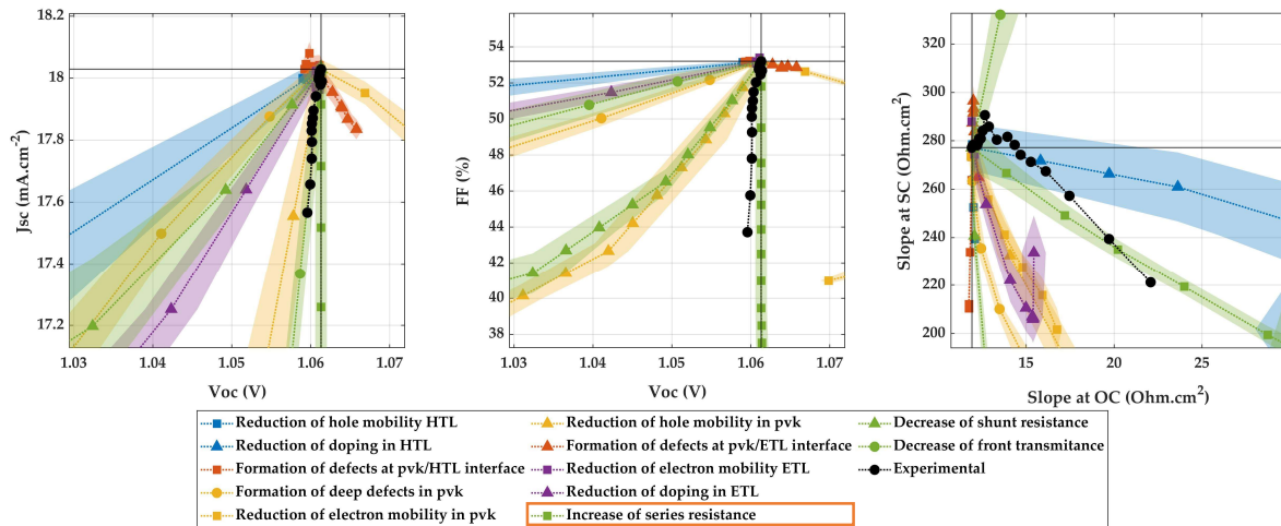
Figure 4-19. Experimental degradation pathway of device JV-1.1 and associated simulated mechanisms. The increase of external series resistance (green squares) is very close to experiment.
