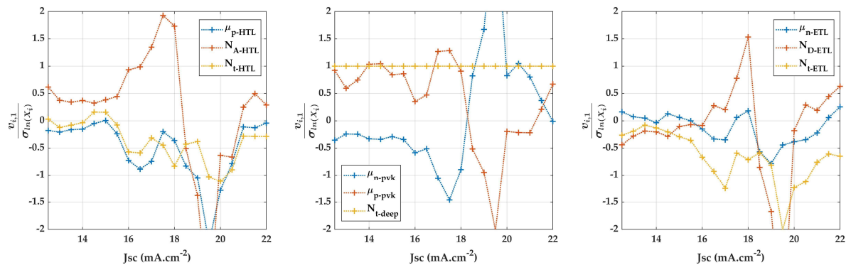
Figure 5-4. Exponents of the first component for fixed values of Jsc. For each point, entries within 1 mA.cm -2 are aggregated. Associated standard deviations are stable above 16 mA.cm -2 , see Appendix E, Figure E9.
