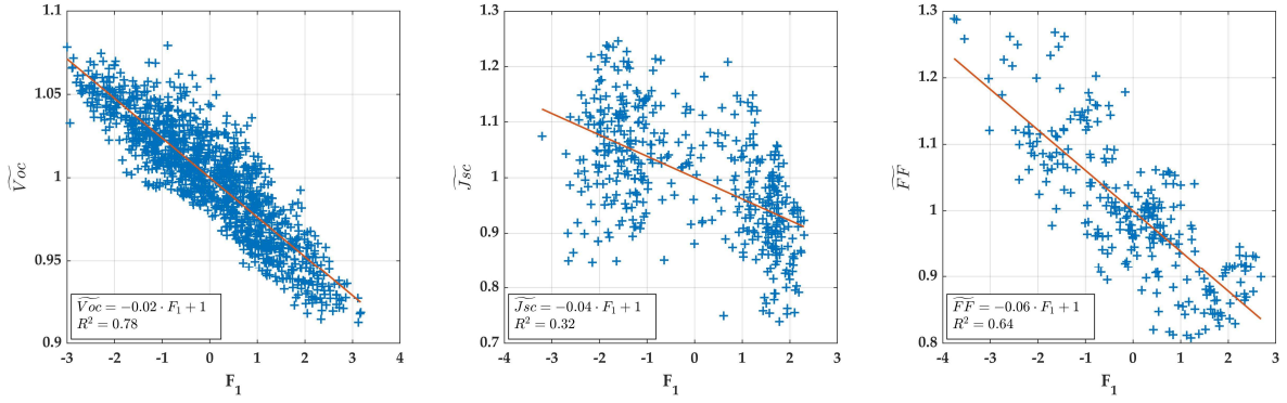
Figure 5-6. Correlation plot of first component with variable output parameter, in the examples of Table 5-4. The linear regression quantifies the correlation strength.
