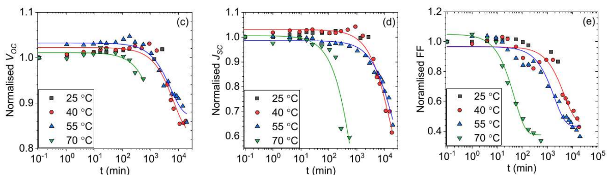
Figure 2-10. Evolution of JV parameters reported by Lim et al. , recorded at 25, 40, 55 and 70 °C. Extracted from [32]
