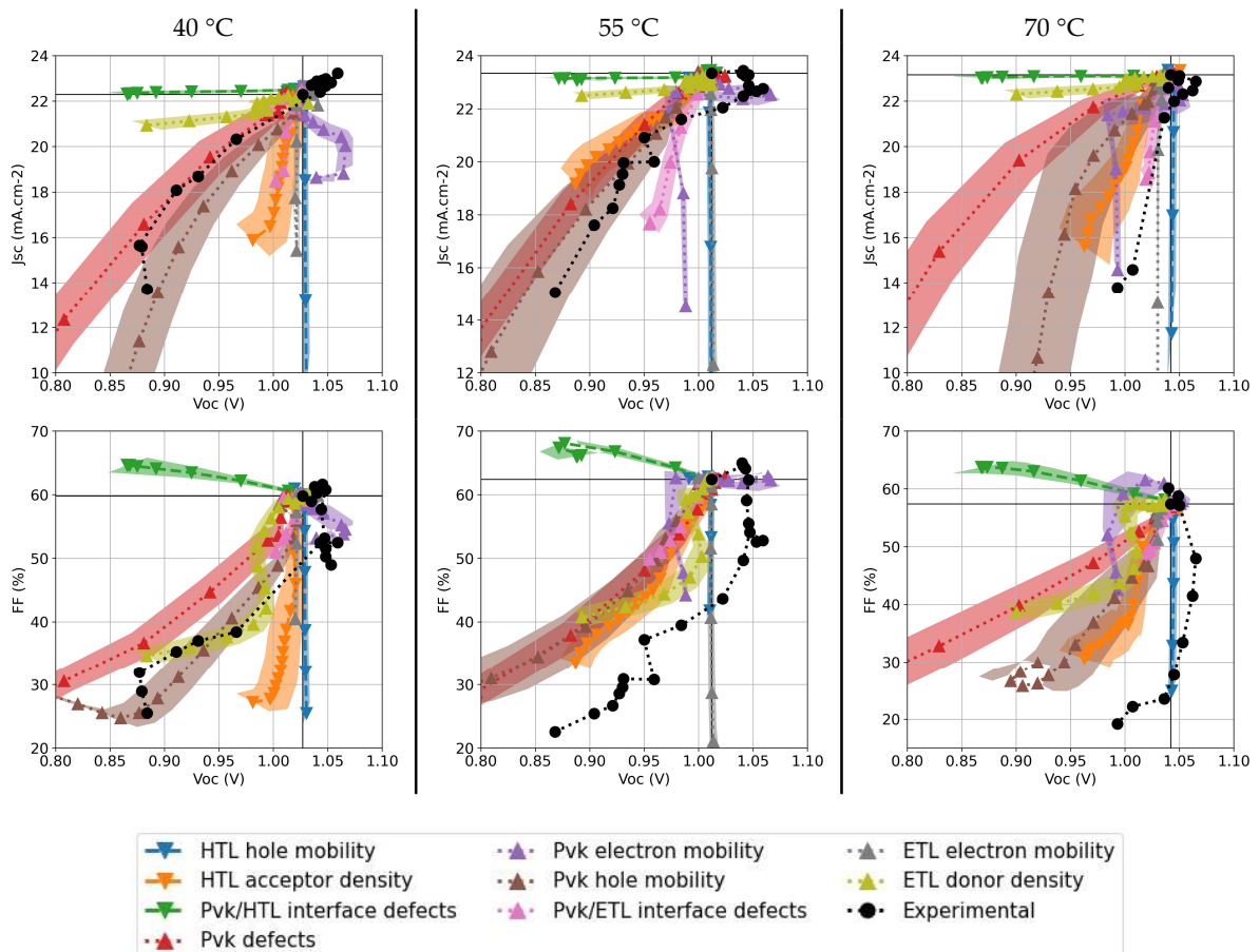
Figure 4-17. Experimental degradation pathways from results published by Lim et al.: perovskite devices were aged under one sun, air and at 40, 55 or 70 °C (left, middle, and right respectively). Associated simulated pathways are superposed (down triangles and dashed lines for causes identified by authors, up triangles and dotted lines for others). At 40 and 55 °C, the closest mechanism is a loss of hole mobility (brown) or a formation of defects (red) in the perovskite layer. At 70 °C, a reduction of hole mobility in HTL (blue) is closer to experimental results.
