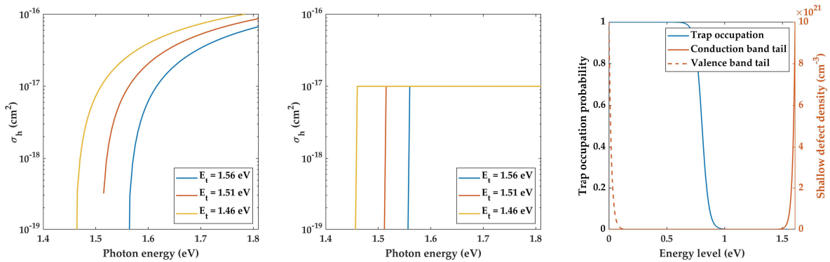
Figure 2-7. Optical capture cross section for three defect state energy levels. Left: Lucovsky model, the effective mass was set to its value in the valence band and the refractive index to its average value in the known range. Middle: constant model, \sigma_c was set to 10^{-17} cm 2 . Right: trap occupation probability across the perovskite bandgap material, assuming it is intrinsic and at equilibrium. The shallow defects from both band tails are also superposed.
