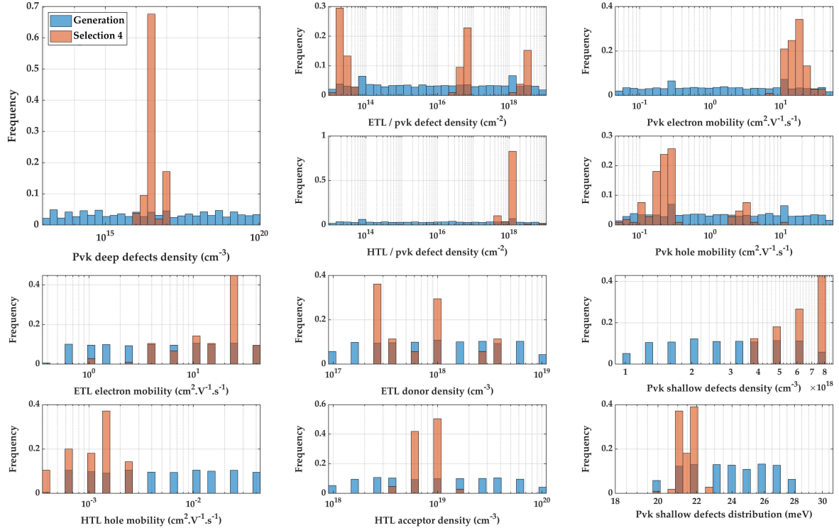
Figure 3-6. Frequency distribution of material parameters in the initial generation and after the final selection step of the genetic algorithm for the device JV-PL-5. The number of counts per bin in the histogram is normalized by the total number of sets.
