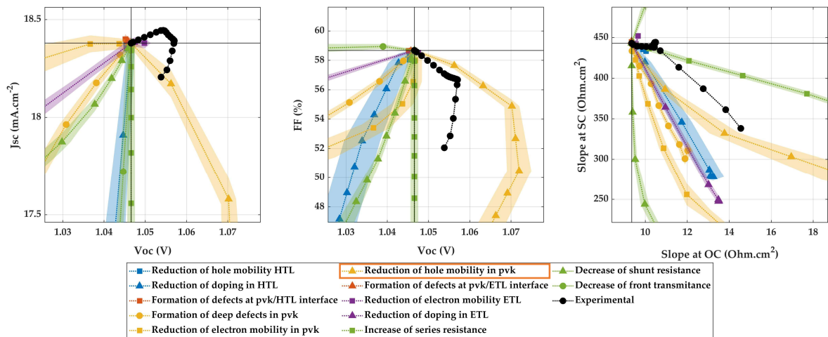
Figure 4-20. Experimental degradation pathway of device JV-2.2 and associated simulated mechanisms. The reduction of hole mobility in perovskite (yellow triangles) is compatible, other mechanisms do not induce an increase of Voc.
