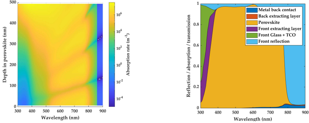
Figure 2-1. Left: absorption rate in the perovskite layer of an exemplary solar cell. Note vertical axis starts at the bottom interface and light enters through the side at 500 nm. Right: absorptivity in the perovskite layer as well as all other absorptions and reflections.
