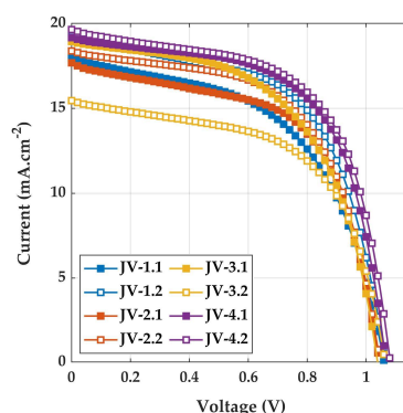
Figure B1. Initial JV characteristics of the eight devices characterized through periodic JV measurements. Four techniques were employed to prepare the perovskite solution: the day of deposition or one day before, and with a pre-heating step of the solution or not.
