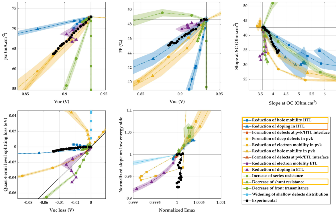
Figure 4-24. Experimental degradation pathway of device JV-PL-2 and associated simulated mechanisms. Reduction of HTL doping (blue triangles) is the most compatible, but reduction of hole mobility in HTL (blue squares), reduction of ETL doping (purple triangles), or reduction of shunt resistance (green triangles) can't be totally excluded.
