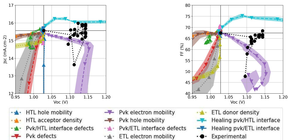
Figure 4-16. Experimental degradation pathways from results published by Chen et al. : perovskite devices were unencapsulated and aged under ambient conditions. Associated simulated pathways are superposed (down triangles and dashed lines for causes identified by authors, up triangles and dotted lines for others). A decrease of electron mobility in perovskite layer (purple) is the closest mechanism explaining experimental degradation.
