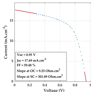
Figure 2-5. Example of current voltage and associated optoelectrical parameters. Slopes at OC and SC are represented through red lines.
