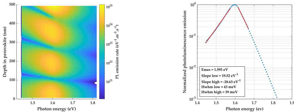
Figure 2-6. Left: photoluminescence emission rate simulated across the depth of a perovskite layer within a solar cell. The same structure as employed for the simulations in Figure 2-1 and Figure 2-3 is employed. Right: corresponding emitted photoluminescence spectrum at the surface of the device.
