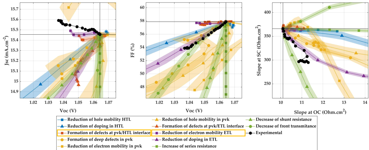
Figure D11. Experimental degradation pathway of device JV-3.2 and associated simulated mechanisms. No simulated mechanism explains the increase of J_{sc} . Reduction of electron mobility (purple squares) or formation of defects at pvk – HTL interface (red squares) could still be compatible with experiment.
