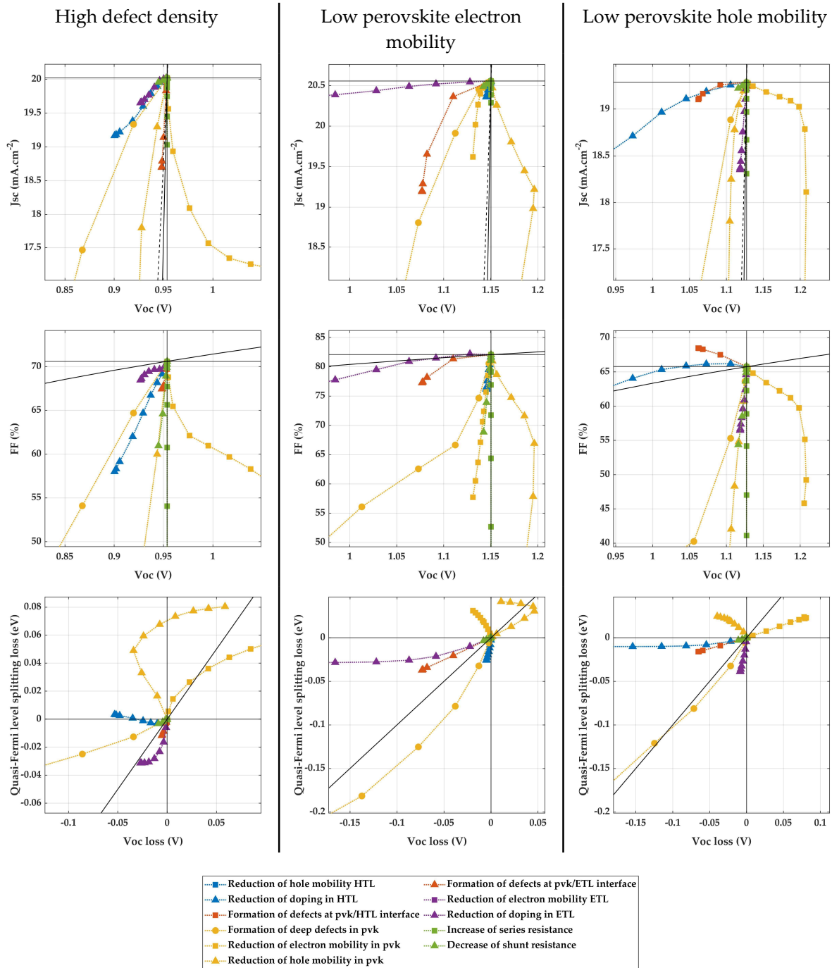
Figure 4-13. Simulated degradation pathways obtained through drift diffusion simulations of a perovskite solar cell. Left: high defect density ( 10^{17} \text{ cm}^{-3} ). Middle: low perovskite electron mobility ( 0.01 \text{ cm}^2 \cdot \text{V}^{-1} \cdot \text{s}^{-1} ). Right: low perovskite hole mobility ( 0.01 \text{ cm}^2 \cdot \text{V}^{-1} \cdot \text{s}^{-1} ). All material parameters are in Appendix D, Table D2.
