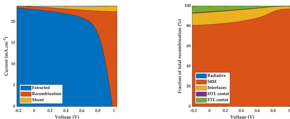
Figure 2-4. Simulation of currents balance across a JV characteristic. Left: balance of extracted current (the actually recorded JV characteristic) and losses through recombination or external shunt resistance. Right: composition of recombination losses. Interfaces refers to perovskite-ETL and perovskite-HTL interfaces. Contacts refers to the outside interfaces of the transport layers.
