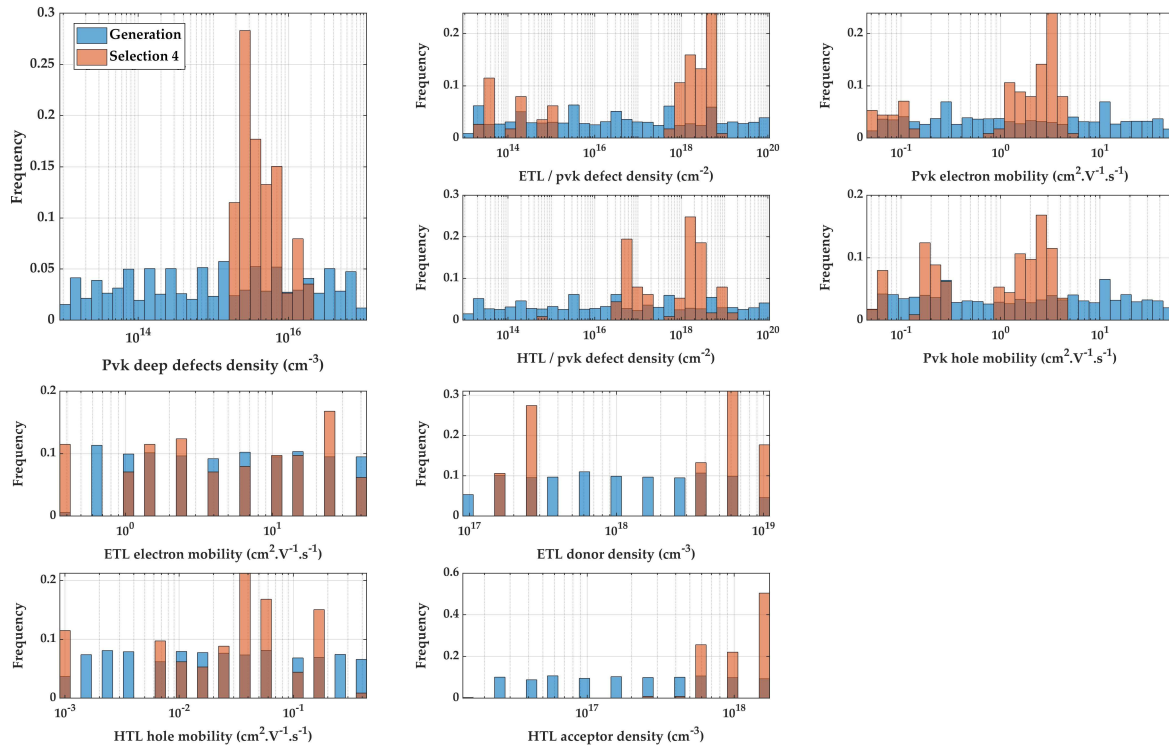
Figure 3-5. Frequency distribution of material parameters in the initial generation and after the final selection step of the genetic algorithm for the device JV-1.1. The number of counts per bin in the histogram is normalized by the total number of sets.
