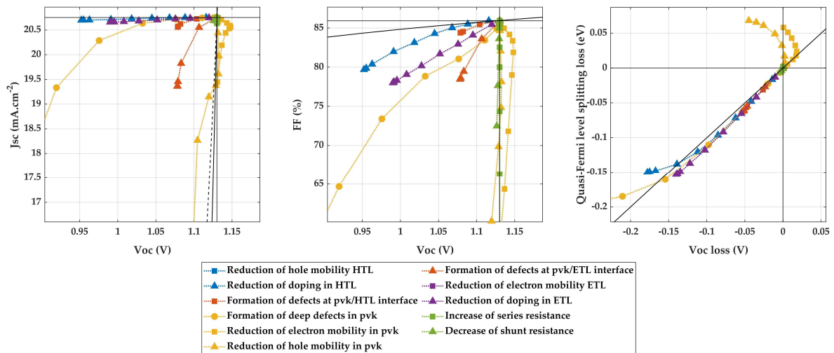
Figure 4-12. Simulated degradation pathways obtained through drift diffusion simulations of a perovskite solar cell. Exemplary hypothetical device with good material qualities (details are in Appendix D, Table D2).
