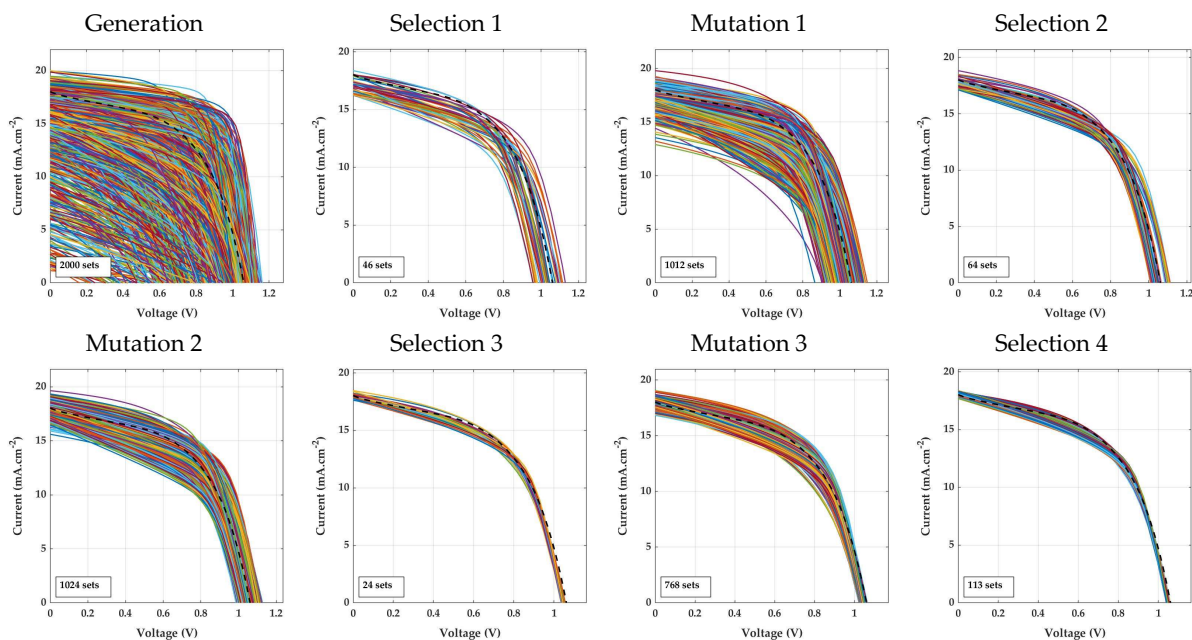
Figure 3-1. JV characteristics generated and selected at each step of the genetic algorithm for the device JV-1.1. Dotted line shows the experimental JV characteristic.
