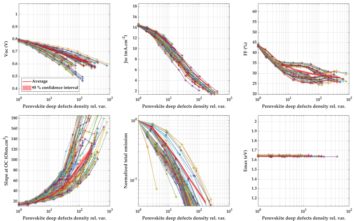
Figure 3-7. Simulated response to an increase of defect density in the perovskite layer. The 105 inputs sets reproducing the initial performances of JV-PL-5 are subjected to the same mechanism and represented with dotted lines and crosses. Average and 95 % confidence intervals are calculated at each degradation step.
