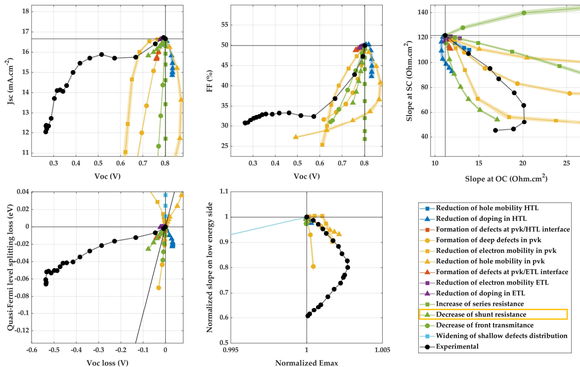
Figure 4-26. Experimental degradation pathway of device JV-PL-4 (starting at 125 h) and associated simulated mechanisms. No mechanism reproduces the large Voc drop accompanied with stable Jsc. Decrease of shunt resistance (green triangles) might not be excluded.
