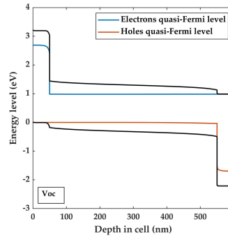
Figure 2-3. Example of output of the electrical simulation of a perovskite solar cell. The quasi-Fermi levels are in blue and red lines, conduction and valence bands in black lines. The applied bias here is V_{oc} .
