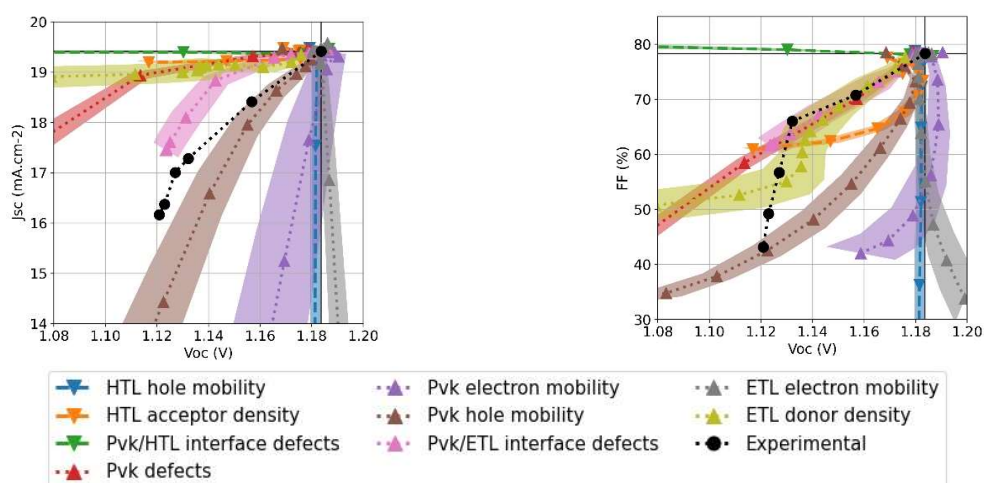
Figure 4-14. Experimental degradation pathways from results published by Peng et al.: perovskite devices were aged under dark, at 85 °C and 85 % relative humidity. Associated simulated pathways (average over 98 material parameters sets used to reproduce initial performances) are superposed (down triangles and dashed lines for causes identified by authors, up triangles and dotted lines for others). A formation of defects at ETL/perovskite interface (pink) or a decrease of hole mobility in perovskite layer (brown) are the two closest mechanisms explaining experimental degradation.
