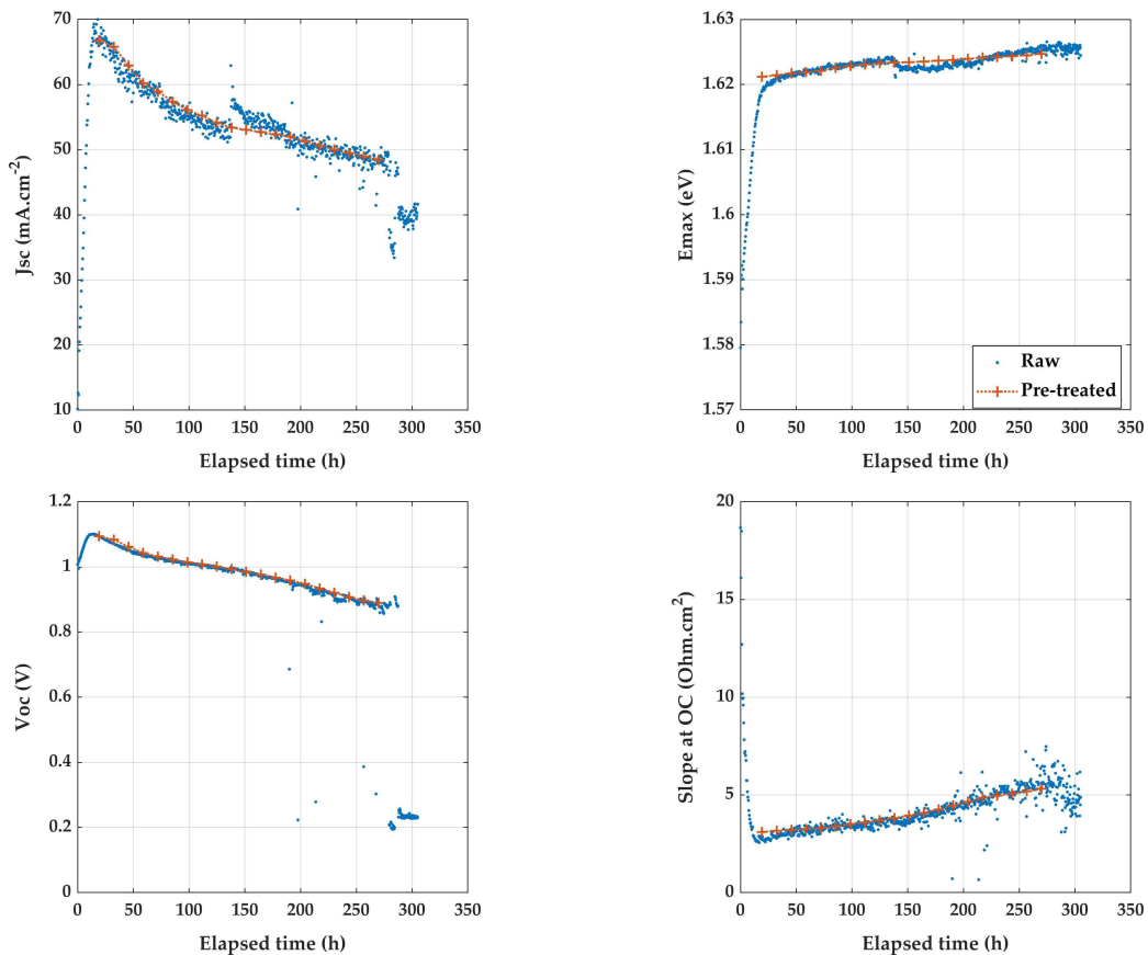
Figure 4-2. Degradation over time of the device JV-PL-1. Only part of the recorded degradation is extracted to be investigated, from 20 to 272 h of aging. All optoelectrical parameters are available in Appendix D, Figure D4.
