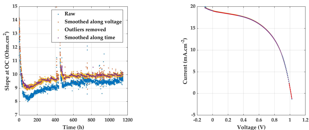
Figure 2-12. Degradation over time of device JV-3.1 for forward measurements. Slope at OC is extracted from the JV characteristics at each step of the pre-treatment. Right show an example of JV characteristic, at 850 h of aging. . Other optoelectrical parameters are displayed in Appendix B, Figure B4.
