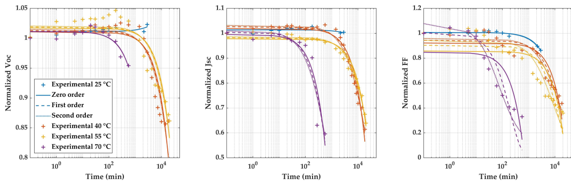
Figure 4-4. Evolution of normalized optoelectrical parameters reported by Lim et al (crosses). Perovskite devices were aged under one sun, air and at 25, 40, 55 or 70 °C. Fittings of the three investigated reaction orders are in lines.
