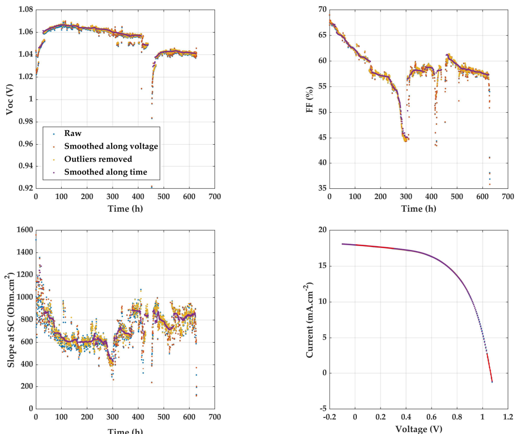
Figure 2-11. Degradation over time of device JV-1.1 for reverse measurements. The parameters are extracted from the JV characteristics at each step of the pre-treatment. Bottom right shows an example of JV characteristic, at 190 h of aging. Other optoelectrical parameters are displayed in Appendix B, Figure B3.
