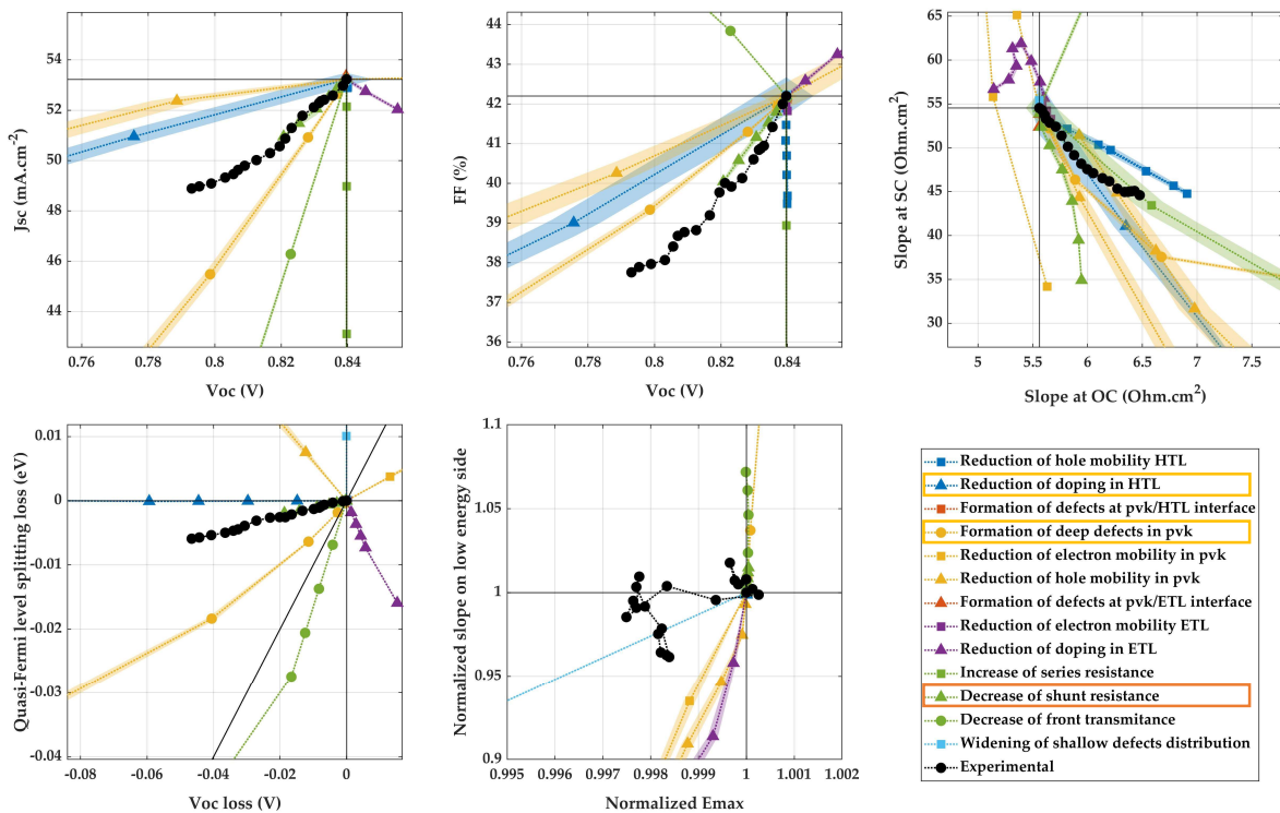
Figure 4-25. Experimental degradation pathway of device JV-PL-3 and associated simulated mechanisms. Reduction of shunt resistance (green triangles) is the closest mechanism. Formation of defects in the perovskite layer (yellow circles) and reduction of HTL doping (blue triangles) are also compatible with experiment.
