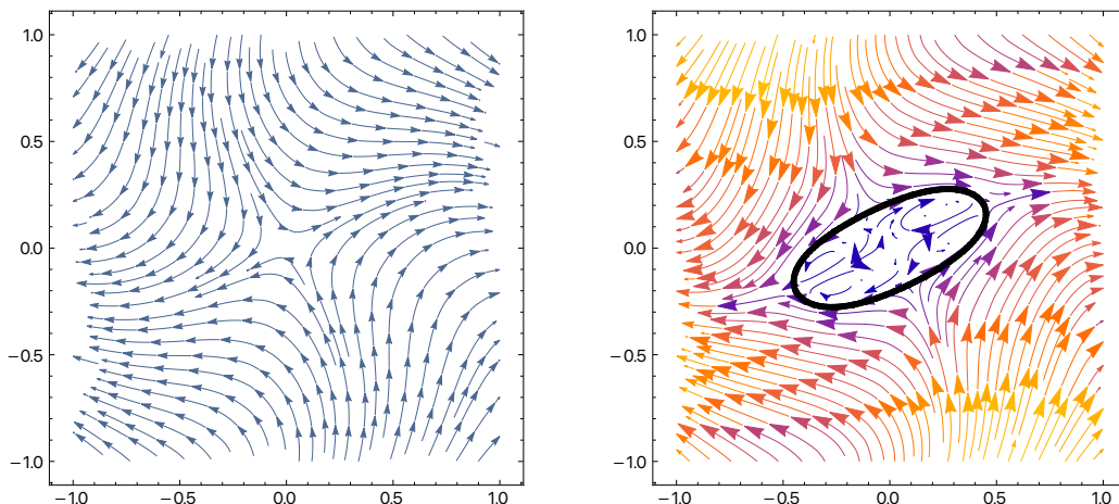
(a) Streamlines for the perturbed velocity field (3.27).
