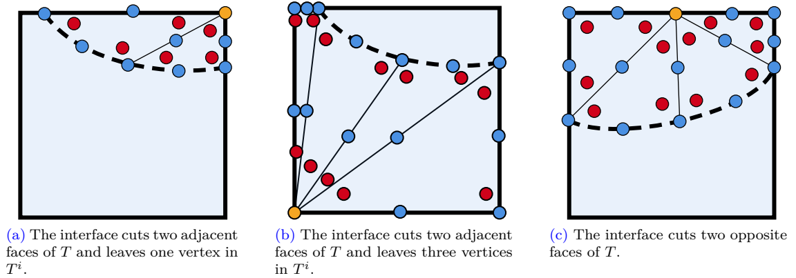
Figure 2.5: Example of cut cells T \in \mathcal{T}^\Gamma and of their decomposition into curved subtriangles. The subtriangulation is performed by connecting the interface points \{\mathbf{x}_m^{T,j}\}_{m \in \{0:2\}} , j \in \{1:2^n\} to a specific point (orange bullet, a vertex or an edge midpoint according to the cut configuration). The interface discretization parameters are (l = 2, n = 1) . The blue bullets, plus the orange bullet, are the physical points used for defining the mapping from the reference triangle into the physical one (quadratic mapping in the present example). Moreover, the red bullets represent the mapped integration Dunavant points for the second-order quadrature.
