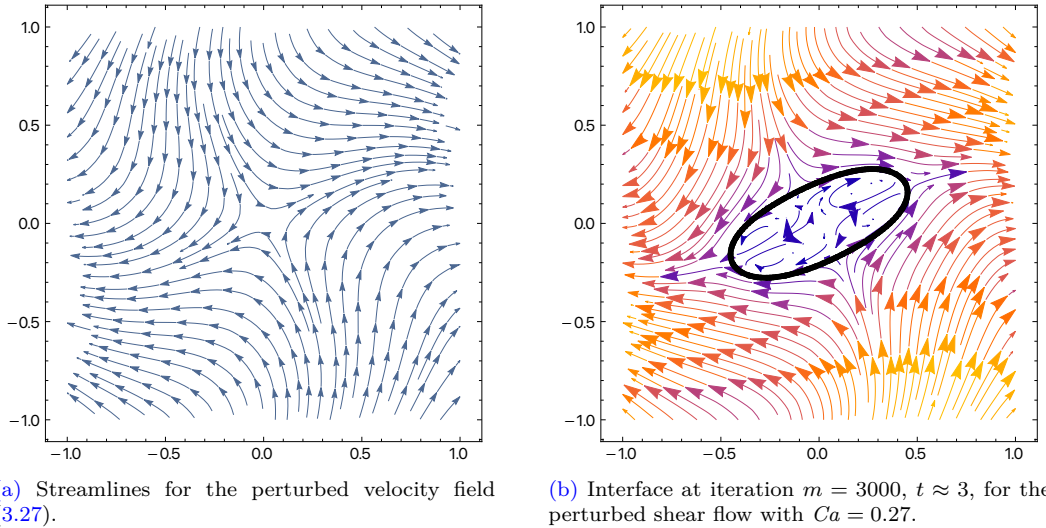
Figure 3.12: Streamlines for the test case with unknown interface. Figure 3.12a illustrates the velocity field (3.27) without the interface (i.e., \gamma = 0 ), Figure 3.12b includes the presence of the interface with Ca = 0.27 (i.e., \varepsilon = 0.26 , \gamma = 1 , \mu_2 = 1 , R_* = 1/3 ). The HHO polynomial order is k = 1 , and we employ q = 2 for the level-set approximation. The mesh is composed of 128 \times 128 square cells. The interface discretization parameters are ( l = 2 , n = 0 ).
