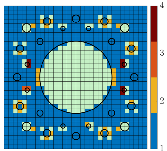
(b) Degree-adaptive approximation space ensuring 2 significant digits.
