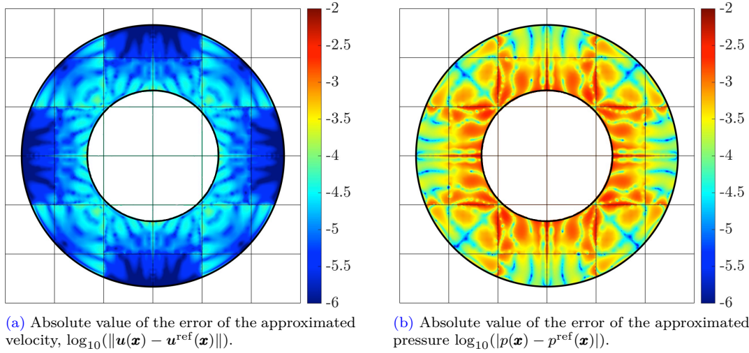
Figure 5.8: Taylor-Couette domain, zoom in (0.125, 0.875)^2 . Absolute value of the velocity and pressure errors for k = 4 . The mesh is composed of 8 \times 8 square elements. The element extension strategy is applied.
