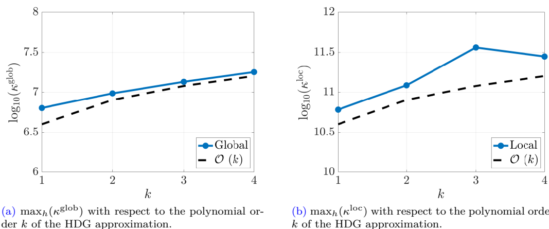
Figure 5.11: Taylor–Couette domain. In Figure 5.11a, the maximum value of the global condition number as a function of the polynomial order k for the meshes composed of 2 \times 2 , 4 \times 4 , 8 \times 8 , 16 \times 16 , and 32 \times 32 square elements. Similarly, in Figure 5.11b, the local condition number. The element extension strategy is applied.
