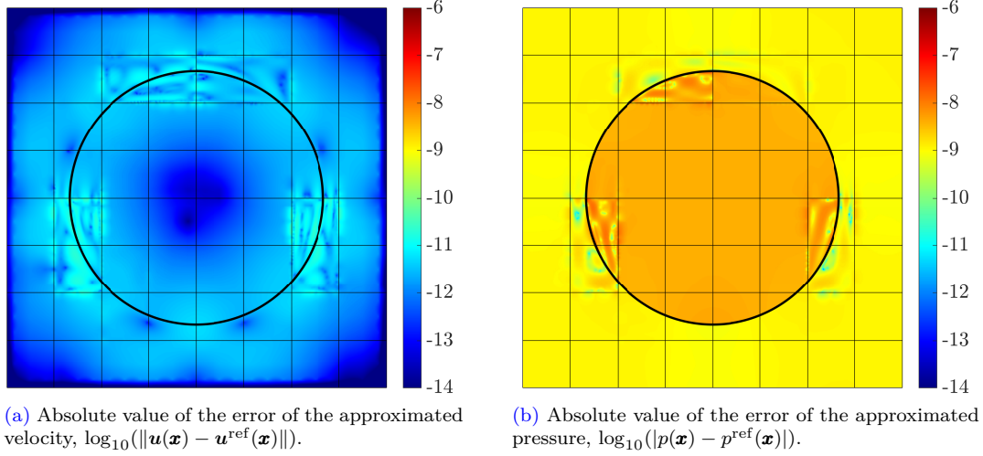
Figure 5.15: Equilibrium bubble. The mesh is composed of 8 \times 8 square elements. The basis order is k = 1 .
