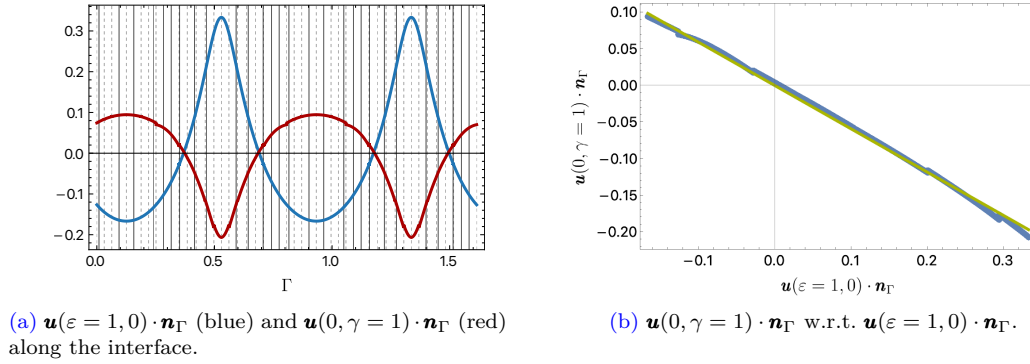
Figure 3.2: Figure 3.2a: normal velocities along the interface; the dashed vertical lines in the background represent the intersections between the interface and the cell faces, whereas the solid lines represent the intersections between the interface and the erased inner faces of the agglomerated cells. Figure 3.2b: \mathbf{u}(0, \gamma = 1) \cdot \mathbf{n}_\Gamma versus \mathbf{u}(\varepsilon = 1, 0) \cdot \mathbf{n}_\Gamma (blue bullets); the green line represents the linear regression curve with slope -m_{\text{eq}} \approx 0.590 . Elliptic interface with D = 1/3 and \mu_1 = \mu_2 = 1 . The velocity fields \mathbf{u}(\varepsilon = 1, 0) and \mathbf{u}(0, \gamma = 1) are computed in the domain \Omega = (-2, 2)^2 discretized by a mesh composed of 128 \times 128 square cells. We employ the unfitted HHO discretization with polynomial order k = 1 .
