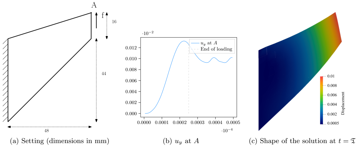
Figure 6.22: Cook's membrane, steel, linear isotropic hardening - Setting, displacement of point A and 2D solution at \mathfrak{T} , HHO with polynomial order k = 2 mixed-order setting, h = 0.05\text{m} .
