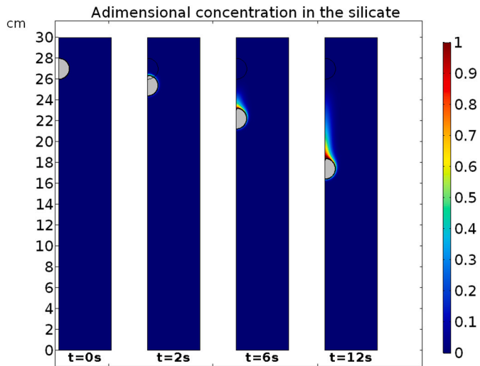
Fig. 6. Evolution of adimensional concentration of the siderophile element in the silicate, for a partition coefficient D^{met/sil} = 1 . For clarity purposes the metal is shown by the grey area surrounded by a black line. The black line is the boundary between metal and silicate and defines the surface where the exchange reaction happens. The adimensional concentration is given by the following formula given in Eq. (9). In this case X_{sil}^0 = 10^{-5} , X_{met}^0 = 0.2 and D^{met/sil} = 1 , and the chemical Peclet number is Pe \sim 800 .
