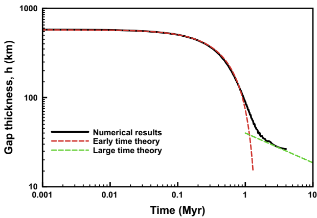
Fig. 6. Evolution of the gap thickness between the merging core and the CMB with R_{imp} = 600 km (i.e. R_{Fe} = R_{imp}/2 = 300 km). Theoretical evolutions for early times from Eq. (15) and late times from Eq. (17) are shown with red and green dashed lines respectively. From this model, we obtain a coalescence time, t_c = 1.55 Myr and a_2 \sim 1.3 \times 10^9 m s ^{1/3} . (For interpretation of the references to color in this figure legend, the reader is referred to the web version of this article.)
