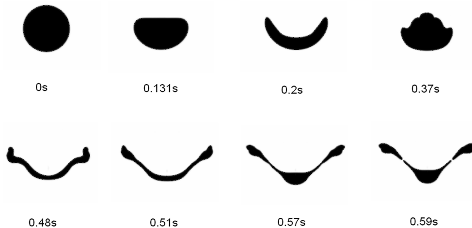
Fig. 7. Deformation and rim shear breakup of an iron drop within a magma ocean. In this model, Re = 92.4 , We = 20.3 , R_\mu = 100 (simulation #22 in Table 2).
