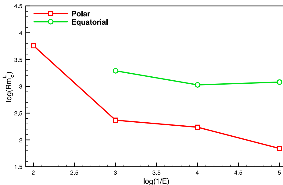
Figure 13. Local magnetic Reynolds number Rm_c^L as a function of E^{-1} . Rm_c^L is obtained by combining the results for Rm_c from Figures 8 and 9 (choosing the most favorable Ro value for each value of E ) and the fits for h from Figure 5.
