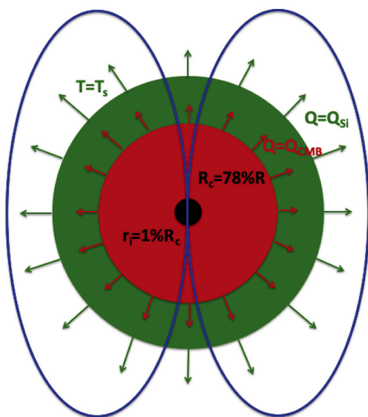
Fig. 10. Schematic representation of the geometry and of the heat flows computed in our model.
