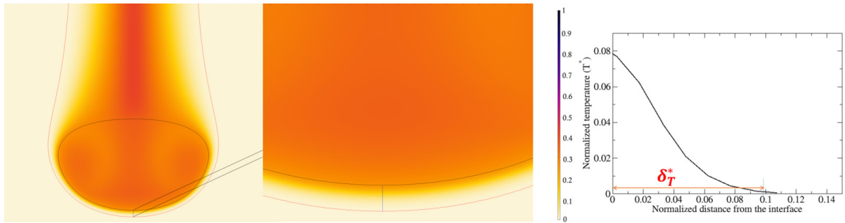
FIG. 8. Left: Temperature anomaly (color scale) and contour of the thermal boundary layer (red line) around the drop (black line) for our reference simulation no. 4 in Table II at time t^* = 0.067 . Middle: zoom at the drop front. Right: Temperature profile of the thermal boundary layer in front of the drop and determination of the local boundary layer thickness.
