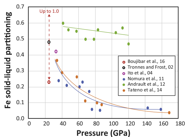
Fig. 8. Change in Fe partitioning ( D_{\text{Fe}}^{\text{Bg/melt}} ) between the Bg and a coexisting melt. Starting materials for LH-DAC experiments were olivine (blue, (Nomura et al., 2011)), chondritic-type mantle (green, (Andraut et al., 2012)) and peridotite (red, (Tateno et al., 2014)). Open circles correspond to previous multi-anvil experiments (Boujibar et al., 2016; Ito et al., 2004; Tronnes and Frost, 2002). The red arrow corresponds to the range of D_{\text{Fe}}^{\text{Bg/melt}} measured in a same study at varying F values.
