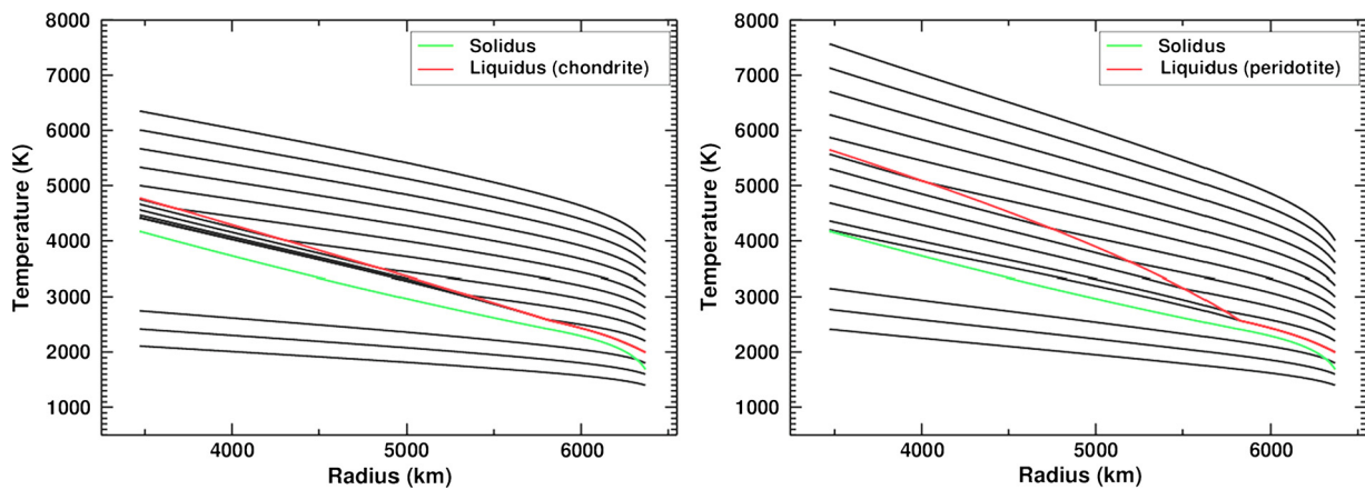
Fig. 1. Adiabats (with T_p ranging between 1400 and 4000 K) computed for the A-chondritic model (left) and the F-peridotitic model (right). The corresponding solidus and liquidus are represented in green and red respectively. (For interpretation of the references to color in this figure legend, the reader is referred to the web version of this article.)
