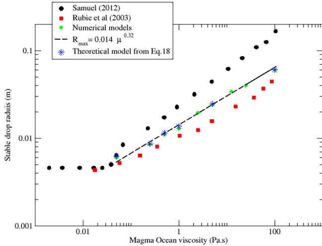
Fig. 14. Stable drop radius as a function of plausible magma ocean viscosities. The green diamonds present our numerical results, the red squares correspond to the results of Rubie et al. (2003), the black circles display the results of Samuel (2012), the blue stars correspond the analytical results of the Eq. (18) and the black dash line presents the scaling law proposed by this study. (For interpretation of the references to colour in this figure legend, the reader is referred to the web version of this article.)
