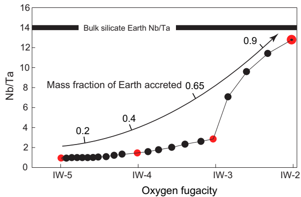
Fig. 3. Evolution of the Earth's mantle Nb/Ta ratio during the planet growth as a function of oxygen fugacity (after Cartier et al., 2014). The model considers the accumulation of impactors, starting with reduced and small-sized bodies, followed by less reduced and larger objects (Rubie et al., 2011). This accretion model also considers the degree of mixing (core – mantle equilibration) after each impact. The first stages are characterized by very low Nb/Ta ratios, due to massive core uptake. The last bodies accreted are more oxidized and their metallic parts do not fully equilibrate with the mantle, yielding to an increase of the Nb/Ta ratio, up to the current estimated value of 14. The arrow indicates the corresponding mass fraction accumulated as accretion progresses.
