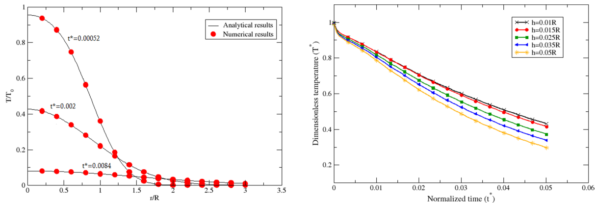
FIG. 2. Left: Comparison of our numerical results with the analytical results in Ref. [41] for the radial profile of the normalized temperature anomaly for a nondeformable and immobile drop. Right: Comparison of the time evolution of the normalized mean temperature anomaly determined with different mesh sizes for a deformable and mobile drop (simulation no. 4 in Table II).
