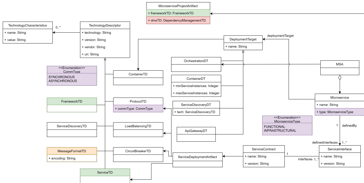
Figure 5.11: MMM's Operation viewpoint based on [RSSZ18]).
