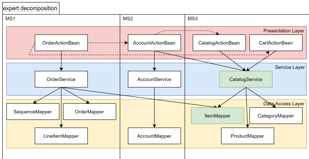
Figure 3.10: Expert decomposition of JPetStore.
