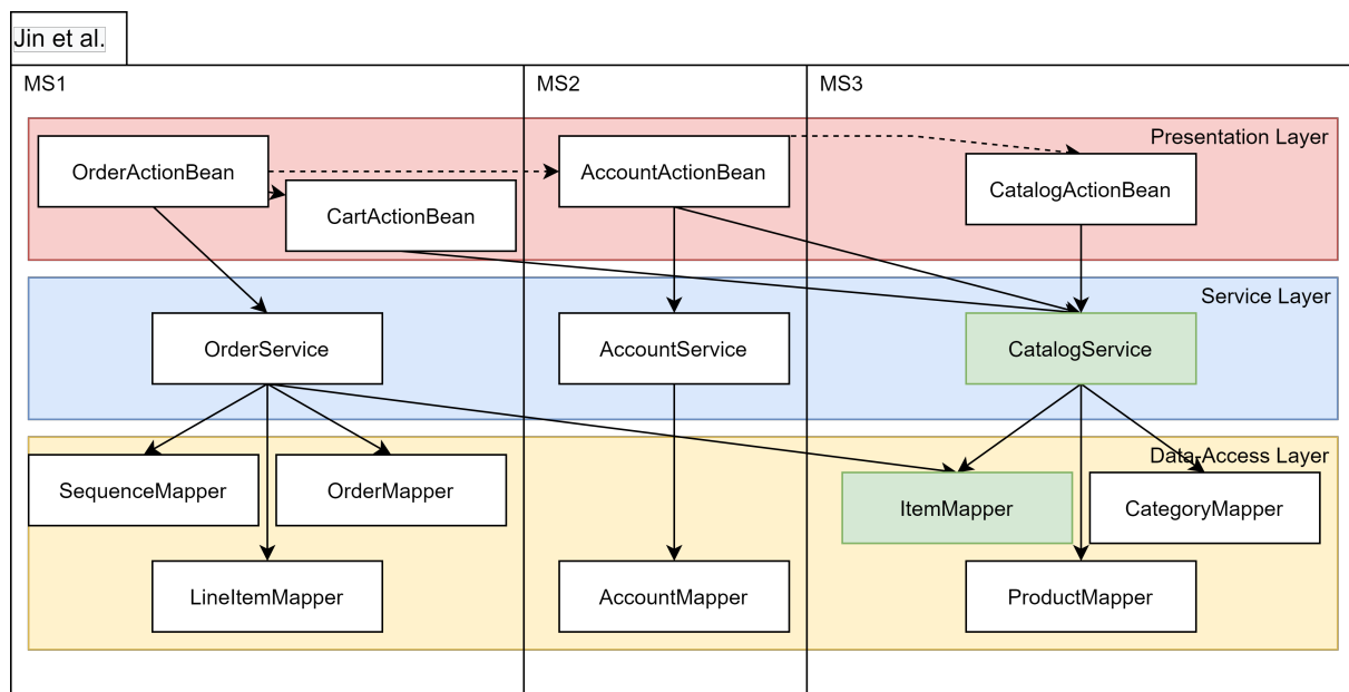
Figure 3.11: Decomposition of JPetStore proposed by [JLZ + 18]
