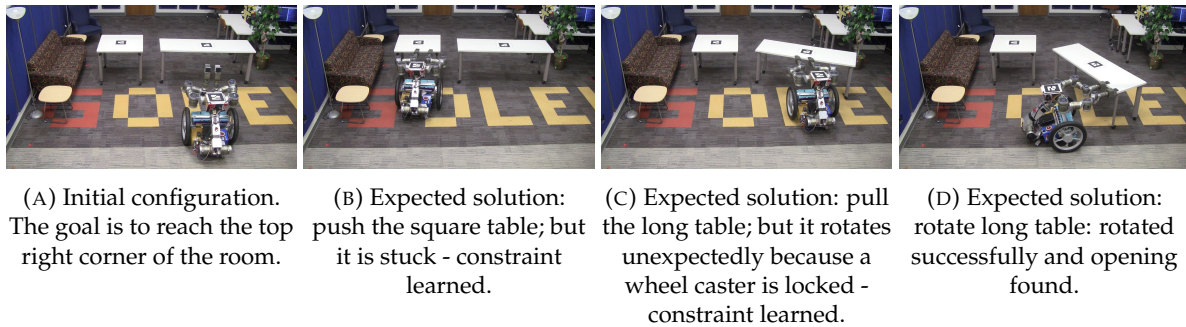
FIGURE II.16: Example NAMO problem resolution by Scholz et al.'s kinodynamic & decision theoretic algorithm [11], in a real-world setting. The robot has a differential drive base and two arms, totaling 17 Degrees of Freedom. Perception is provided by six overhead cameras tracking AR-tags[62].
