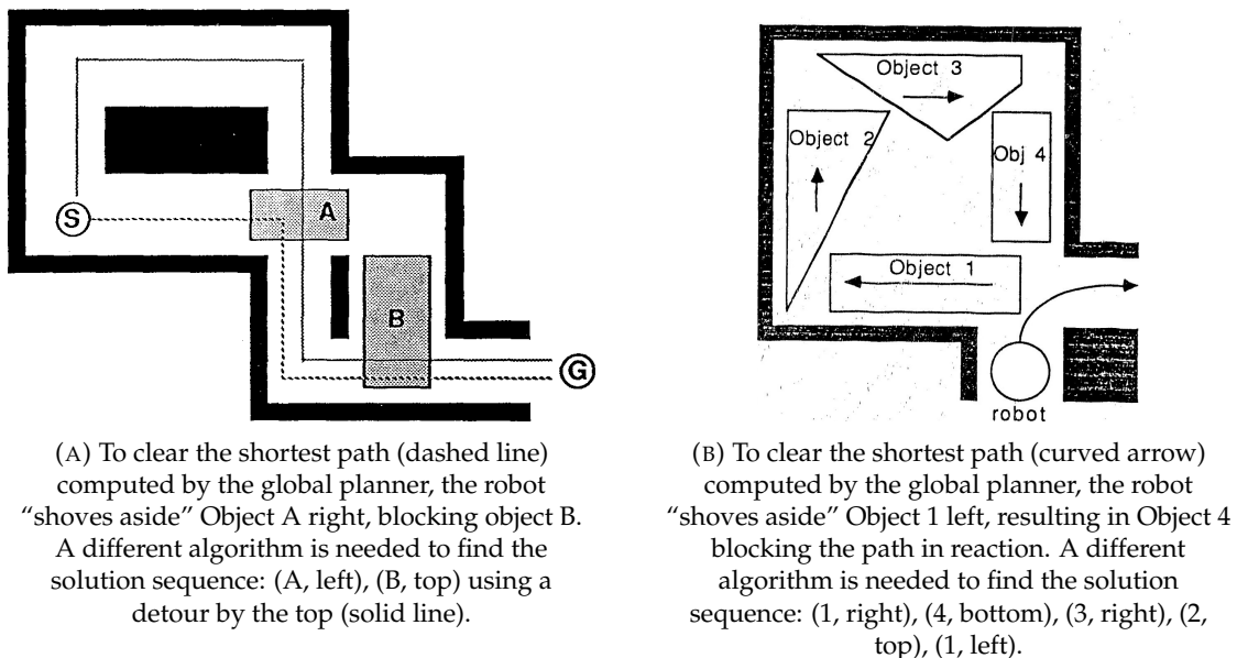
FIGURE II.4: Unsolvability cases for Chen&Hwang's algorithm [1].
