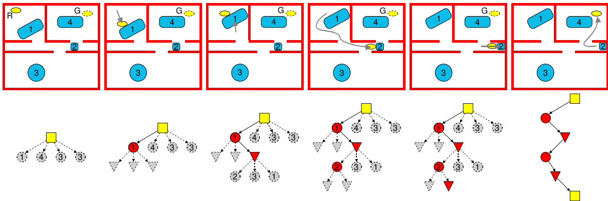
FIGURE II.9: Example L_1 NAMO problem solved by Nieuwenhuis et al.’s algorithm [4]. From left to right, the vignettes depict the initial world state, then the alternating “grasp”/“manipulate” sequence for obstacles 1 then 2, before a direct navigation path to the goal can be found in the last vignette. Under each vignette is the “action tree”, where round nodes are “grasp” nodes with the associated obstacle’s number, and triangle nodes are “manipulate” nodes. The yellow squares represent the initial and goal states, and the red nodes are the selected nodes branch represented in the vignettes.
