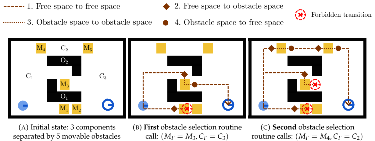
FIGURE III.19: Example NAMO scenario showcasing the obstacle selection routine. The four types of allowed transitions are shown as brown lines and markers. For the sake of simplicity, only axis-aligned translations are allowed and only the relevant branches of the A^* search are shown instead of the full tree.
