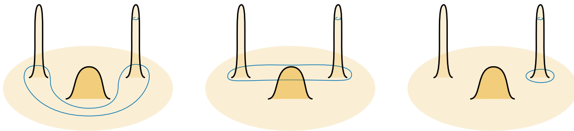
FIGURE 5.5 – An optimal homotopy between the two blue curves picture on the left escapes the annulus that they cobound, and is thus in particular not monotone. Indeed, in order to minimize the maximal length of the curves, it first climbs over the small bump before climbing over the left peak.
