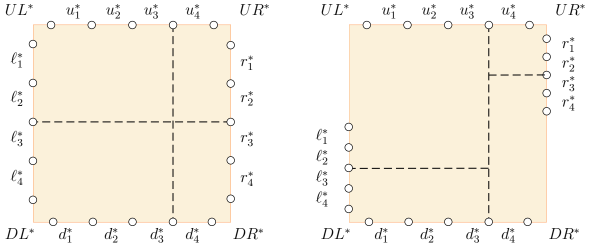
FIGURE 4.4 – Left: a dual multiway cut in a dual cross gadget. Right: A more realistic representation of an actual optimal multiway cut in a dual cross gadget.
