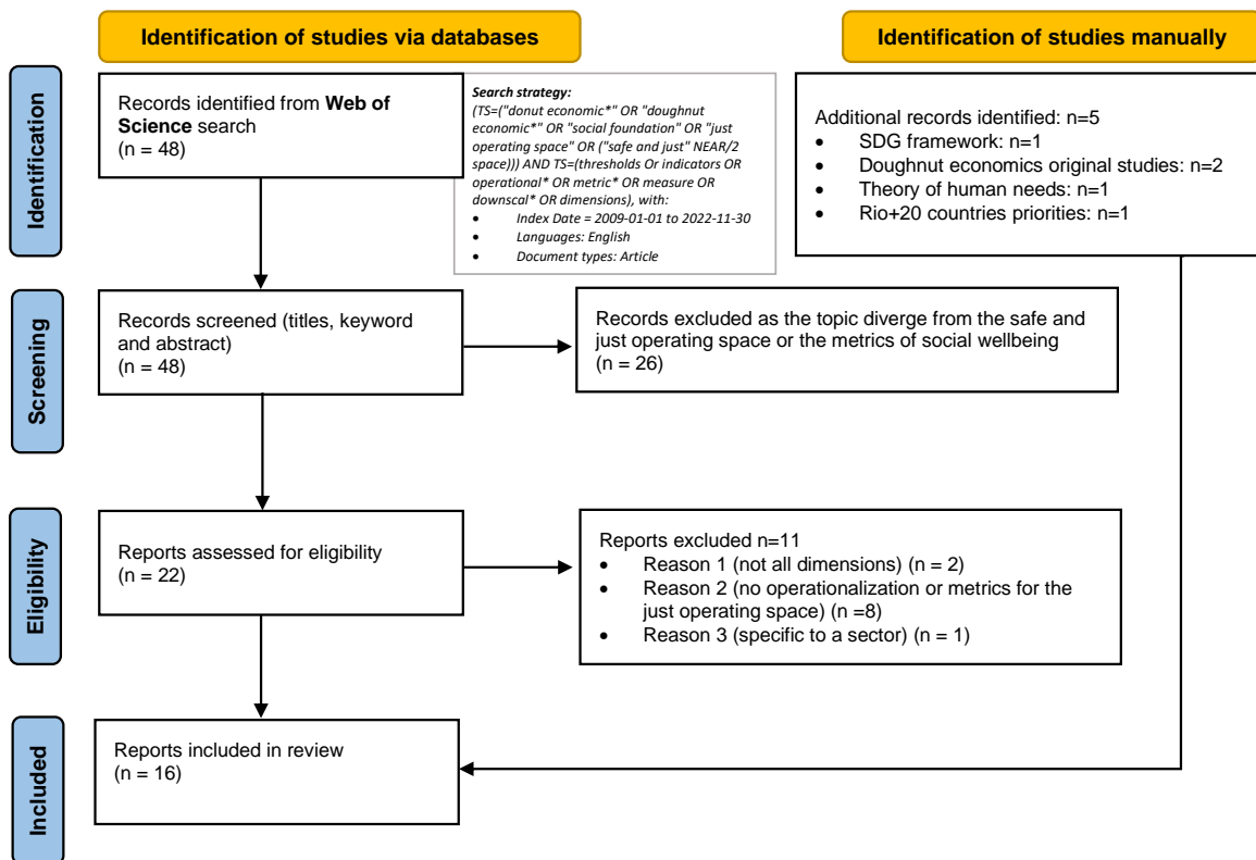
Figure A.3: Search strategy for the literature review on studies operationalizing the Safe and Just Operating Space
