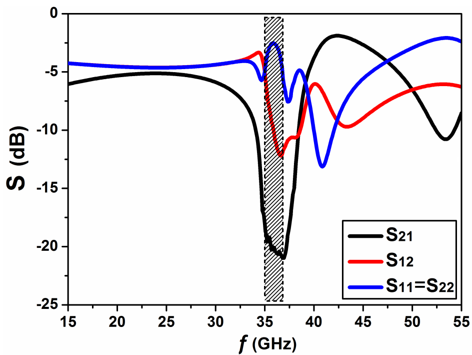
Figure 4.19: Simulated S -parameters of the coplanar circulator.
