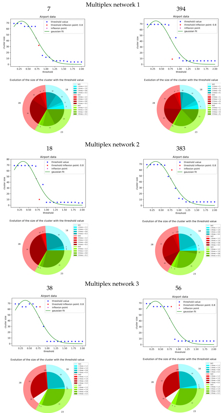
Fig. S1. Each pair of two charts represent the evolution of the community's final size depending on the threshold value. The top chart represents the evolution of the final community size depending on the threshold value from 0.1 to 2.0. The green curve represents the Gaussian fit with its inflection (pink point) that gives us the value for which we observe an abrupt behavior, we expect to observe a better threshold value around this value. The red point represents the nearest experimental point (here always associated with a threshold value equal to 0.8). The bottom chart represents the evolution of the community size for different threshold values represented by the shades of colors. The colors represent the nodes of a specific multiplex network, blue for the first multiplex network (French multiplex network), red for the second multiplex network (British multiplex network), and green for the third multiplex network (German multiplex network). The external part of the pie chart gives the total number of nodes in each multiplex network, and the inner part gives the number of nodes in the final community depending on the threshold value and concerning their multiplex network of origin. The left figures represent the highest degree node selected as a seed in each multiplex network (#7, #18, #38), and the right figures represent the lowest degree node selected as a seed in each multiplex network (#394, #383, #56).
