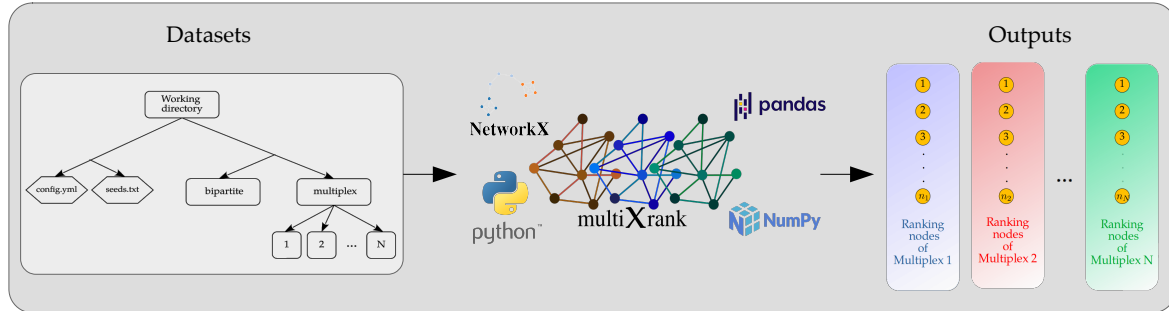
Fig. S3. Workflow of the MultiXrank Python package. The network and the parameter datasets need to be ordered as in the tree file in the left panel. This tree file is used by MultiXrank to run RWR on the multilayer network defined in the bipartite and multiplex folders, with the parameters given in the config and seeds files. MultiXrank returns the output scores in an output folder, as shown in the right panel. A Conda environment is available on GitHub ( https://github.com/anthbapt/multixrank ) to install all dependencies needed by MultiXrank.
