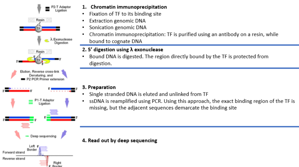
Figure 6 : ChIP-exo datasets : ChIP-exo is a technique for determining transcription factor (TF) binding sites with near nucleotide precision. Different steps of the procedure are shown.
