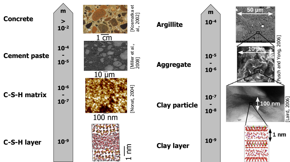
Figure 1.1 – Multiscale structure of (left) concrete and (right) argillite. C-S-H stands for calcium silicate hydrates. Subfigures are adapted from Kosmatka et al. (2002); Miller et al. (2008); Nonat (2004); Pusch and Yong (2006); Laird (2006).
