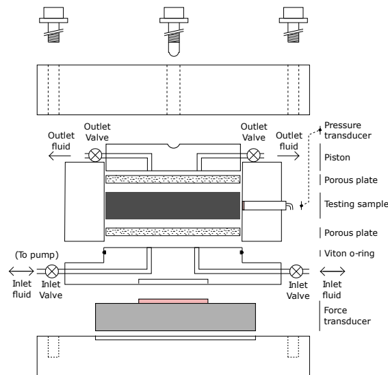
Figure 4.4 – Isochoric cell used for the measurement of crystallization-induced pressures in ground and recompacted cement paste samples.
