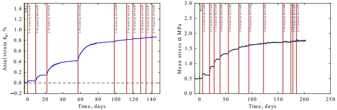
Figure 4.5 – Typical results obtained upon flushing of ground and recompacted cement paste samples with sodium sulfate solution: (left) axial strain measured during an experiment performed in an oedometric cell, and (right) volume stress measured during an experiment performed in an isochoric cell. Each vertical red or green line represents a flushing of the sample with the sodium sulfate solution or with water, respectively. Figure adapted from Bui (2016) .
