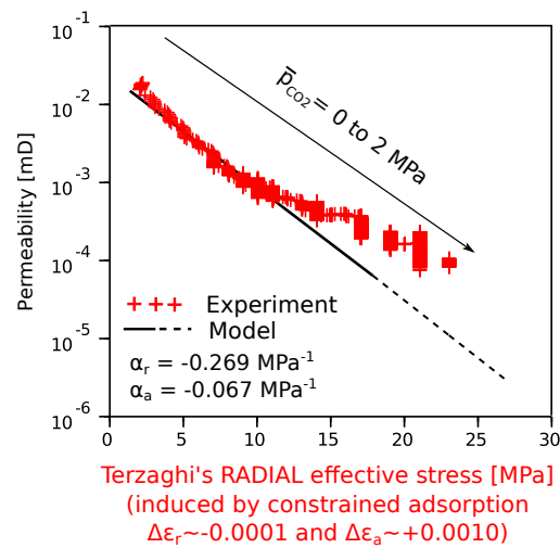
Figure 2.11 – CO 2 permeability evolution of coal core subjected to constrained adsorption under near constant-volume conditions. The specimen is subjected to increasing compressive stresses as a result of CO 2 injection and constrained swelling. Ensuing stresses lower measured permeability up to 100 times. The dashed line indicates values of permeability extrapolated out from the experimental fitting range. Time goes from top left to bottom right. Figure from Espinoza et al. (2014) .
