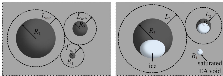
Figure 4.1 – Schematic describing the distribution of entrained air voids and the shell of cement paste surrounding them. (left) Before the first freeze-thaw cycle, the thickness of the shell of cement paste from which water flows toward the air void upon freezing is assumed to be the same for all air voids. (right) After a given number of freeze-thaw cycles, air voids have absorbed some water, to such extent that the smallest air voids are now filled and all water in the cement paste around those air voids must flow to other air voids, resulting in an increasing shell thickness around those latter air voids. Figures from Mayercsik et al. (2016) .
