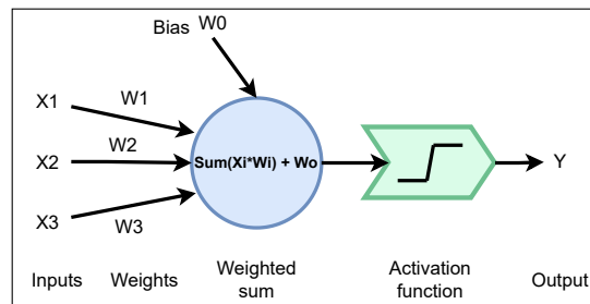
Figure 1.10 – An example of an artificial neuron.
