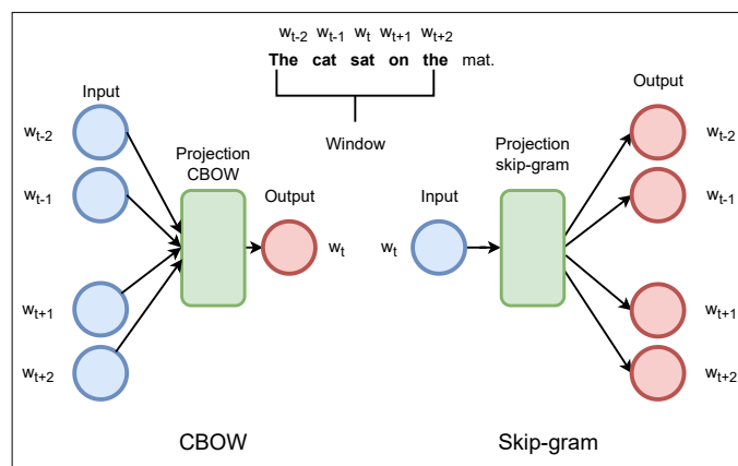
Figure 1.18 – Word2vec architecture (CBOW and Skip-gram).
