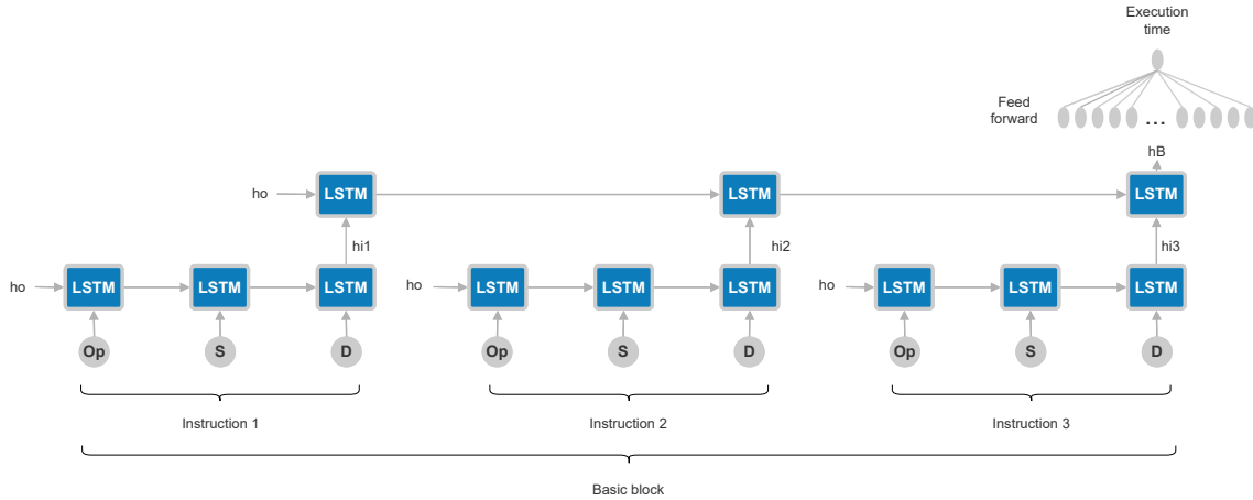
Figure 1.20 – ITHEMAL architecture.
