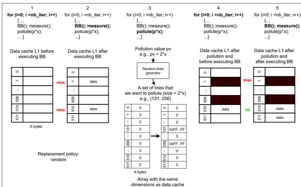
Figure 2.3 – An example illustrating data cache pollution simulation on a basic block in 5 steps. The process targets a data cache that employs a random replacement policy.
