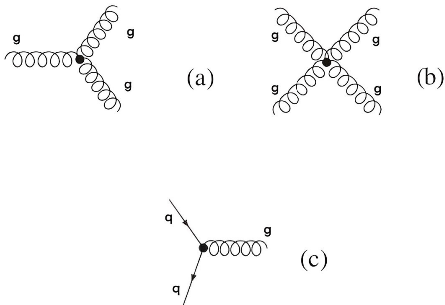
Figure 11 – Representation of the potential interaction vertices within QCD are depicted as follows: (a) represents a three-gluon vertex, (b) represents a four-gluon vertex, and (c) represents a quark-gluon interaction. [12]
