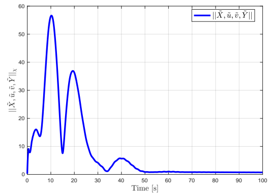
(b) Evolution of the \chi -norm of the error state (\tilde{X}, \tilde{u}, \tilde{v}, \tilde{Y}) .
