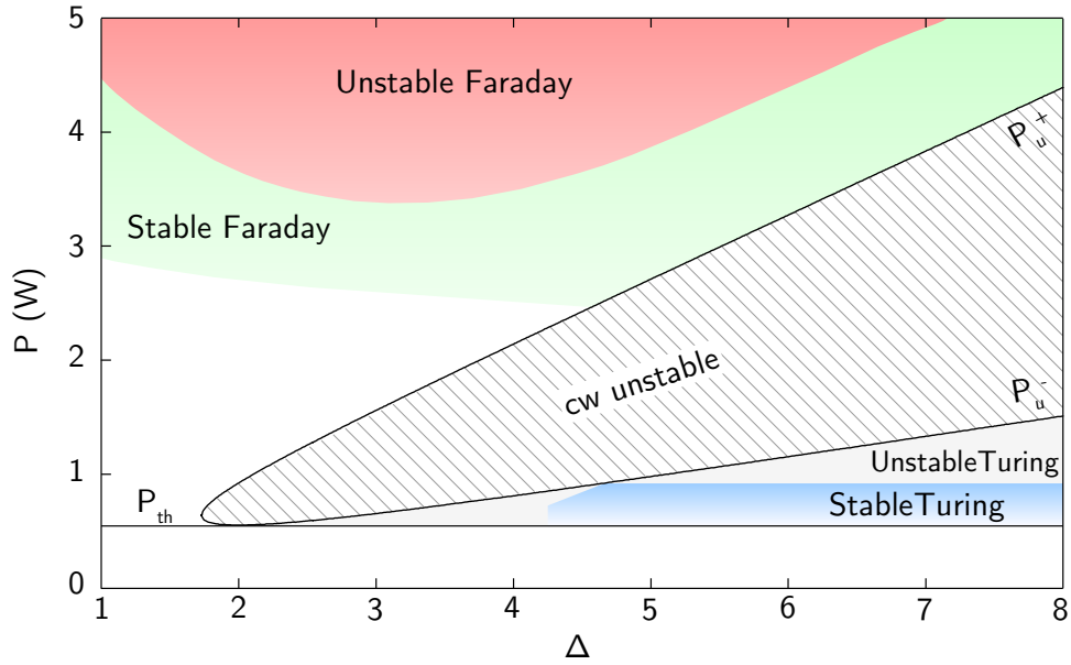
Figure 4.3 – Instability chart of the different domains of instability in our longitudinally modulated cavity.
