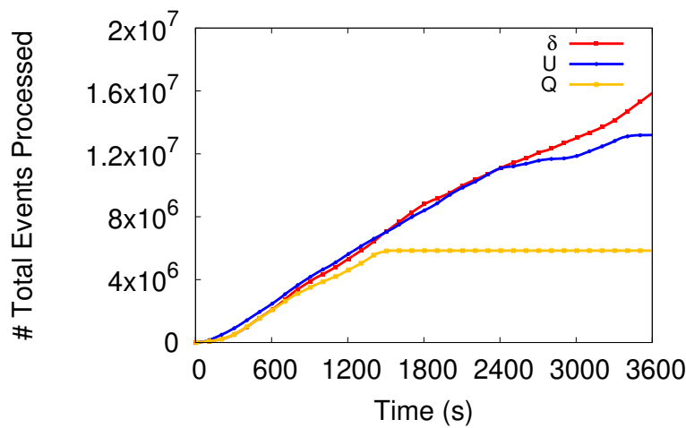
Fig. 5.19: Total number of processed events of \delta , U , and Q .
