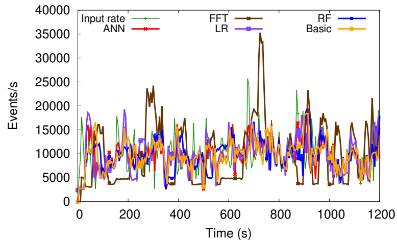
Fig. 5.32: Throughput of PA-SPS using Log dataset.
