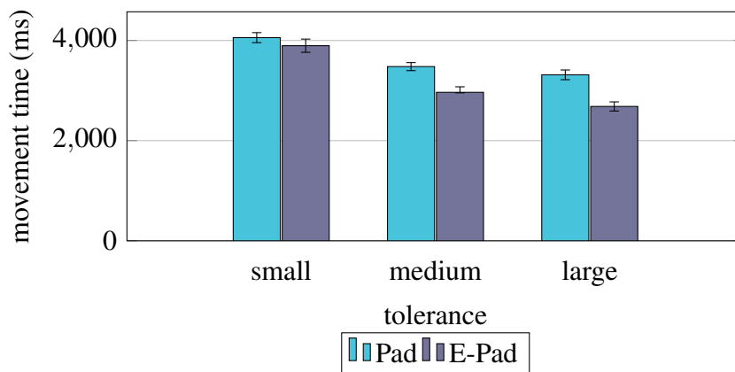
Figure 5.7: Effect of tolerance on movement time
