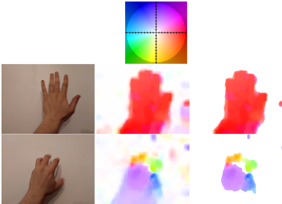
Figure 3.1: Color representation of the optical flow. (Top) Color space: hue indicates direction, saturation indicates amplitude. (Middle) Swipe right gesture, calculated flow, filtered flow. (Bottom) Grasp gesture, estimated flow, filtered flow
