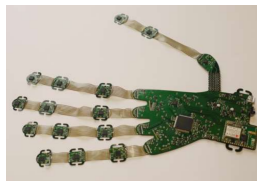
Figure 2.2: The IMU Smart Glove rev 2, extracted from [134]
