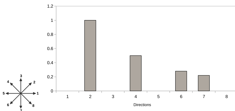
Figure 3.2: (left) 8 directions (right) Histogram of the grasp gesture
