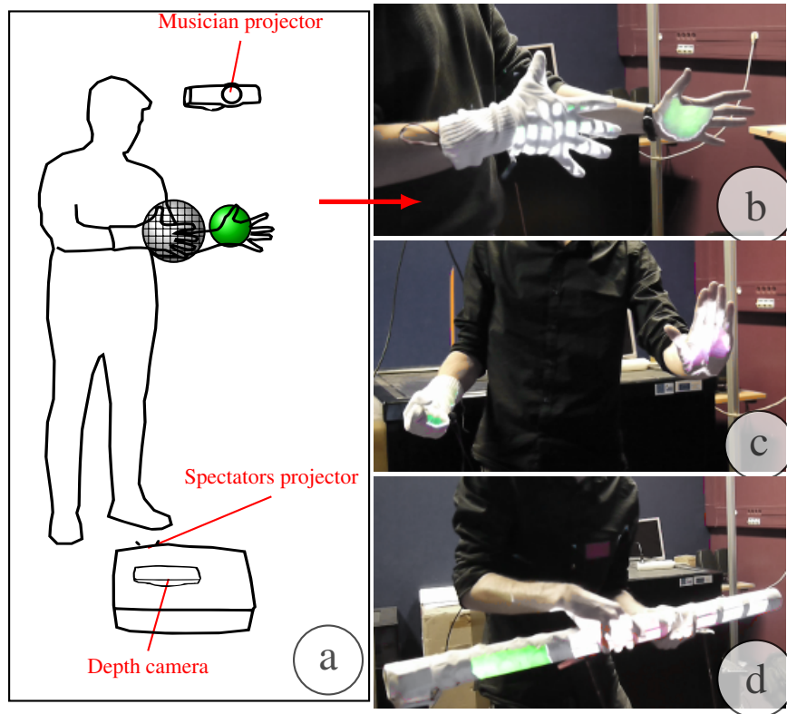
Figure 4.6: (a) Revgest in a setup with two projectors and one depth camera for public performance. The top projector is placed behind the musician and allows for feedback visible only to them. A virtual sphere is attached to the musician's right hand and provides feedback on finger movements sensed by a glove, another sphere in green controls a delay effect. (b) The resulting augmented gestural instrument. (c) Another glove based gestural instrument. (d) Augmentation of a handheld instrument.
