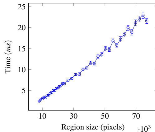
Figure 4.5: Computation time of the features vs region size
