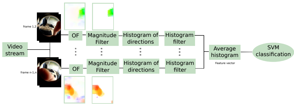
Figure 3.5: Pipeline of our method
