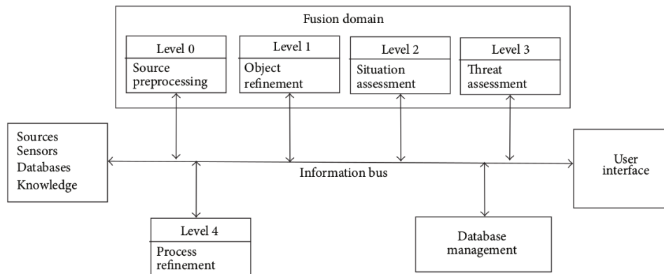
Figure 2.1: JDL fusion model. Extracted from [40]
