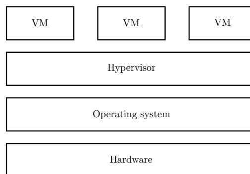
Figure 1.7: Type 2 hypervisor
