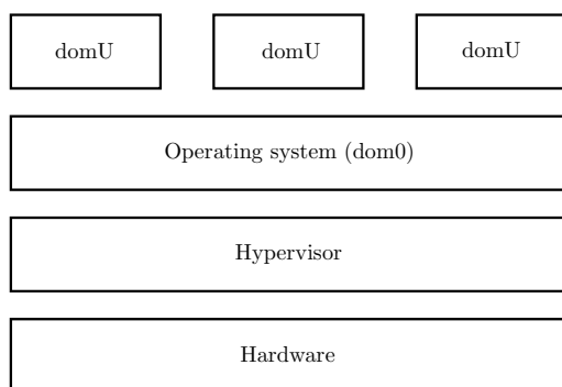
Figure 1.6: Type 1 hypervisor
