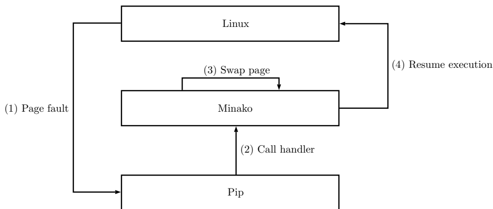
Figure 4.5: Page swapping in Minako, part 1
