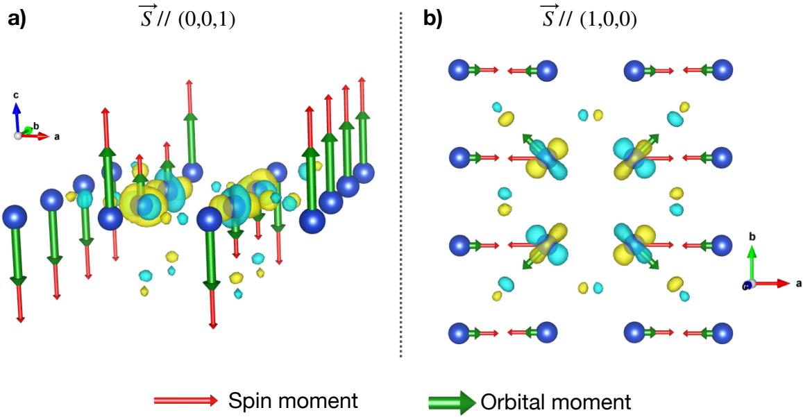
Figure 5.6: Schematic representation of the orbital momentum orientation for two different magnetization axis: (a) (0,0,1), (b) (1,0,0). The length of the vectors illustrates the variation of the absolute value of the moments.
