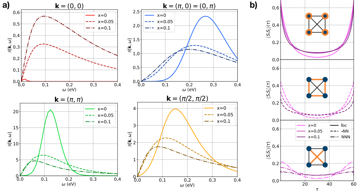
Figure 3.14: (a) DSSF at different \mathbf{k} points as a function of doping ( x = 0, x = 0.05, x = 0.1 ), all calculated at \beta = 60\text{eV}^{-1} . The same error estimate ( 10^{-2} ) was used for all spectra to perform the analytic continuation. (b) Local, NN , and NNN cluster spin-spin correlation functions as a function of imaginary time, for different dopings and calculated at \beta = 60\text{eV}^{-1} . Note that the NN component has been multiplied by -1.
