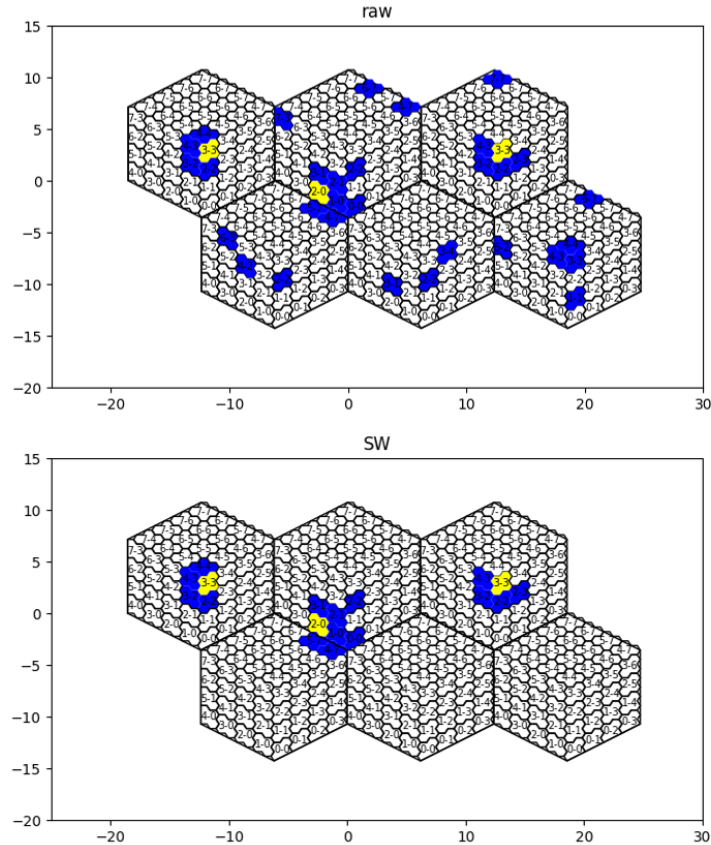
Figure 2.9: Example of 2D topological clustering with distance constraints [18]. The seed trigger cells are drawn in yellow while trigger cells above the clustering threshold but below the seed threshold are drawn in blue. All trigger cells are shown in the upper plot, while clustered trigger cells are shown in the bottom plot.
