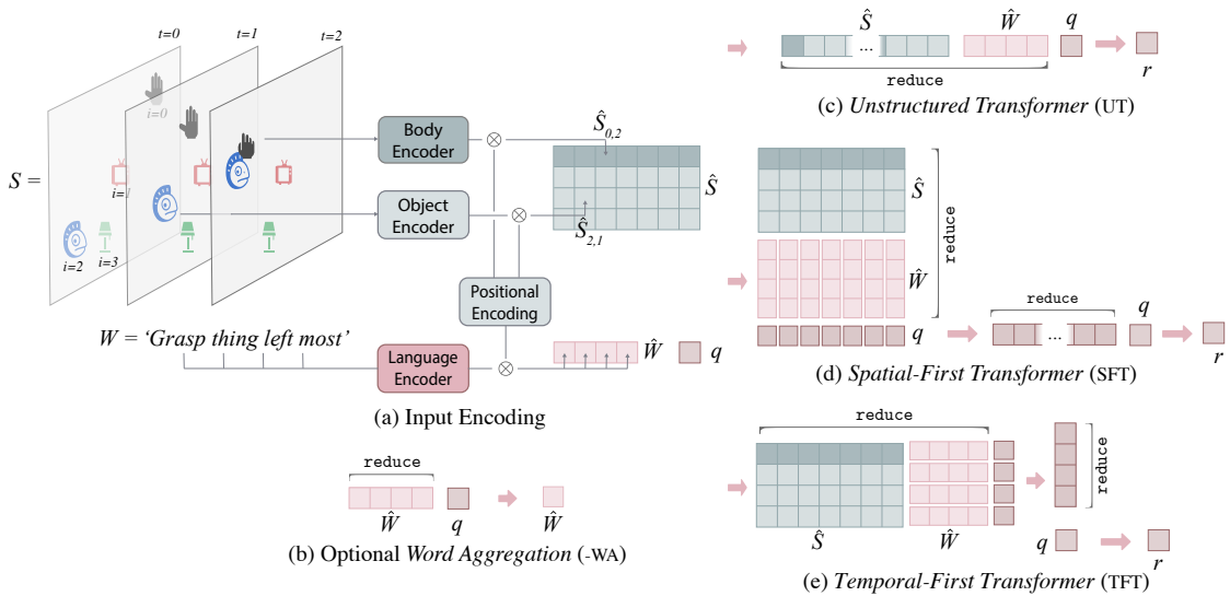
Figure 3.4: Visual summary of the architectures used. We show the details of UT, SFT and TFT respectively in sub (c), (d), (e), as well as a schematic illustration of the preprocessing phase (a) and the optional word-aggregation procedure (b).
