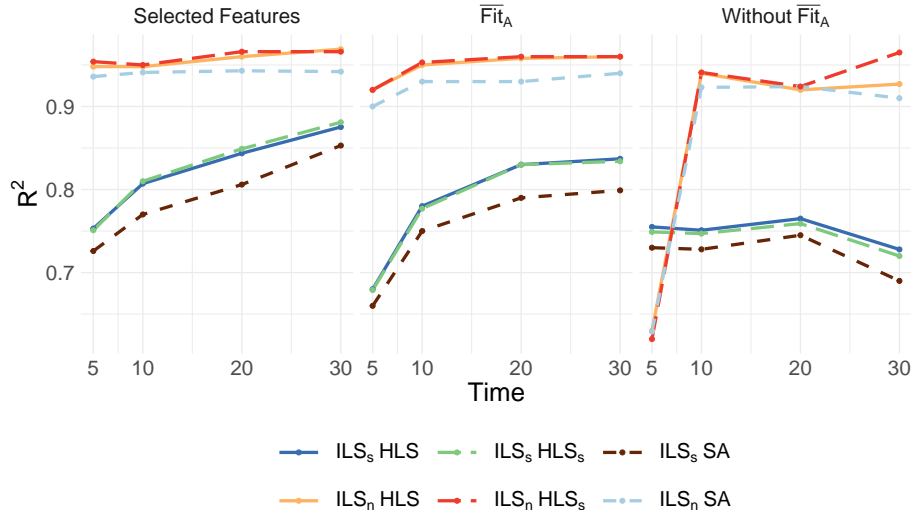
Figure 2.9: R^2 values for models, where each point represents a (sampler, solver) pair.
