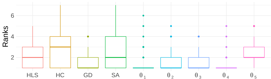
Figure 5.8: Value of Ranking by Method over all real-world Instances.
