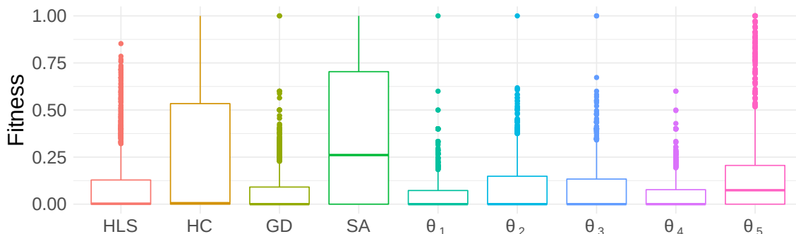
Figure 5.6: Distribution Fitness Scaled per configuration over New real-world instances.
