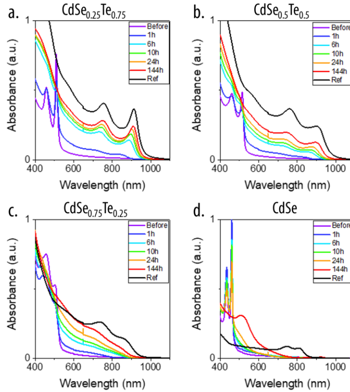
Figure 62: Cation exchange speed on CdSe_xTe_{1-x} with different alloys compositions. a-d. Absorption spectra of the solution according to the time during the CE of respectively CdSe_{0.25}Te_{0.75} (a), CdSe_{0.5}Te_{0.5} (b), CdSe_{0.75}Te_{0.25} (c), and CdSe (d) 3ML NPLs using exact same conditions. A black reference curve is added on all the graph to compare the optimized CE with the initial one on a similar amount of NPLs.
