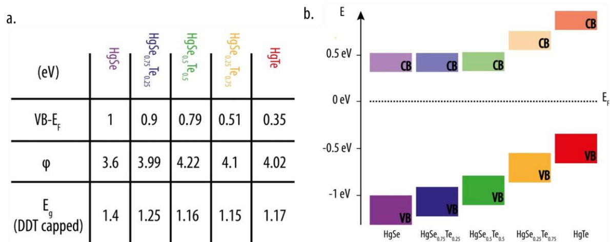
Figure 68: Band alignment establishment. a. Table summing up the energetical value extracted from valence band and work-function measurements, and optical measurements for all the alloy compositions. b. Plotted band diagram with Fermi level set at 0 eV according to the alloy's composition.
