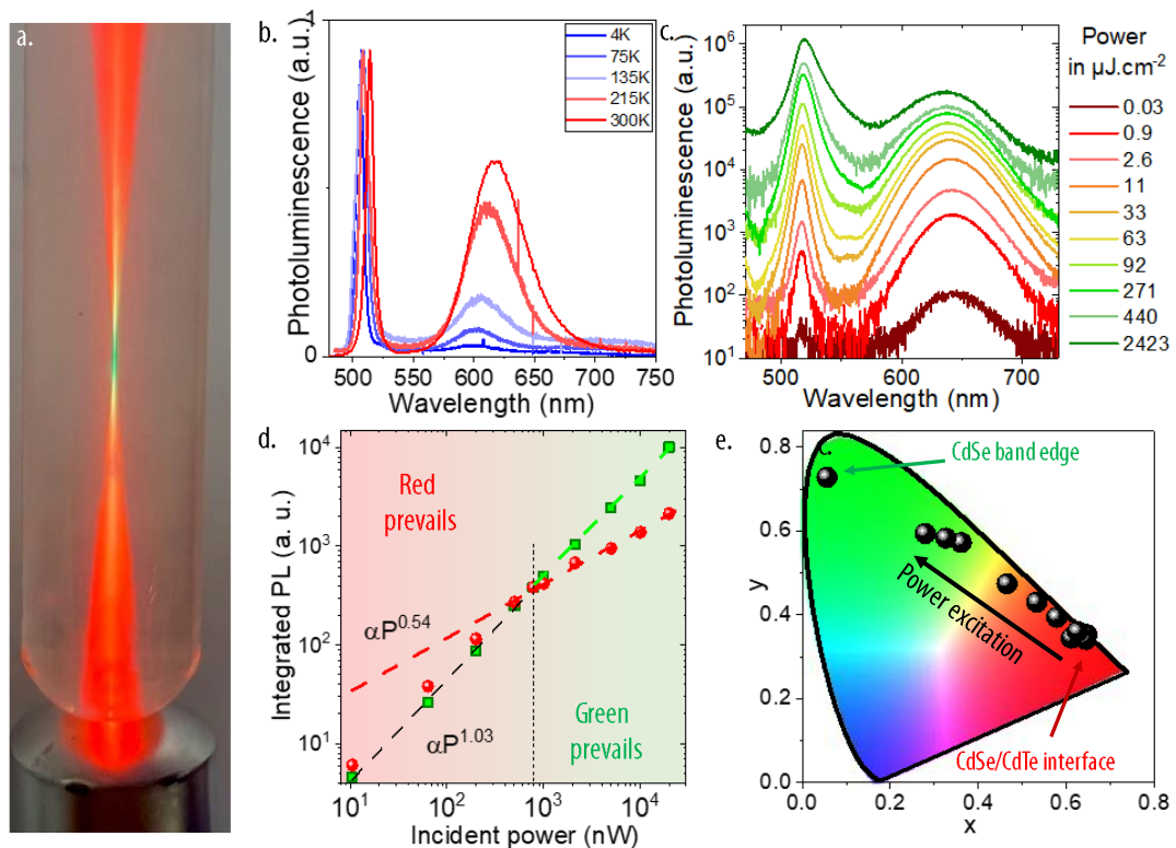
Figure 39: Power dependency of the green-to-red ratio. a. Picture of a heterostructure solution diluted inside a test tube. The excitation is provided by a 405 nm laser pointer and a filter is used to cut the excitation wavelengths. b. Evolution of the emission spectra according to the temperature. c. Evolution of the PL spectrum according to the incident power excitation. d. Integrated green and red features according to the incident excitation power. The dashed lines correspond to the linear fit of the two emissions before the saturation (black), to the linear fit of the red and green emissions after the saturation (resp. red and green). The prevailing features are underlines by the red and green font color. e. Localization of the emission spectra presented in c. inside the CIE color gamut. The green and red arrows are pinpointing the position of the two emissions taken separately. In all those experiments, the excitation have been conducted at 400 nm.
