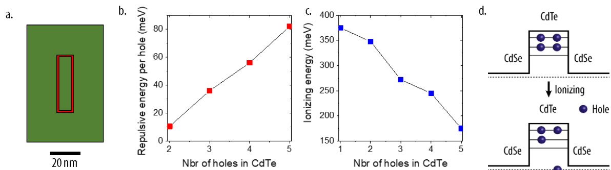
Figure 41: Coulomb blockade investigation. a. Sketch of the modeled NPLs. b-c. Evolution of the inter-hole repulsion energy (b) and ionizing energy (c) according to the number of holes injected inside the CdTe crown. d. Sketch of the ionizing process.
