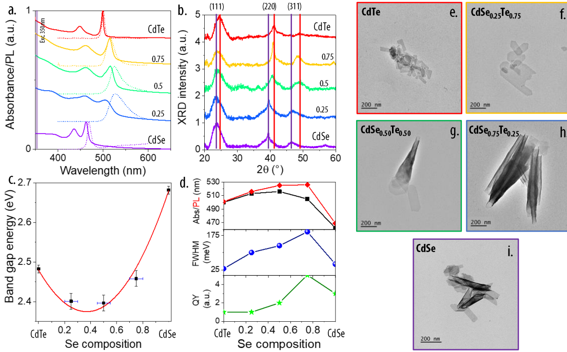
Figure 54: Sum up of the optical features of 3 ML CdSe x Te 1-x NPLs with 0 ≤ x ≤ 1. a. Absorption (plain) and emission (dots) spectra for 3 ML CdSe x Te 1-x NPLs. For clarity, the absorption and emission spectra have been shift by pairs of same composition. The excitation have been conducted at 350 nm. b. XRD diffractograms of 3 ML CdSe x Te 1-x NPLs. The diffraction peaks are labeled on top of the window, the red (resp. purple) dashed line corresponds to the position of the corresponding diffraction peak for CdTe (resp. CdSe). For clarity, the curves have been shifted. c. Band gap energy according to the composition is Se (x) in CdSe x Te 1-x 3ML NPLs. The red fitting curve unveils the bowing effect in these alloys. d. Maximum in absorption (in red) and emission (in black), full width at half maximum (in blue) and quantum yield (in green) of the 3ML CdSe x Te 1-x NPLs according to their composition in Se (x). e-i. TEM pictures of respectively CdTe, CdSe 0.25 Te 0.75 , CdSe 0.5 Te 0.50 , CdSe 0.75 Te 0.25 and CdSe 3ML NPLs.
