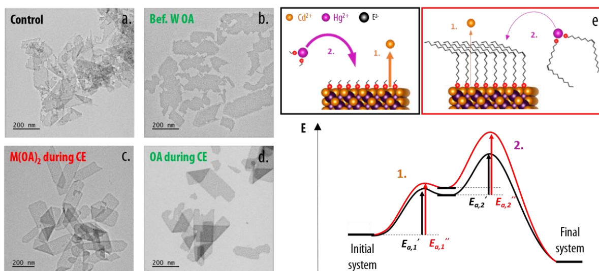
Figure 60: Influence of the addition of bulky ligands during the cation exchange. a-d. TEM pictures of HgSe 0.5 Te 0.5 after exchange using different conditions at RT in TCE: a. reference sample exchanged in TCE, b. same as a. but with addition of OA before the washing process, c. same as a. but adding few drops of Cd(OA) 2 (0.1 M in OA) before the exchange, d. same as a. but adding OA before the cation exchange. e. Sketch of the cation exchanged procedure seen as successive activations barriers. The small panel describes situations where small/bulky ligands are introduced before the cation exchange.
