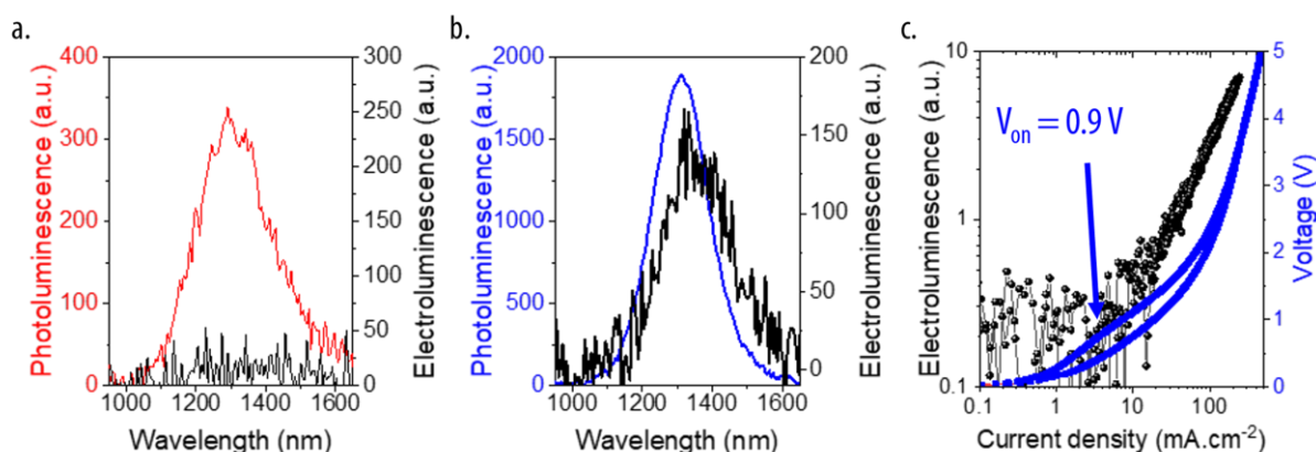
Figure 77: Electroluminescence comparison between treated and untreated LED. a. Photoluminescence (red, exc. 405 nm, and electroluminescence (black) of the LED stack based on untreated HgTe 3 ML NPLs. b. Photoluminescence (blue, exc. 405 nm)) and electroluminescence (black) of the LED stack based on treated HgTe 3 ML NPLs. c. Evolution of the electroluminescence (black) and imposed bias (blue) according to the current density going through the stack.
