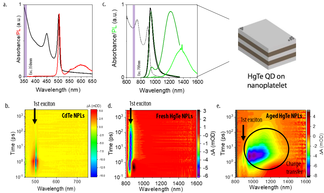
Figure 73: Aging of HgTe 3 ML NPLs. a. Absorption (black) and photoluminescence spectra (red, exc. 350 nm) of CdTe 3 ML NPLs. b. Transient absorption map of CdTe 3 ML NPLs (exc. 400 nm). c. Absorption spectrum (black dot line) and photoluminescence spectra (colored lines, exc. 700 nm) evolution of HgTe 3 ML NPLs according to the time. The sketch on the side is adapted from ref 190 and represents the HgTe 3 ML NPLs after aging and after the formation of small dots on it. d. Transient absorption map of freshly synthesized HgTe 3 ML NPLs (exc. 700 nm). e. Transient absorption map of aged HgTe 3 ML NPLs (exc. 700 nm).
