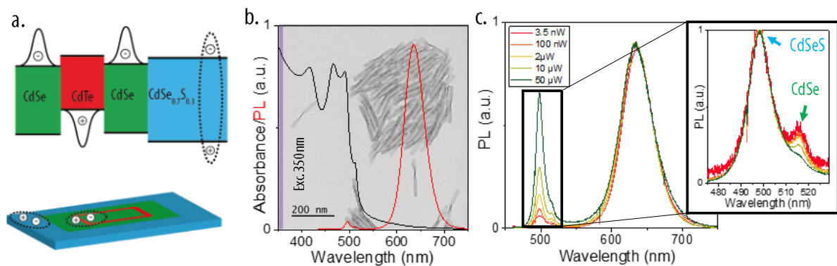
Figure 40: Tricolor emitting NPLs. a. Sketch and band alignment of the CdSe-CdTe-CdSe-CdS x Se 1-x heterostructure. b. Absorption (black) and PL (red) spectra of the CdSe-CdTe-CdSe-CdS x Se 1-x heterostructure. In the back font is introduced a corresponding TEM picture. The excitation has been conducted at 350 nm. c. PL spectra according to the incoming excitation fluence. The panel corresponds to a zoom on the 500 nm region. For clarity, the PL spectra have been normalized to the red emission. The excitation has been conducted at 400 nm.
