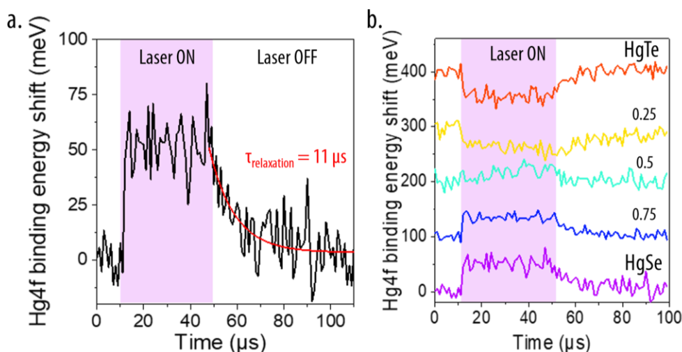
Figure 70: Unveiling charge carrier dynamics in \text{HgSe}_x\text{Te}_{1-x} 3ML NPLs. a. TRXPS spectrum of HgSe 3ML NPLs. The Hg4f core-level are shifting toward higher BE when under illumination. The 10 first \mu\text{s} before the rise have been reported at the end of the window to fully visualize the SPV relaxation. The red curve corresponds to the fitting of the SPV relaxation. b. Sum up of the TRXPS as a function of the alloy composition. The curves have been shifted for more clarity.
