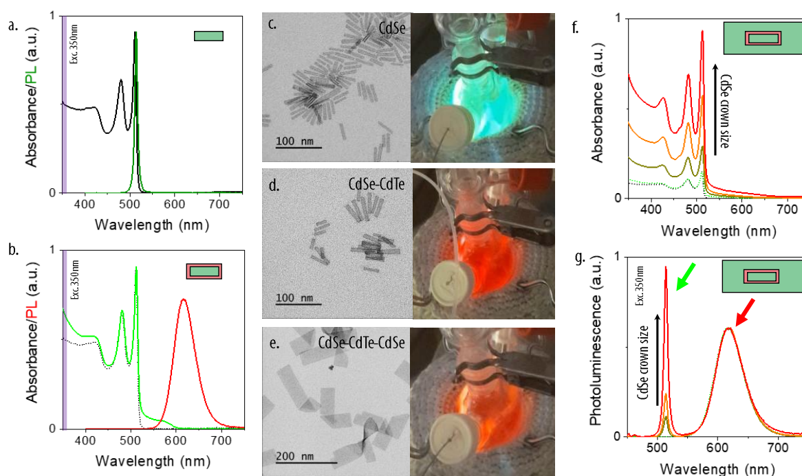
Figure 32: Synthesis of CdSe-CdTe-CdSe core-crown-crown heterostructure. a. Absorption (black) and emission (green) spectra of the CdSe 4ML core NPLs. b. Absorption (green) and emission (red) spectra of the CdSe-CdTe 4ML intermediate NPLs. c-e. TEM picture and flask luminescence when excited by a 407 nm laser associated to the CdSe 4ML core NPLs (c), the CdSe-CdTe 4ML intermediate NPLs (d) and the CdSe-CdTe-CdSe 4ML NPLs (e). f-g. Absorption (f) and emission (g) spectra of according to the injection time. The black arrows underlines the trend when the size of the lateral CdSe crown size increases. Emission spectra have been normalized to the red maximum in emission and all the excitation spectra have been conducted at 350 nm.
