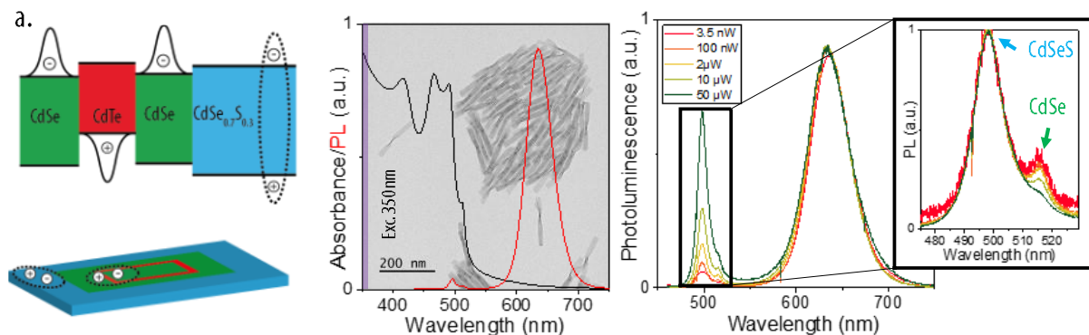
Figure 40: Tricolor emitting NPLs. a. Sketch and band alignment of the CdSe-CdTe-CdSe-CdSe x S 1-x heterostructure. b. Absorption (black) and PL (red) spectra of the CdSe-CdTe-CdSe-CdSe x S 1-x heterostructure. In the back font is introduced a corresponding TEM picture. The excitation has been conducted at 350 nm. c. PL spectra according to the incoming excitation fluence. The panel corresponds to a zoom on the 500 nm region. For clarity, the PL spectra have been normalized to the red emission. The excitation has been conducted at 400 nm.
