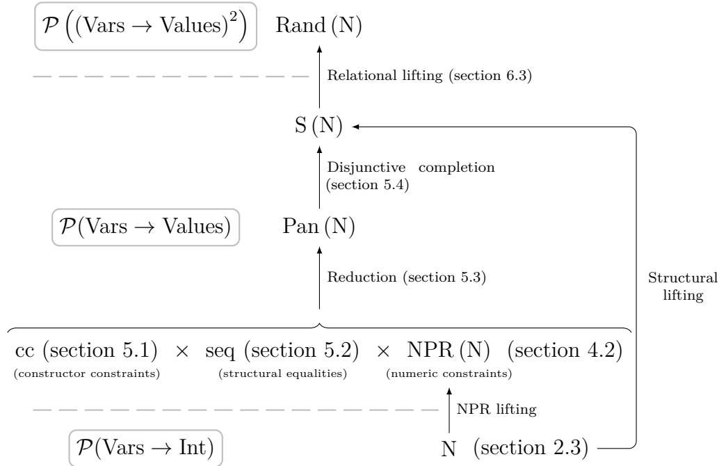
Figure 4.1: The construction of the RAND abstract domain. The frame-enclosed sets are the sets the abstract domains concretize to.
