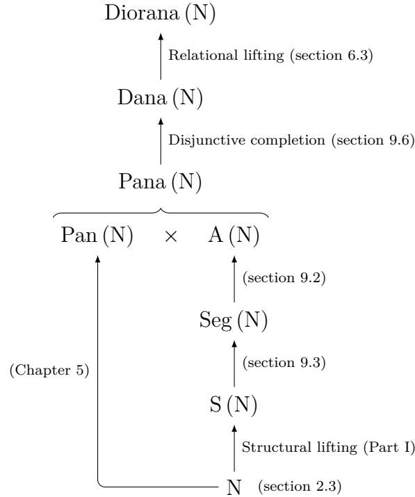
Figure 9.2: The construction of the abstract domain for analyzing programs that manipulate both values from algebraic types, and arrays containing values from algebraic types.
