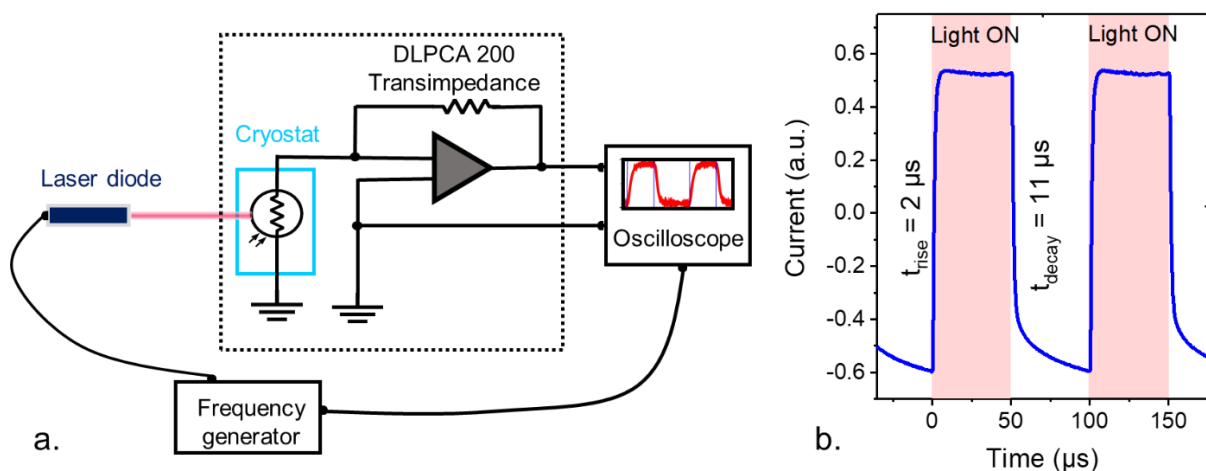
Figure 2.17: Device time response measurement. a. Experimental setup for response time measurement with a laser diode. b. Current as a function of time under illumination of 2.5 \mu m
