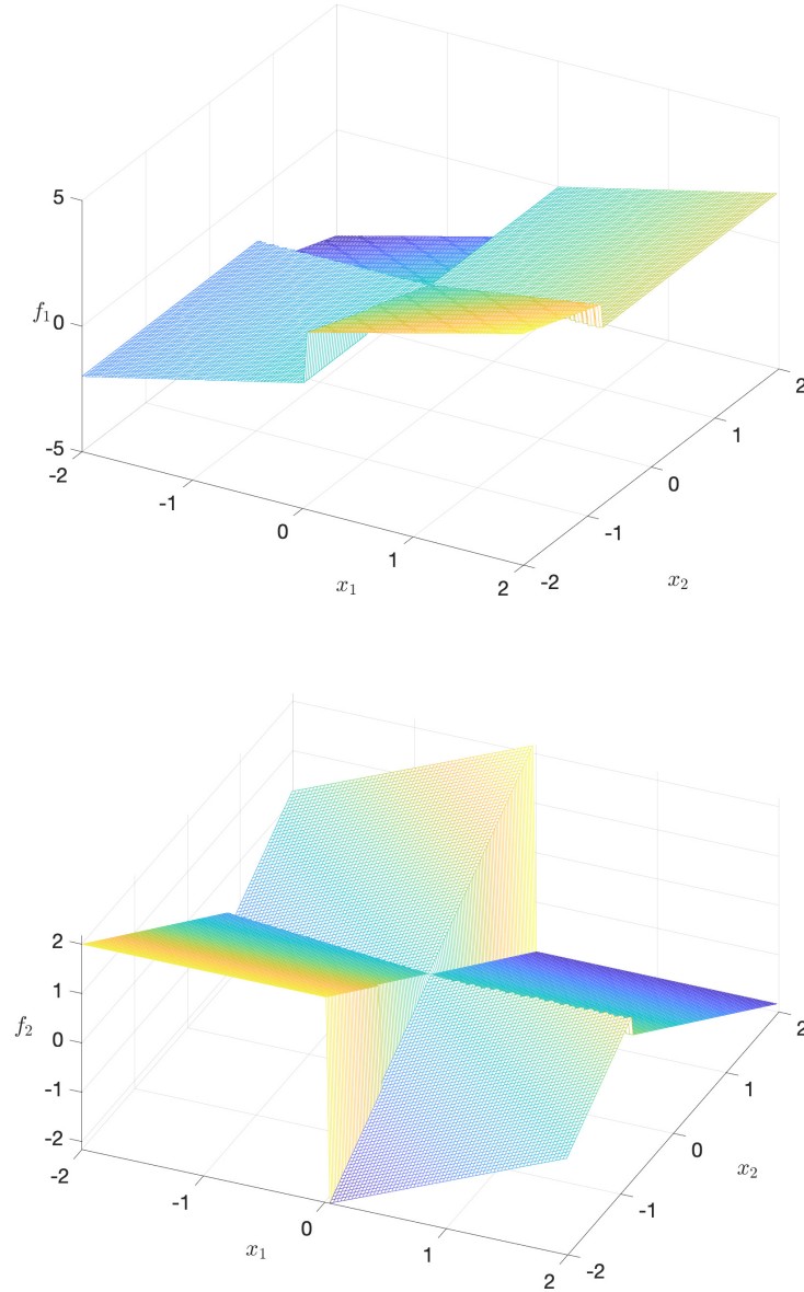
Figure P.13: Plots of the two components of f(x) = A_n x + A_p R^{-1} H_1 \phi(u) in (4.53) with the data in (4.54) (plots were obtained with the PWA description, without the use of explicit representation).
