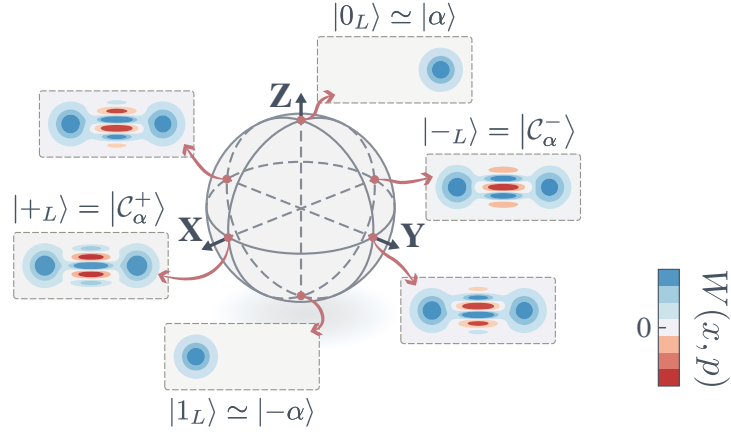
Figure 1.4: Encoding a cat qubit in a quantum harmonic oscillator. Computational states on the Z axis of the Bloch sphere are approximately coherent states delocalized on either side of phase space, hence providing an exponentially small probability of bit-flip errors.
