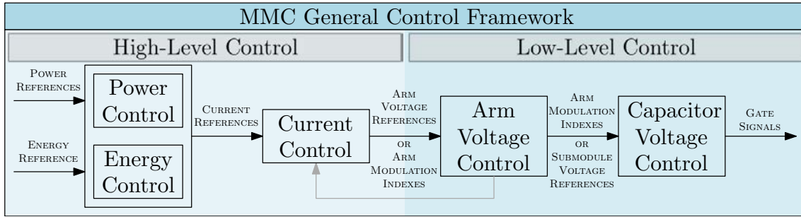
Figure 1.9: Modular multilevel converter general control framework.
