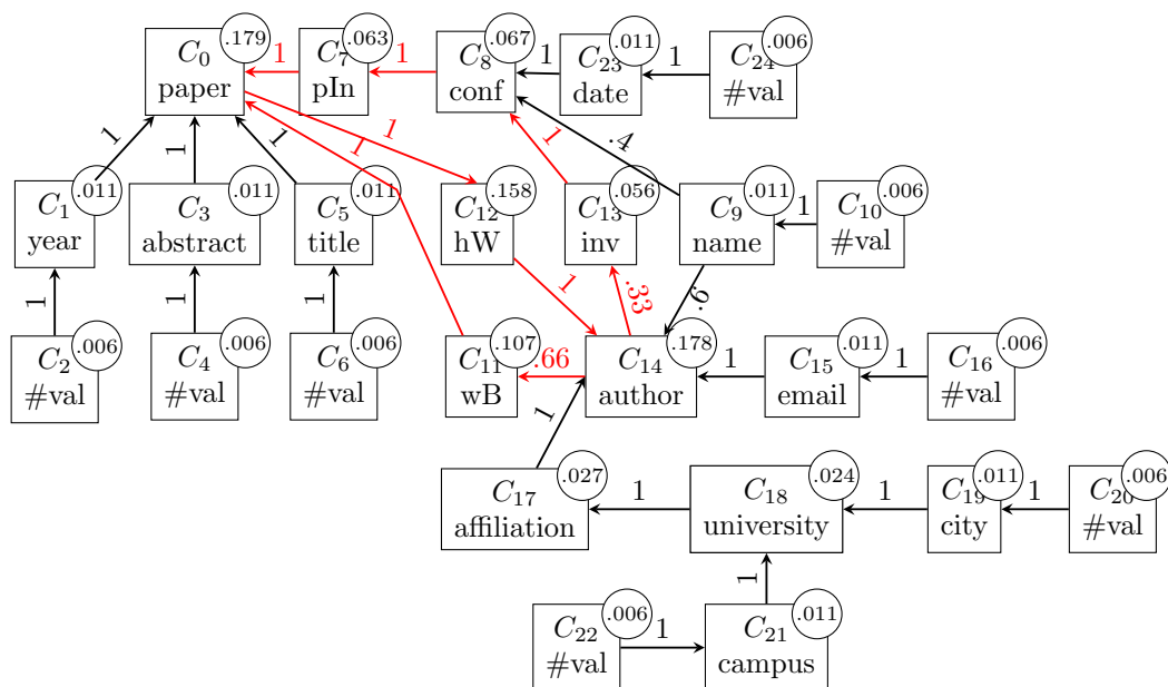
Figure 6.6: The w_{dw-PR} propagation on \mathcal{G}_R , the reversed collection graph.
