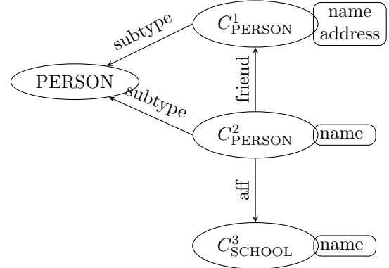
Figure 3.17: The Property Graph schema inferred from Figure 3.16.
