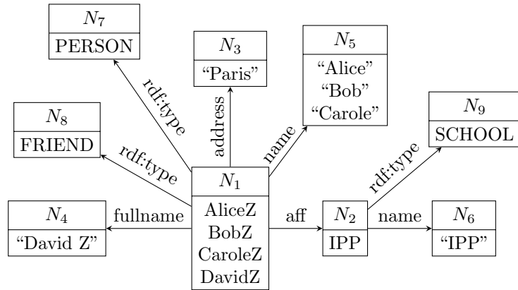
Figure 3.11: The type-then-data (weak and strong) quotient summary with type generalization.
