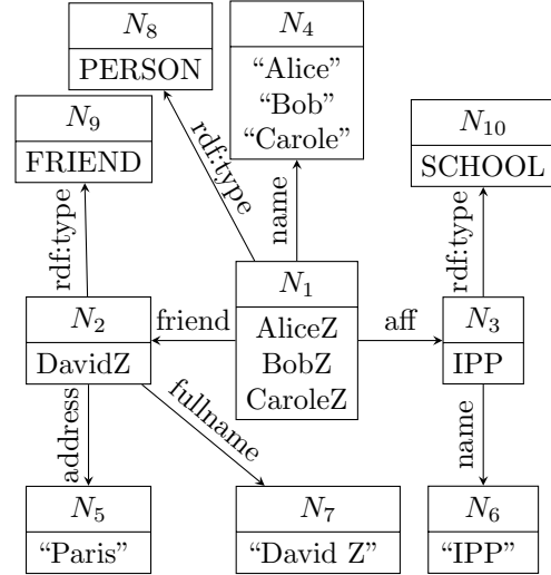
Figure 3.10: Data-then-type strong summary.
