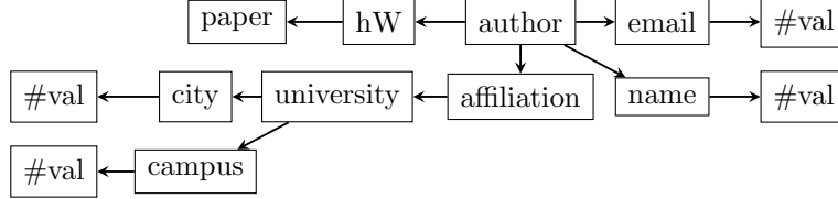
Figure 6.8: The bound_{DAG} boundary obtained for the main entity author , based on w_{DAG} scores.
