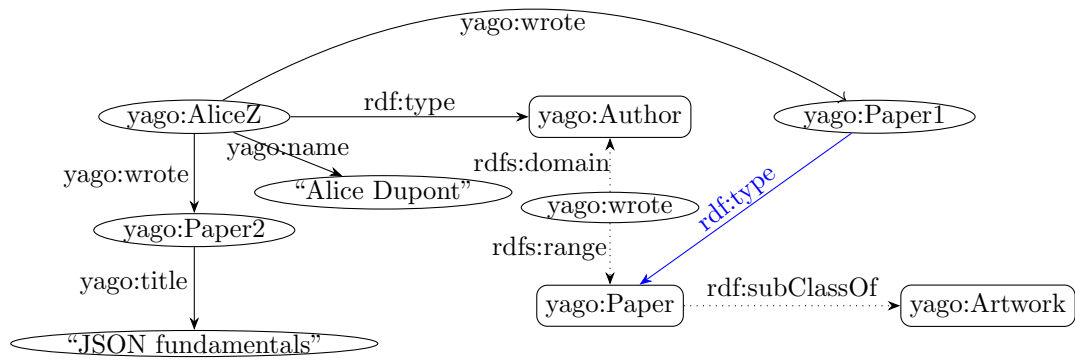
Figure 2.7: The RDF graph corresponding to the RDF triples in Figure 2.6. The graph also contains those inferred by the graph saturation.
