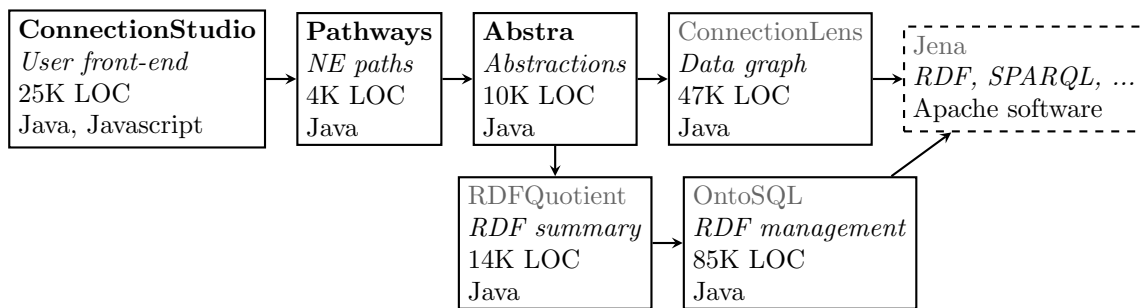
Figure 1.1: The software pile: from existing contributions (ONTOSQL, RDFQUOTIENT, CONNECTIONLENS) to the original ones (ABSTRA, PATHWAYS, CONNECTIONSTUDIO) proposed in the thesis.
