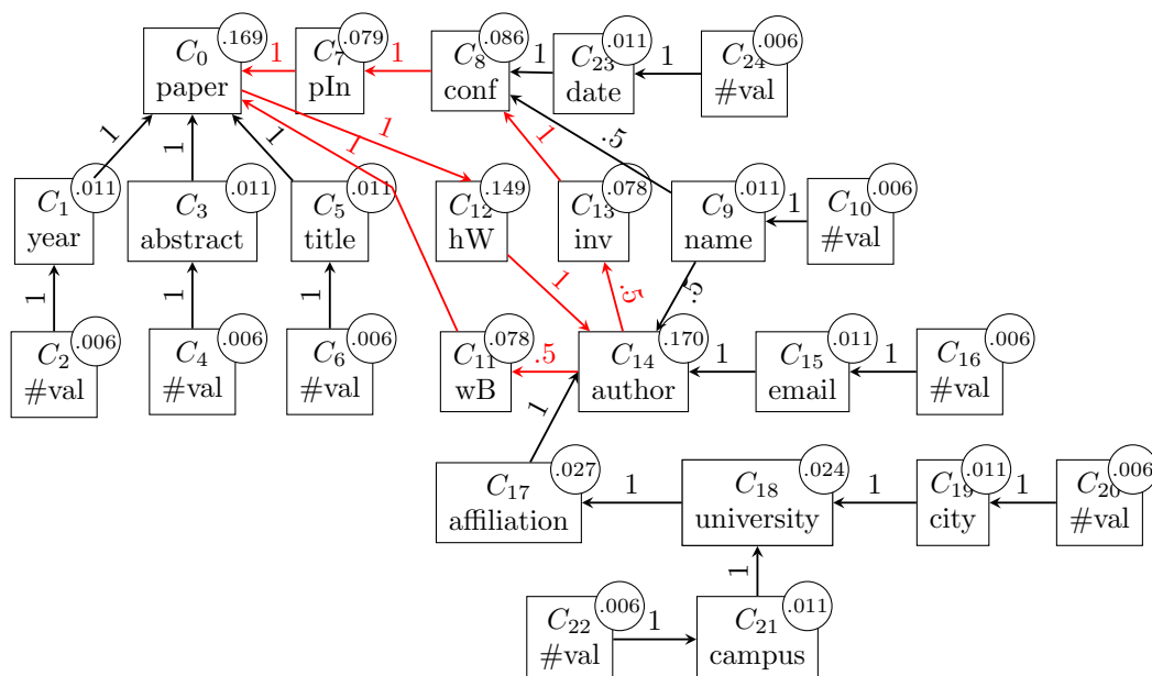
Figure 6.5: The w_{PR} propagation on \mathcal{G}_R , the reversed collection graph.
