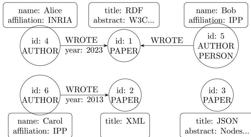
Figure 2.8: Property graph modelling scientific publications and their authors.
