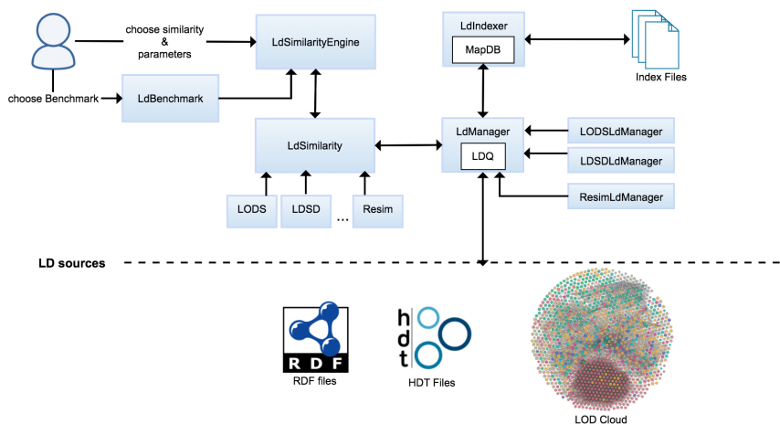
Figure 4.1: Overview of the Architecture of LDS .
