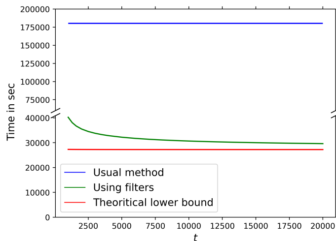
Figure 4.1. – Time (sec) to generate a clean RT according to t ( N = 2^{42} , r = 20 )
