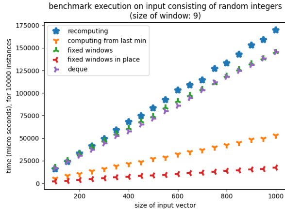
Figure 4.6: Comparison of five approaches for computing sliding window minimum. The input vector is composed of random integers. The size of the window is set to 9 and for each size of the input vector, 10000 instances were tested.
