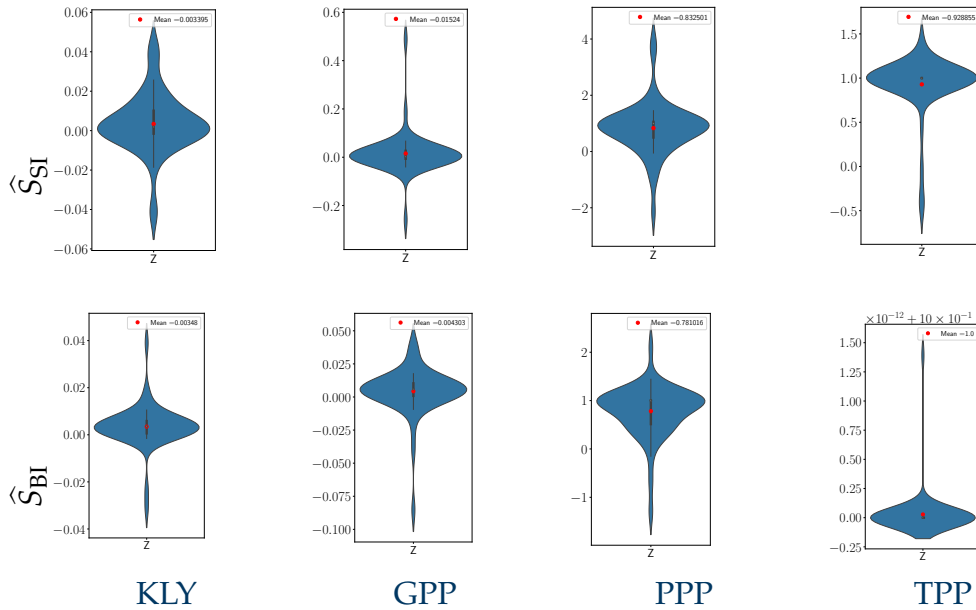
Figure 3.10 – Violin plots of Z across 50 samples from the KLY , GPP , PPP , and TPP using \widehat{S}_{\text{SI}} (first line) and \widehat{S}_{\text{BI}} (last line). Plots obtained using the toolbox structure_factor .
