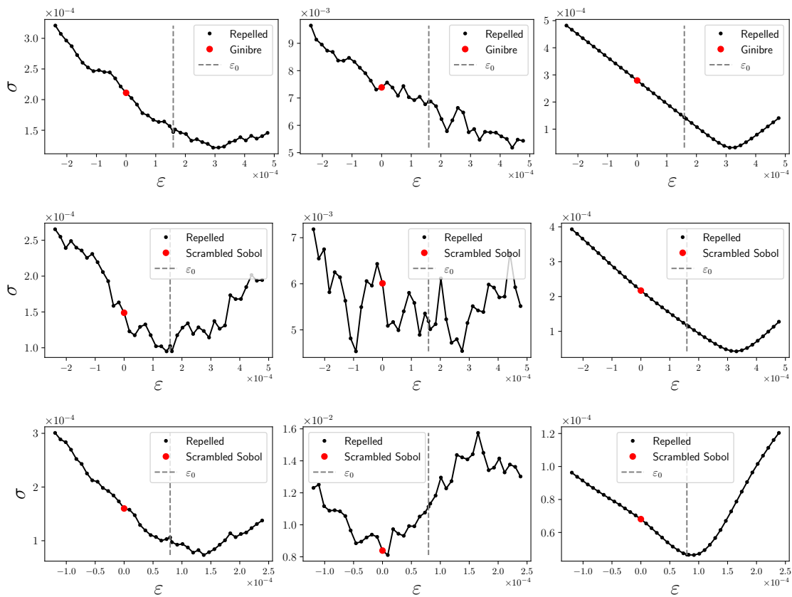
Figure 4.10 – Estimated standard deviations of \widehat{I}_{s,\Pi_\varepsilon\mathcal{G}\cap K} (Ginibre) and \widehat{I}_{s,\Pi_\varepsilon\mathcal{S}\cap K} (scrambled Sobol) with respect to \varepsilon for f_1 (first column), f_2 (second column), and f_3 (last column). The first row shows the obtained results for the GPP in d = 2 , the second row for the SSS in d = 2 , and the last one for the SSS in d = 3 . Plots obtained using the toolbox MCRPPy .
