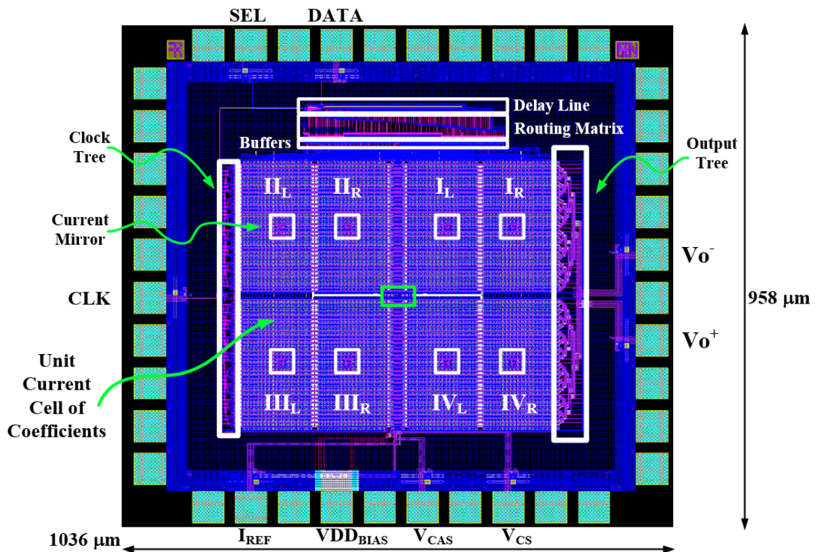
Figure 6.7: FIKRDAC Layout
