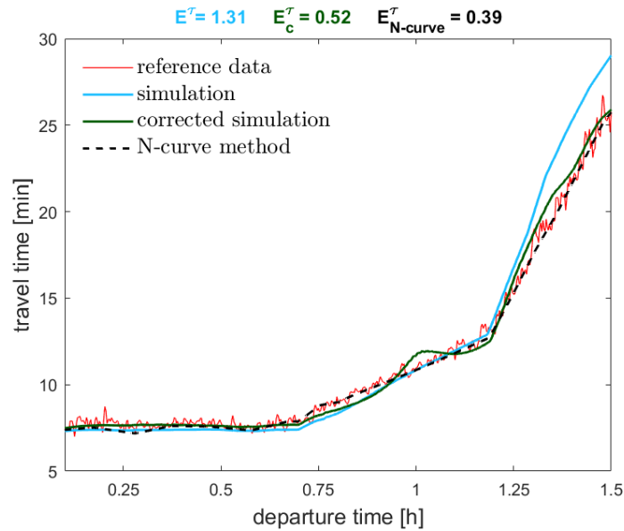
Figure 6.12: SUMO-1B . 1^{st} – Godu – \rho , L^2 approach. E_{GP}^\tau = 0.53 , E_{\text{baseline}}^\tau = 0.67 . Travel time estimation results.
